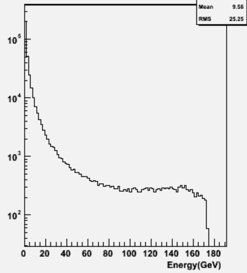
Start point R : w103902 ae1_e1e2e2ss_o
