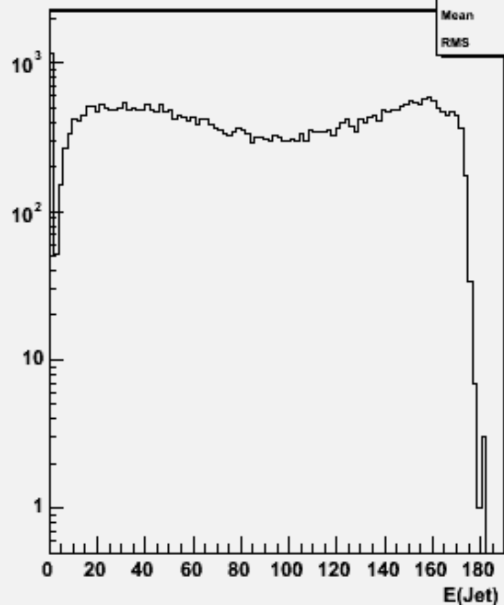
Jet energies(All jets)w103902 ae1_e1e2e2ss_o
