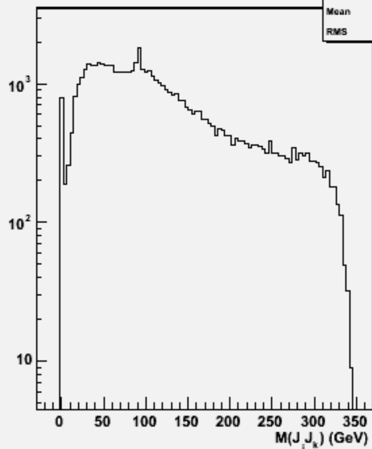
2jets mass(All comb)w103902 ae1_e1e2e2ss_o
