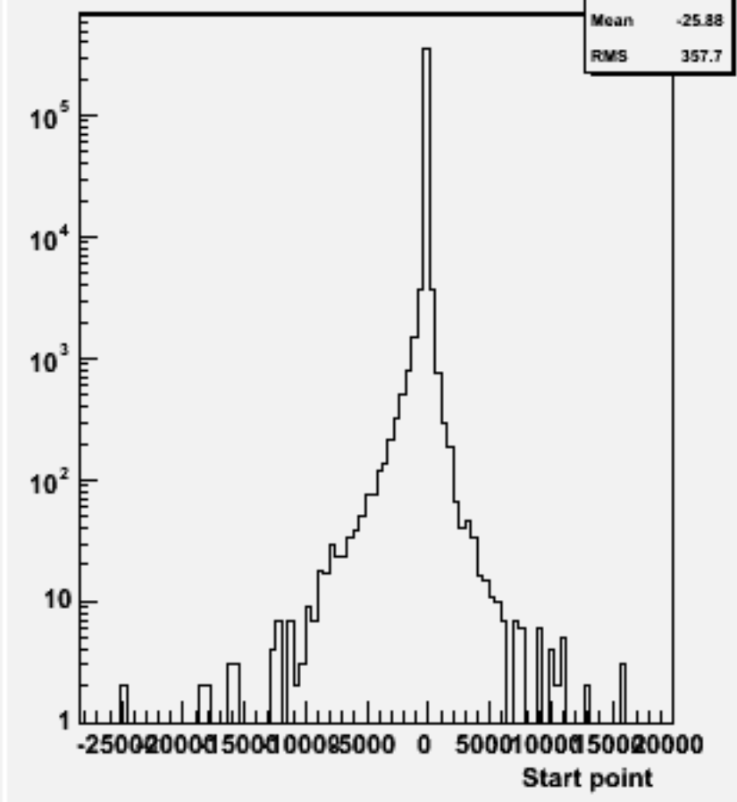
Start point Z : w103902 ae1_e1e2e2ss_o
