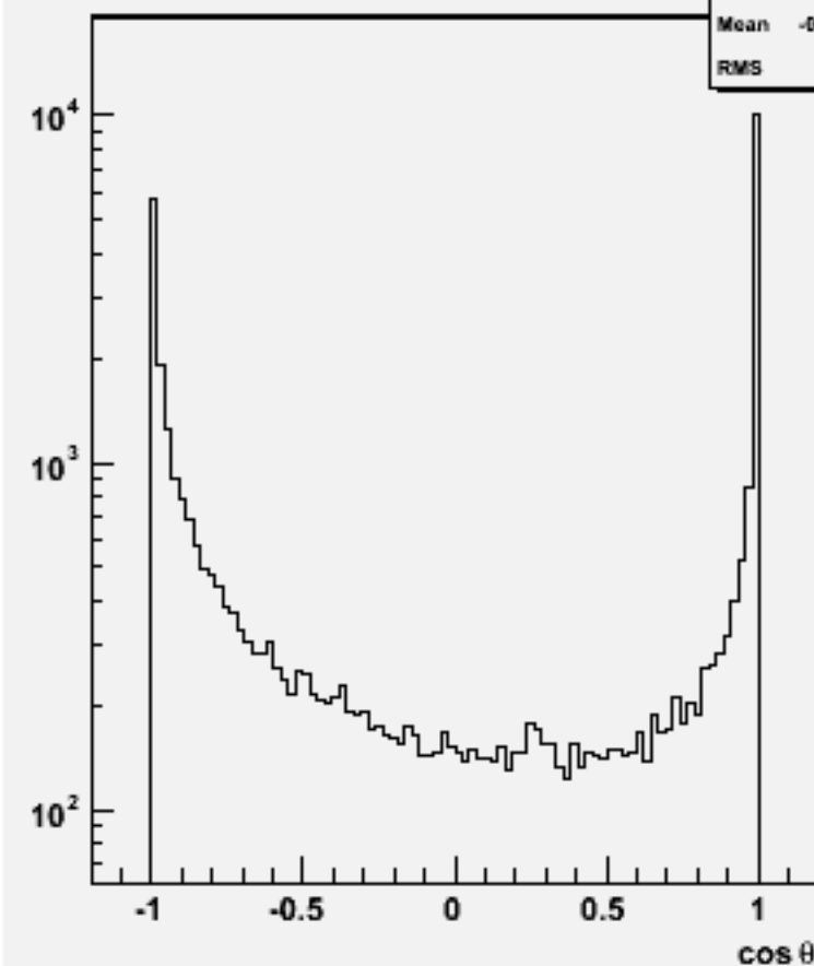
Jet cos \theta (All jets)w103902 ae1_e1e2e2ss_o
