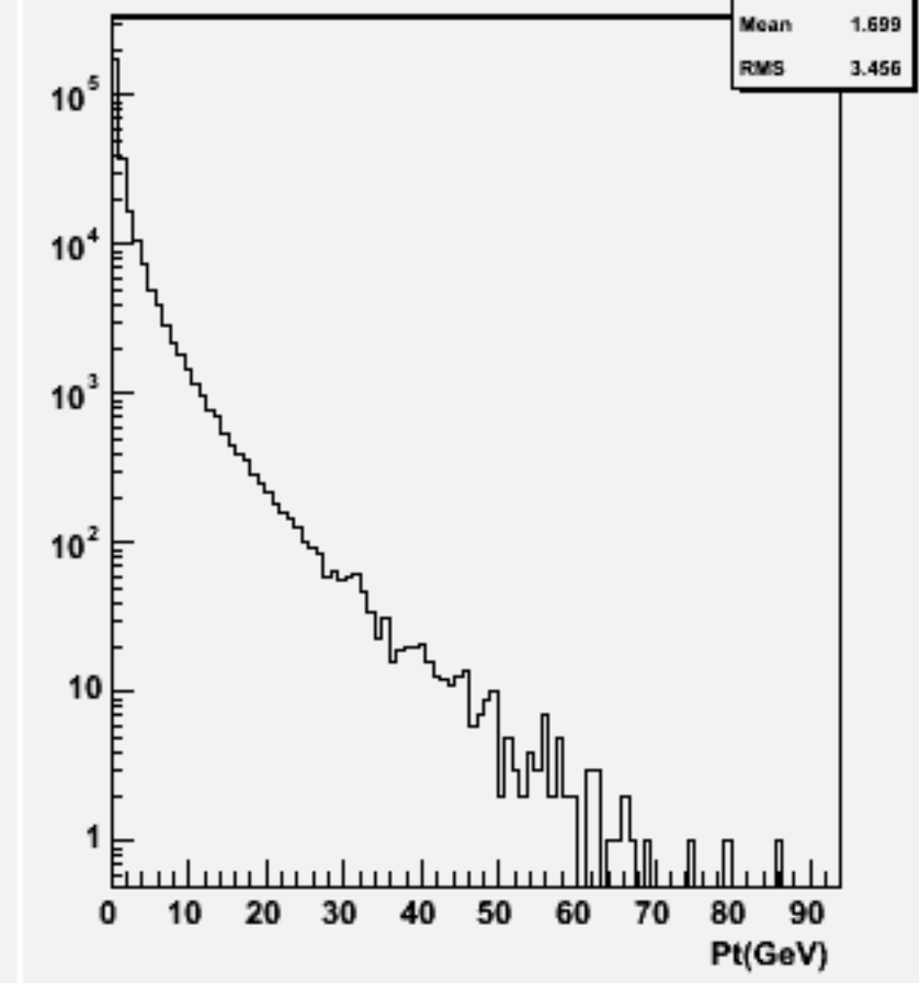
Start point Z : w103901 ae1_e1e2e2ss_o
