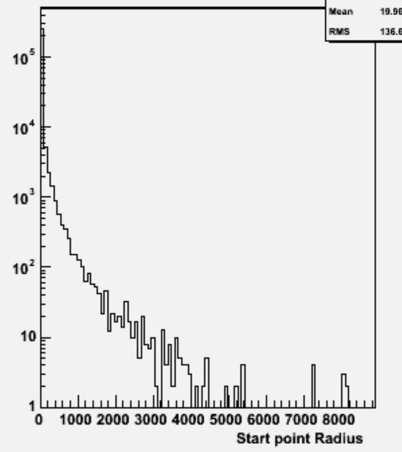
Start point R : w103901 ae1_e1e2e2ss_o
