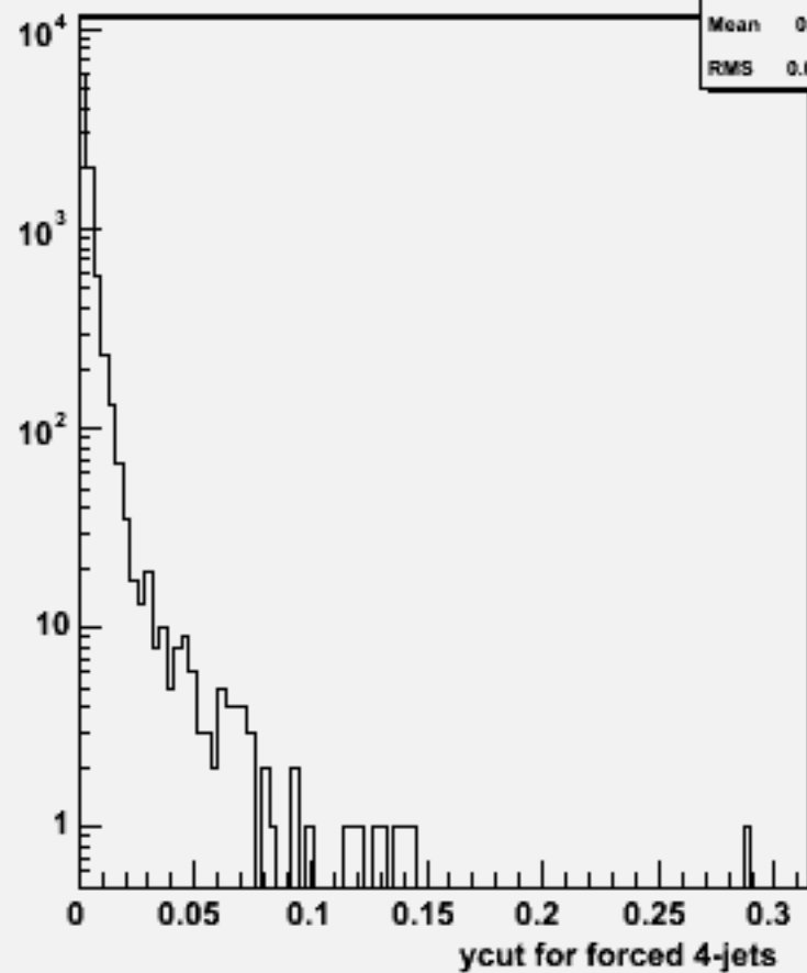
Ycut for 4-jets :w103901 ae1_e1e2e2ss_o
