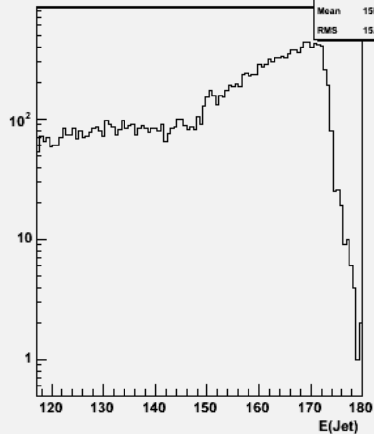
Jet energies(All jets)w103901 ae1_e1e2e2ss_o
