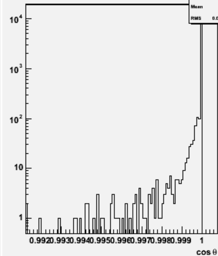
Jet cos \theta (All jets)w103901 ae1_e1e2e2ss_o
