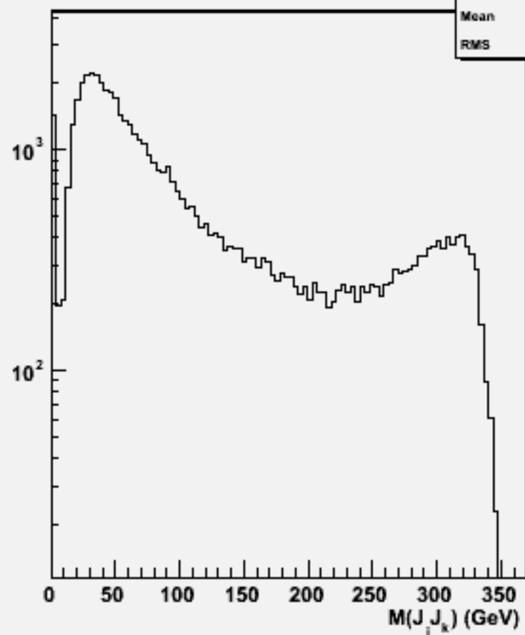
2jets mass(All comb)w103901 ae1_e1e2e2ss_o
