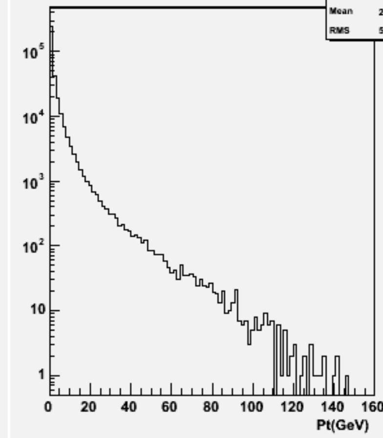
Start point Z : w103900 ae1_e1e2e2ss_o
