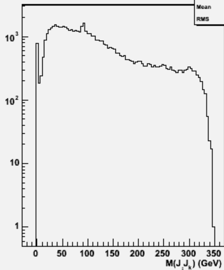
2jets mass(All comb)w103900 ae1_e1e2e2ss_o
