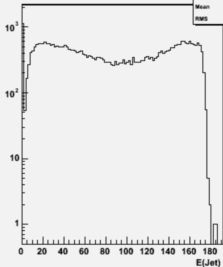
Jet energies(All jets)w103900 ae1_e1e2e2ss_o
