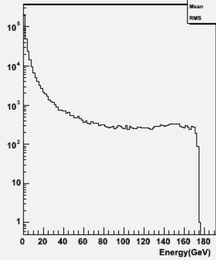
Start point R : w103900 ae1_e1e2e2ss_o
