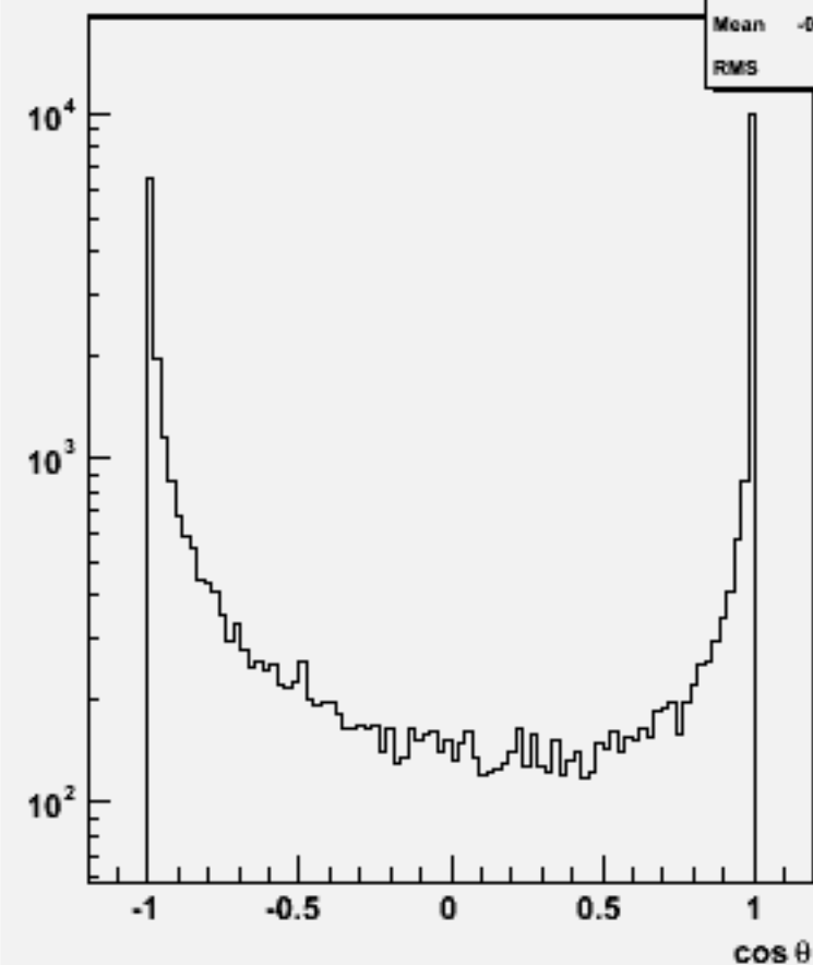
Jet cos \theta (All jets)w103900 ae1_e1e2e2ss_o
