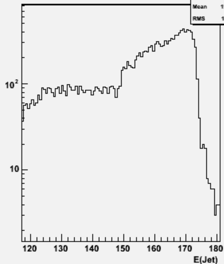
Jet energies(All jets)w103899 ae1_e1e2e2dd_o
