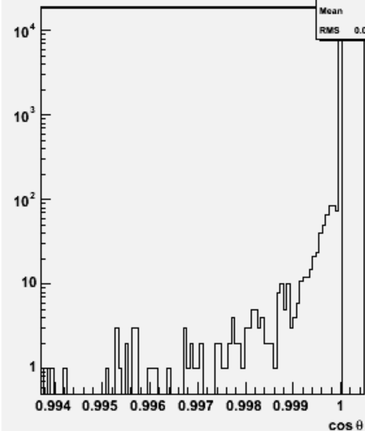
Jet cos \theta (All jets)w103899 ae1_e1e2e2dd_o
