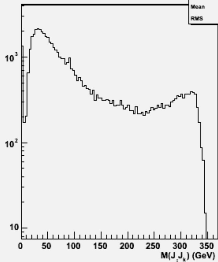
2jets mass(All comb)w103899 ae1_e1e2e2dd_o
