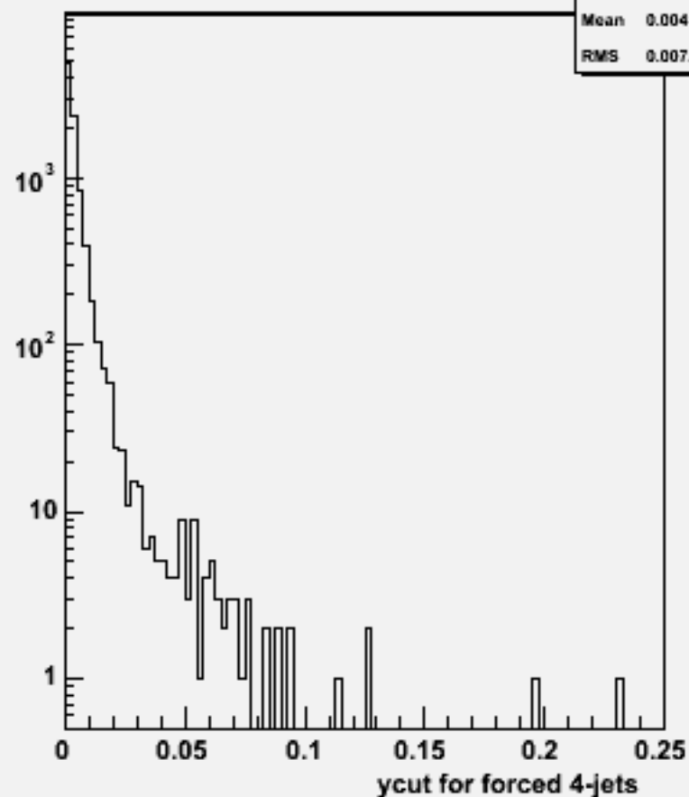
Ycut for 4-jets :w103899 ae1_e1e2e2dd_o
