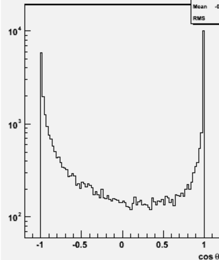
Jet cos \theta (All jets)w103898 ae1_e1e2e2dd_o
