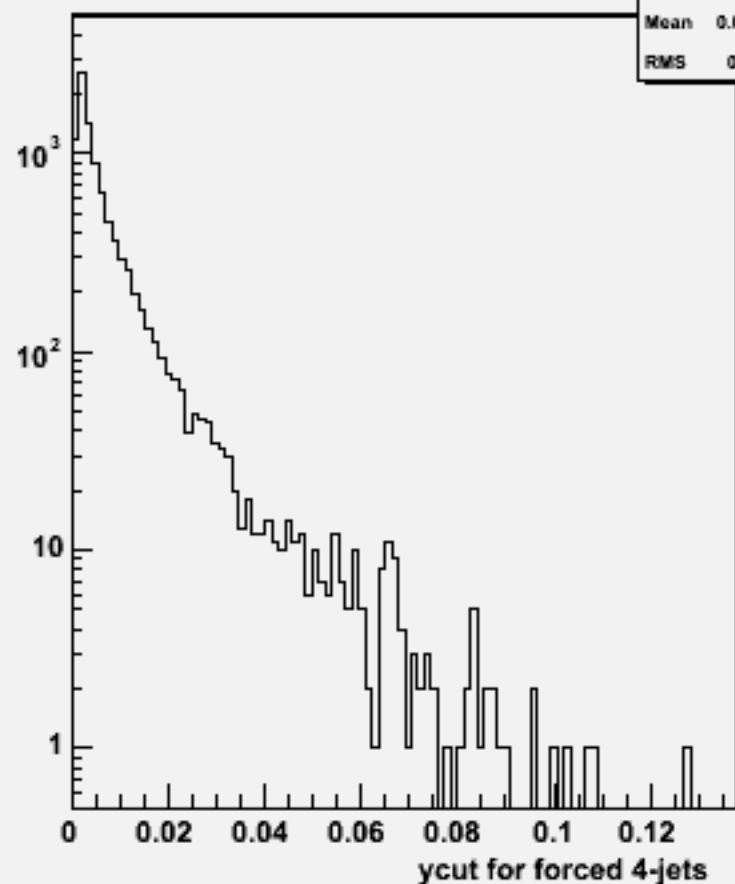
Ycut for 4-jets :w103898 ae1_e1e2e2dd_o
