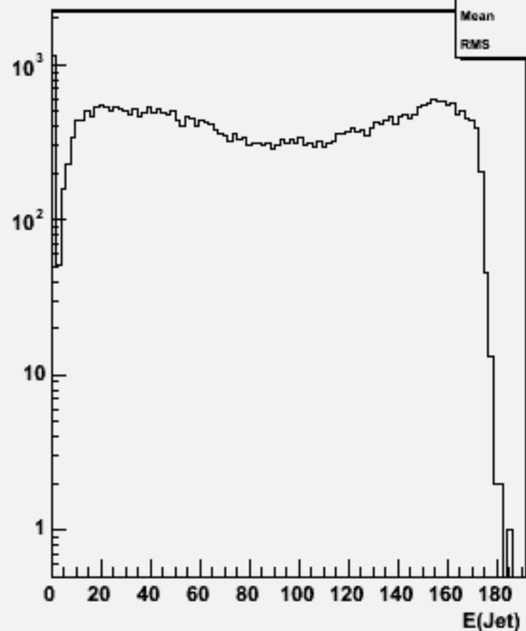
Jet energies(All jets)w103898 ae1_e1e2e2dd_o
