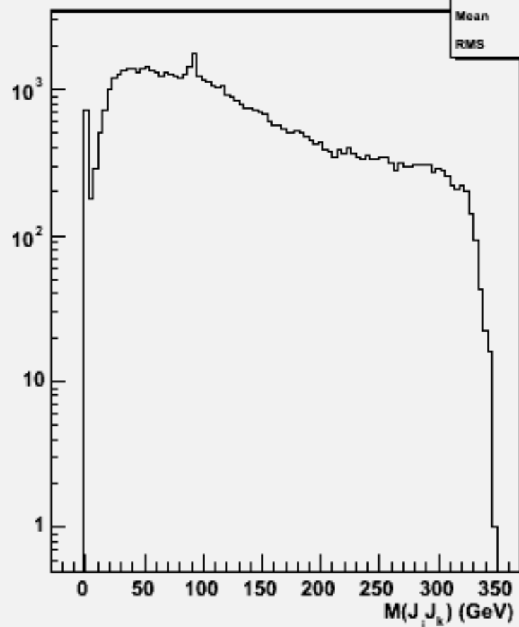
2jets mass(All comb)w103898 ae1_e1e2e2dd_o
