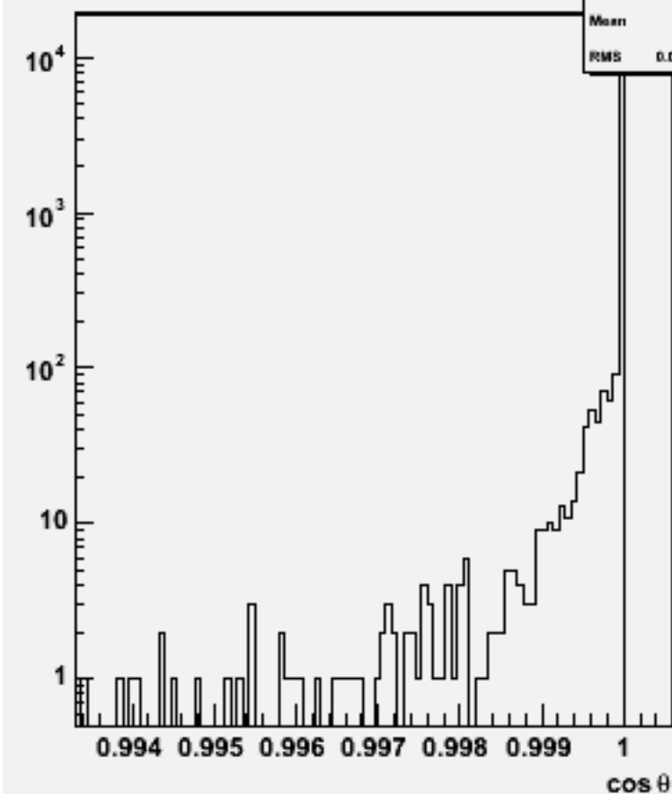
Jet cos \theta (All jets)w103897 ae1_e1e2e2dd_o
