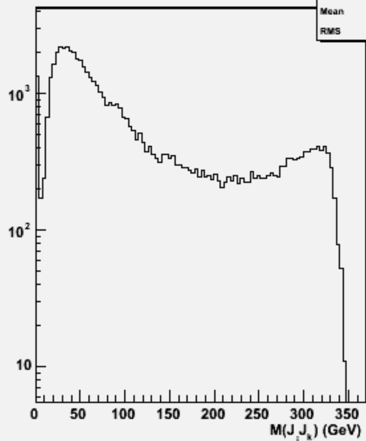
2jets mass(All comb)w103897 ae1_e1e2e2dd_o
