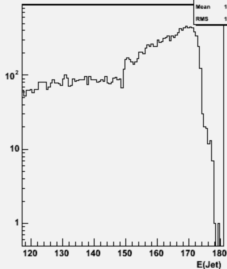
Jet energies(All jets)w103897 ae1_e1e2e2dd_o
