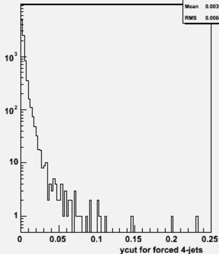
Ycut for 4-jets :w103897 ae1_e1e2e2dd_o
