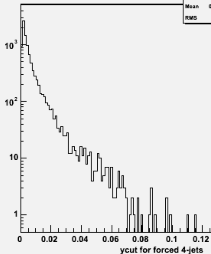
Ycut for 4-jets :w103896 ae1_e1e2e2dd_o
