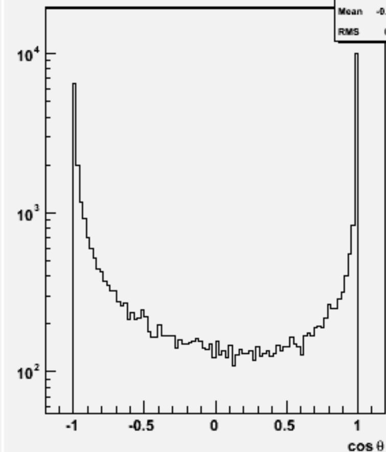
Jet cos \theta (All jets)w103896 ae1_e1e2e2dd_o
