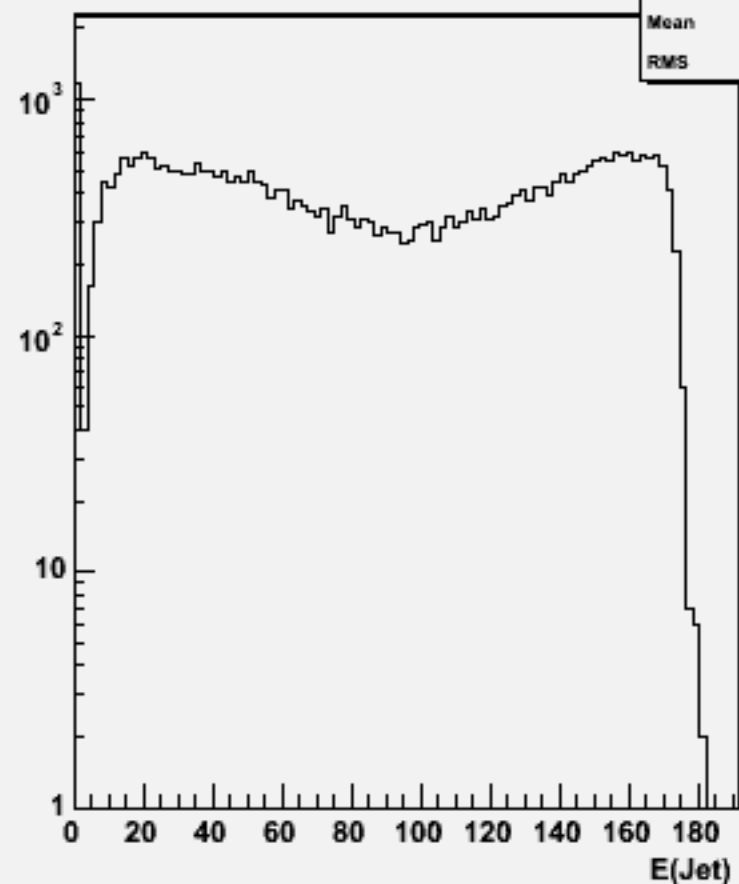
Jet energies(All jets)w103896 ae1_e1e2e2dd_o
