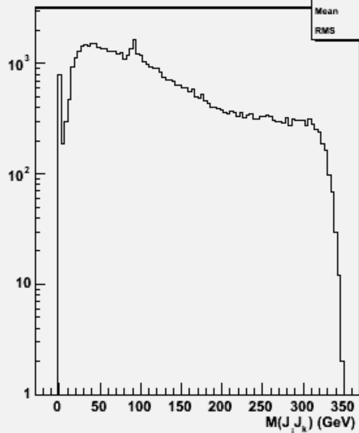
2jets mass(All comb)w103896 ae1_e1e2e2dd_o
