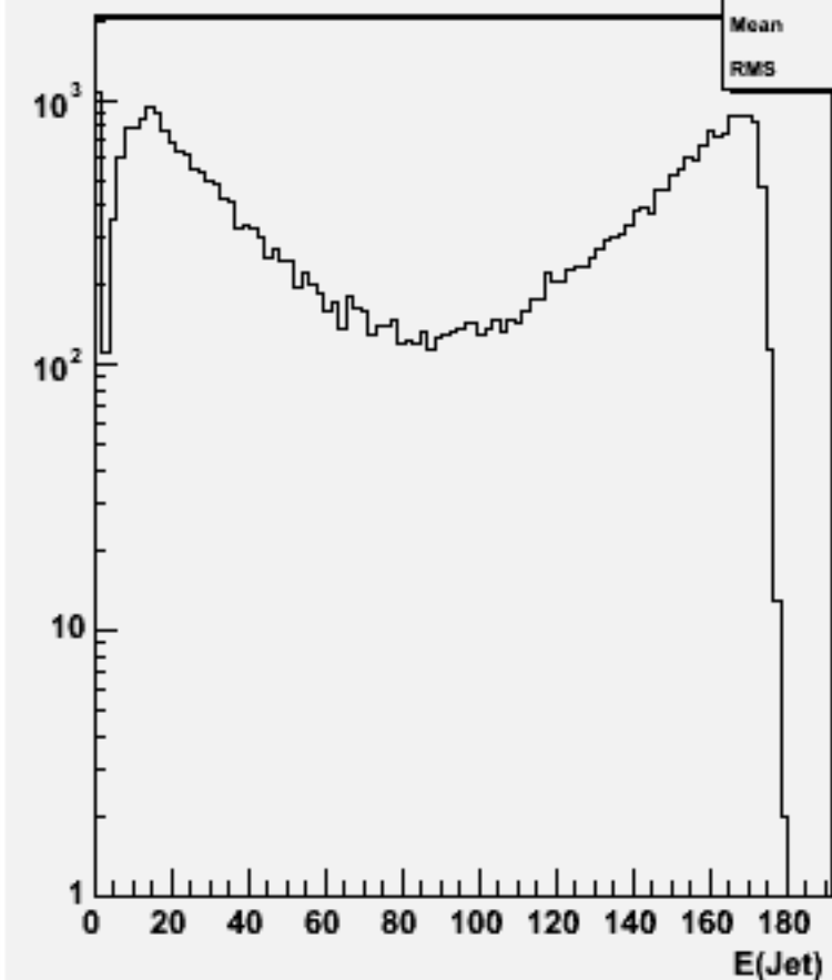
Jet energies(All jets)w103890 ae1_e1e2e2e2_o
