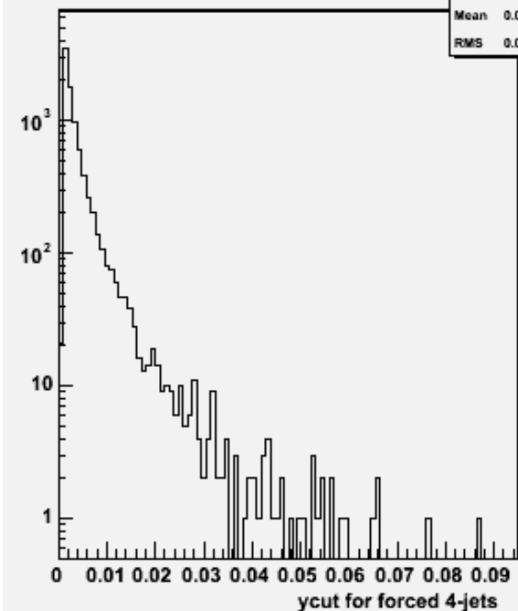
Ycut for 4-jets :w103890 ae1_e1e2e2e2_o
