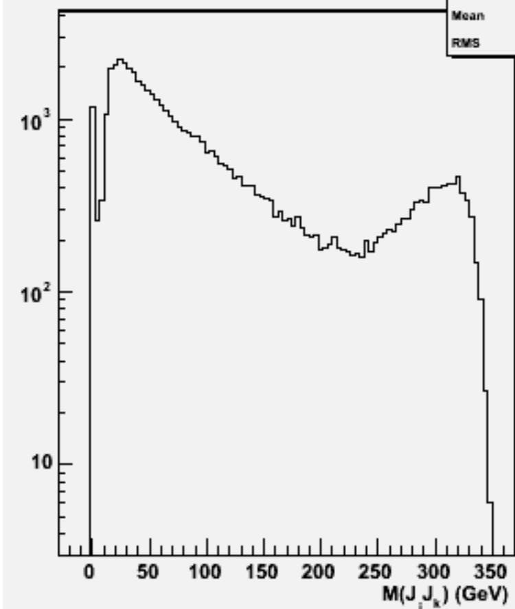
2jets mass(All comb)w103890 ae1_e1e2e2e2_o
