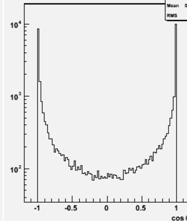
Jet cos \theta (All jets)w103890 ae1_e1e2e2e2_o
