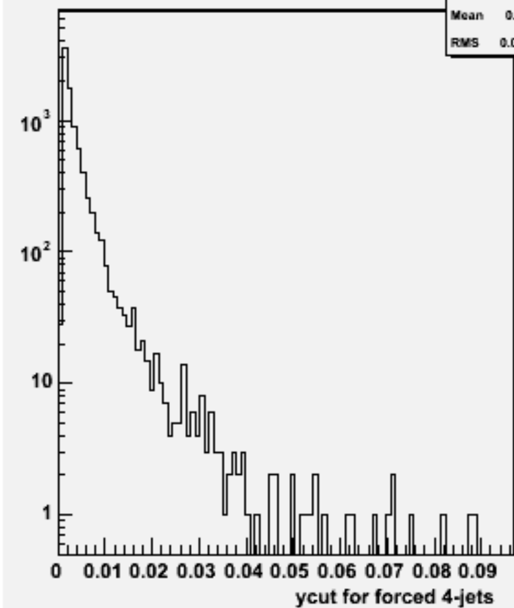
Ycut for 4-jets :w103888 ae1_e1e2e2e2_o
