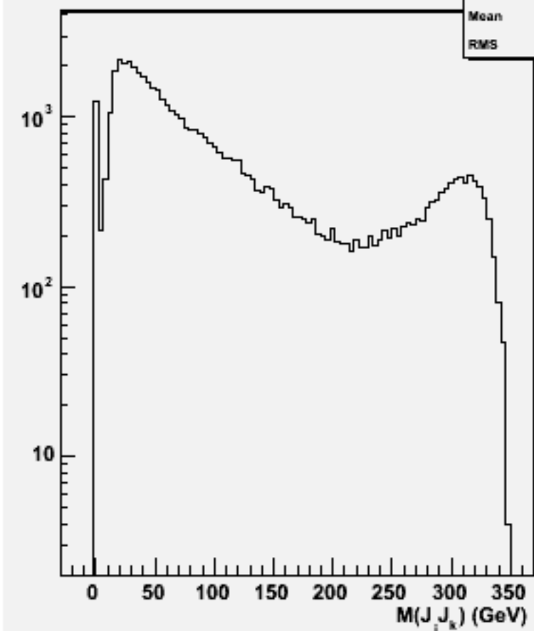
2jets mass(All comb)w103888 ae1_e1e2e2e2_o
