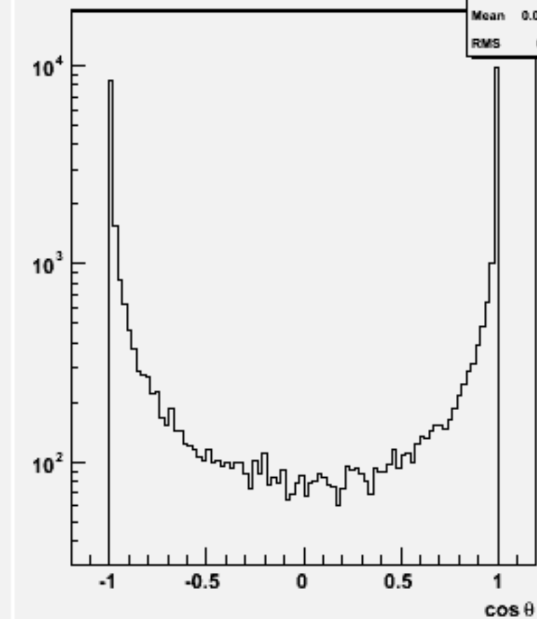
Jet cos \theta (All jets)w103888 ae1_e1e2e2e2_o
