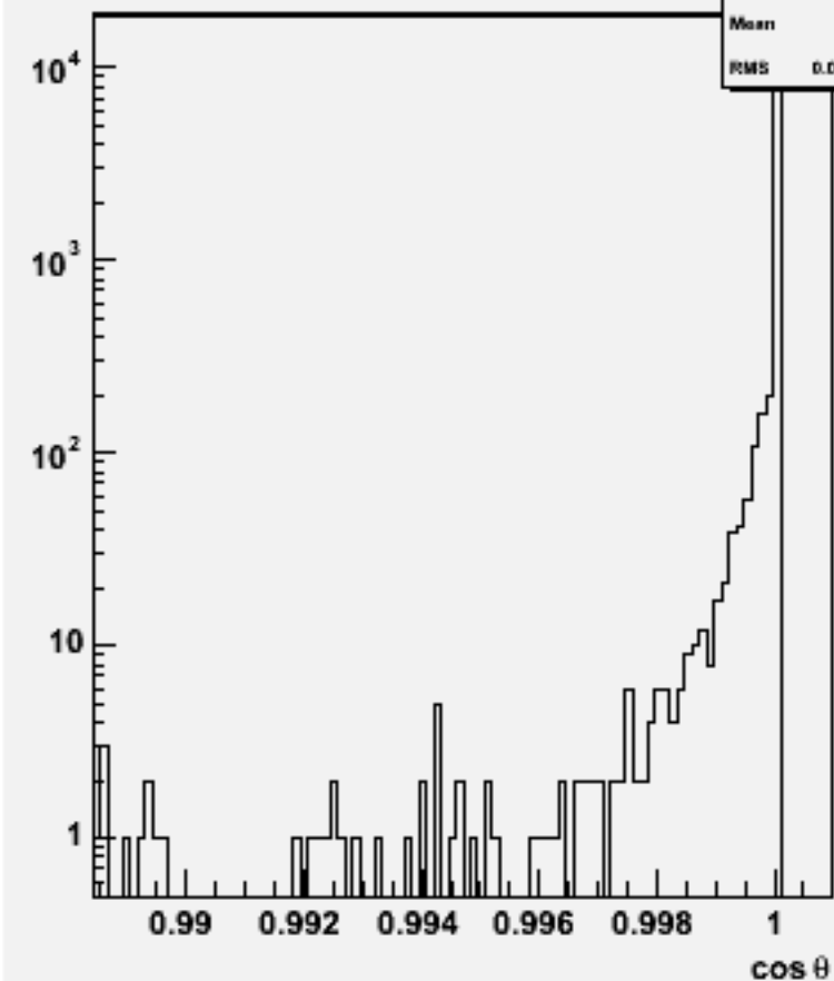
Jet cos \theta (All jets)w103885 ae1_e1e1e1bb_o
