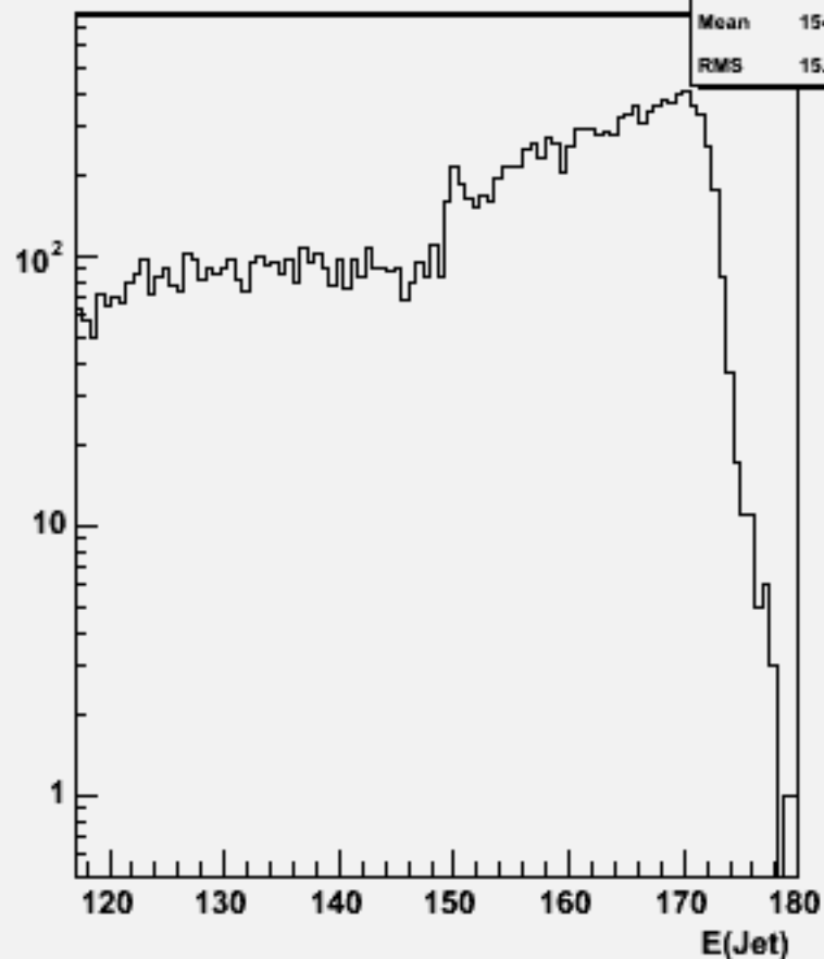
Jet energies(All jets)w103885 ae1_e1e1e1bb_o
