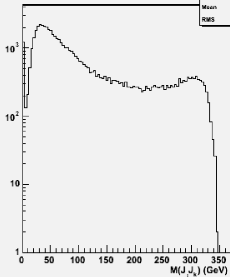
2jets mass(All comb)w103885 ae1_e1e1e1bb_o
