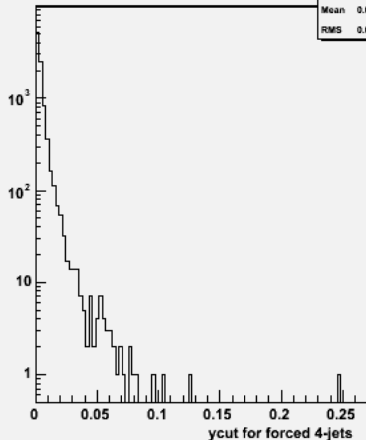
Ycut for 4-jets :w103885 ae1_e1e1e1bb_o
