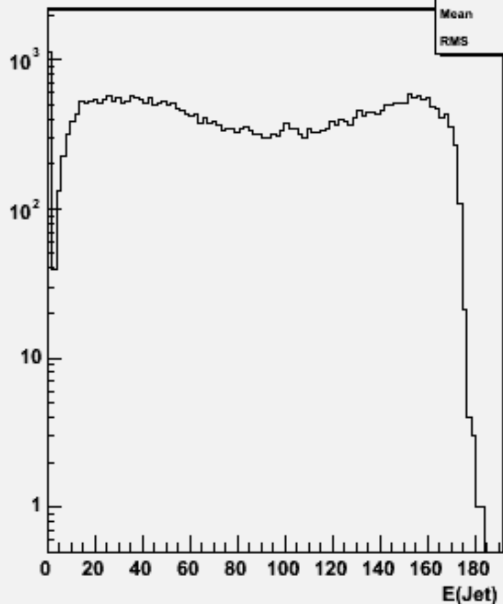
Jet energies(All jets)w103884 ae1_e1e1e1bb_o
