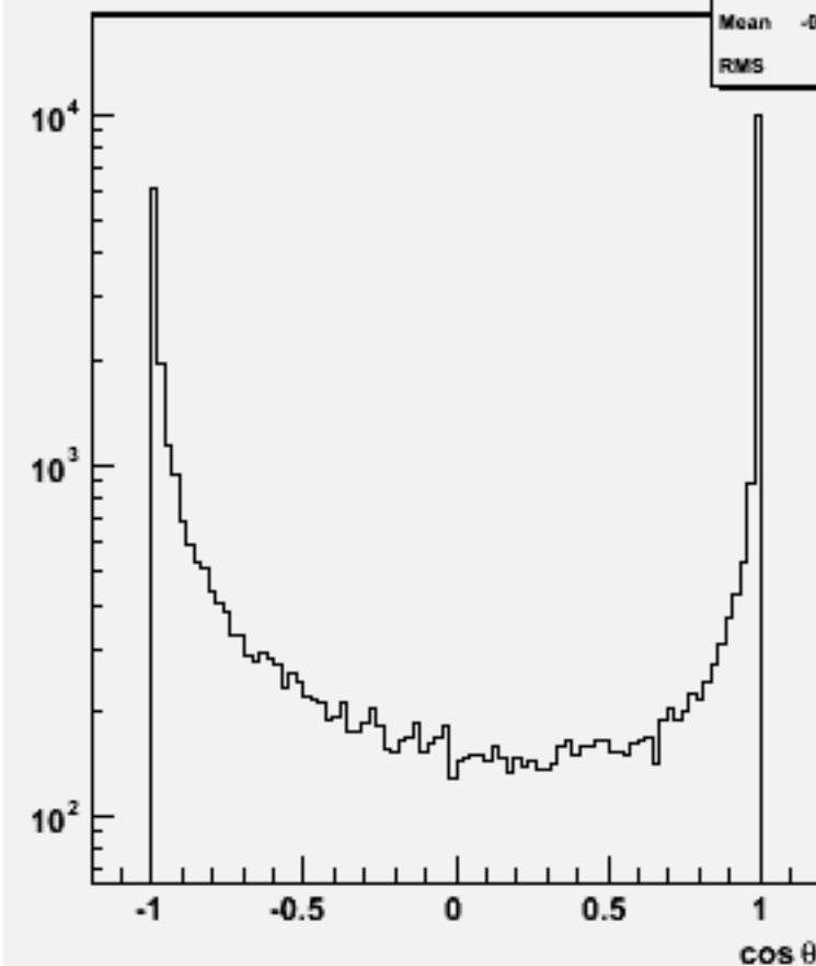
Jet cos \theta (All jets)w103884 ae1_e1e1e1bb_o
