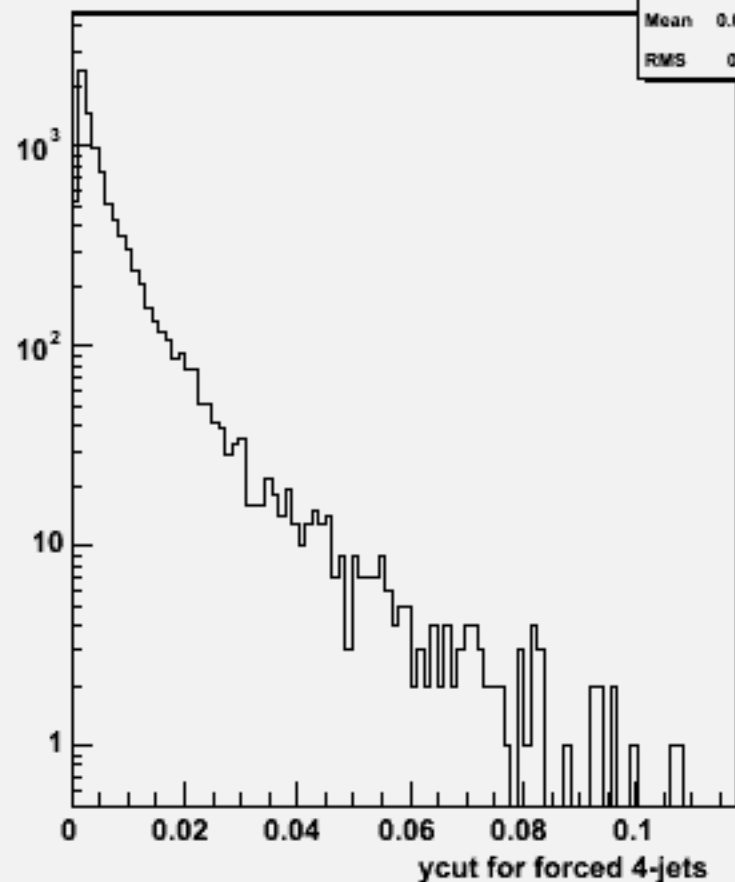
Ycut for 4-jets :w103884 ae1_e1e1e1bb_o
