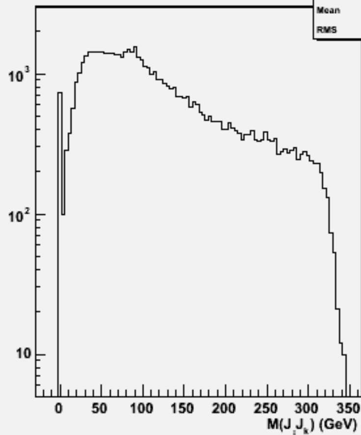
2jets mass(All comb)w103884 ae1_e1e1e1bb_o
