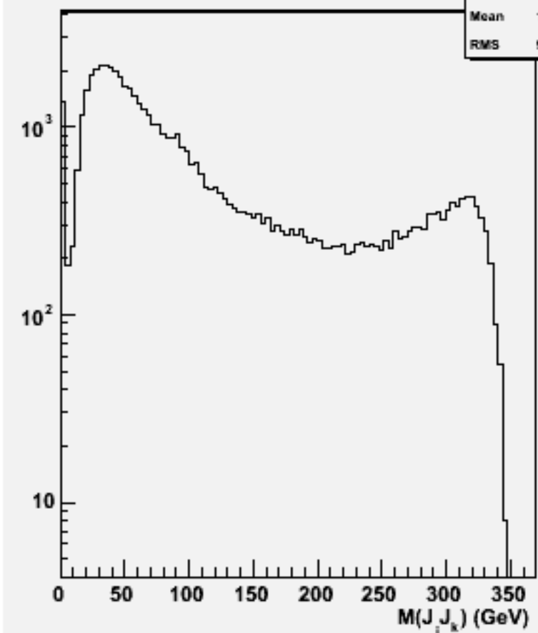
2jets mass(All comb)w103883 ae1_e1e1e1ss_o
