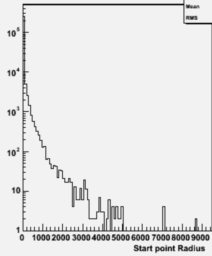
Start point R : w103883 ae1_e1e1e1ss_o
