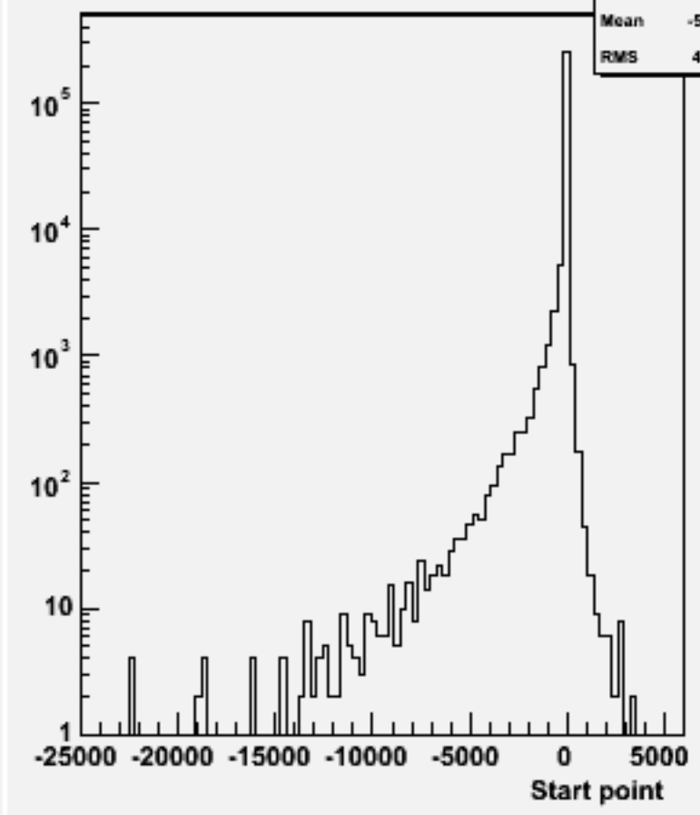
Start point Z : w103883 ae1_e1e1e1ss_o
