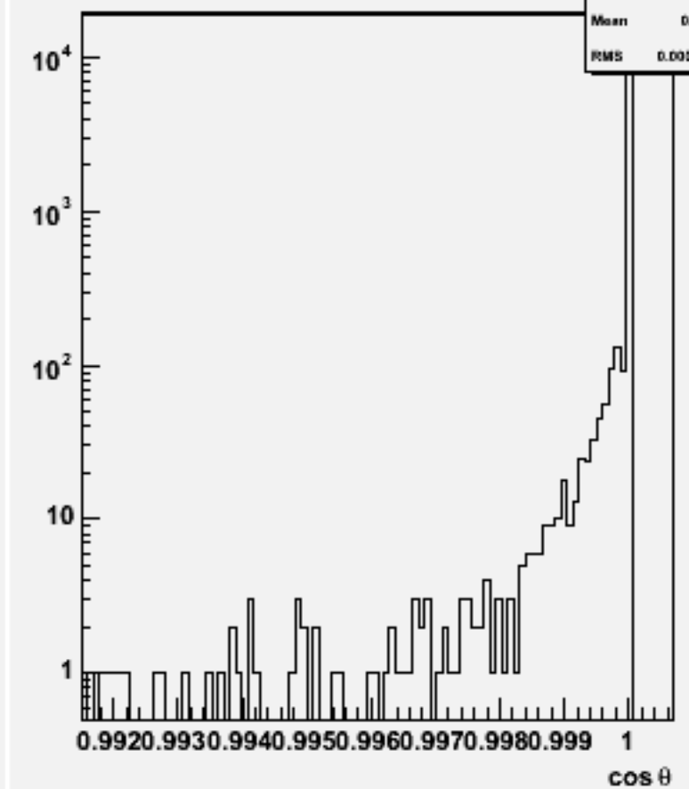
Jet cos \theta (All jets)w103883 ae1_e1e1e1ss_o
