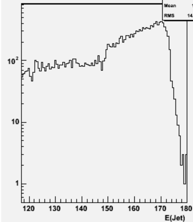
Jet energies(All jets)w103883 ae1_e1e1e1ss_o
