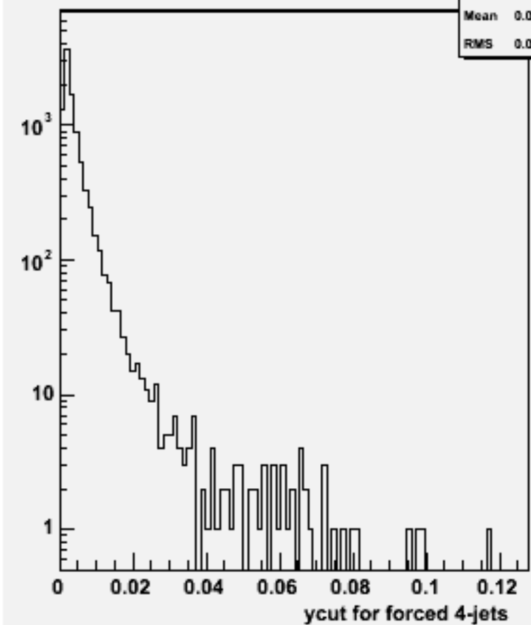
Ycut for 4-jets :w103883 ae1_e1e1e1ss_o
