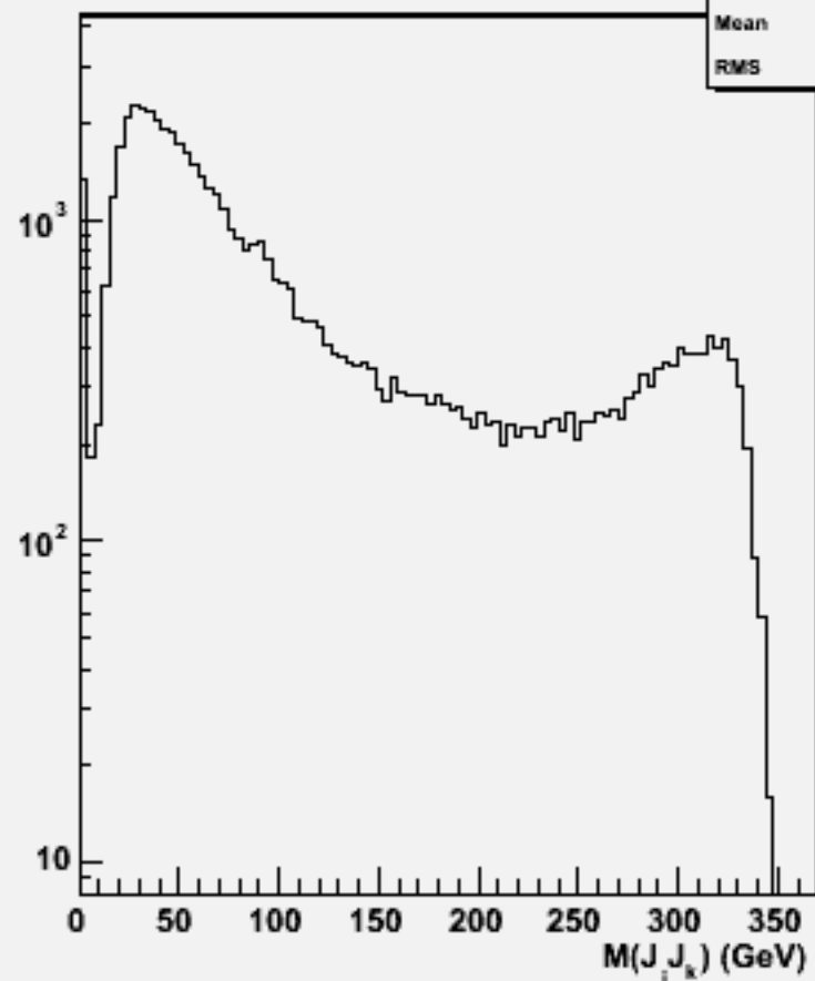
2jets mass(All comb)w103881 ae1_e1e1e1ss_o
