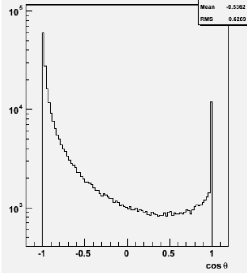
Particle cos \theta : w103881 ae1_e1e1e1ss_o
