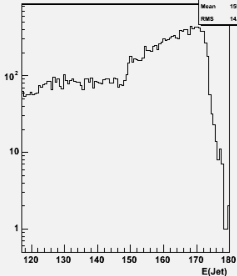
Jet energies(All jets)w103881 ae1_e1e1e1ss_o
