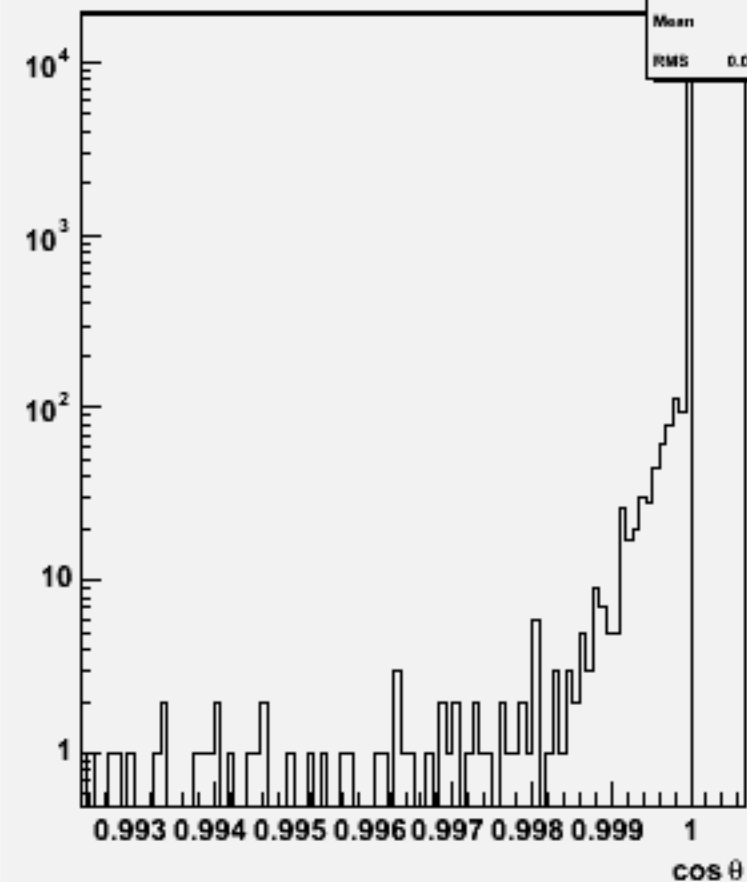
Jet cos \theta (All jets)w103881 ae1_e1e1e1ss_o
