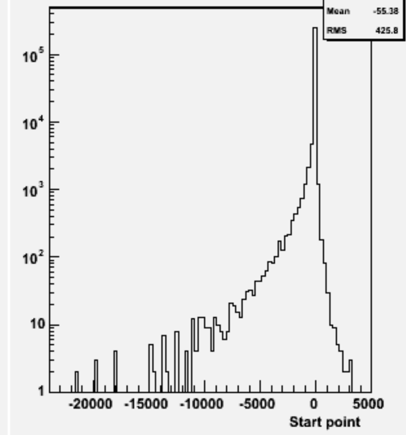
Start point Z : w103881 ae1_e1e1e1ss_o
