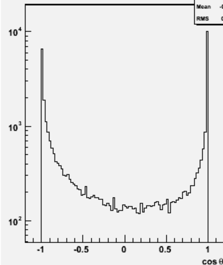
Jet cos \theta (All jets)w103880 ae1_e1e1e1ss_o
