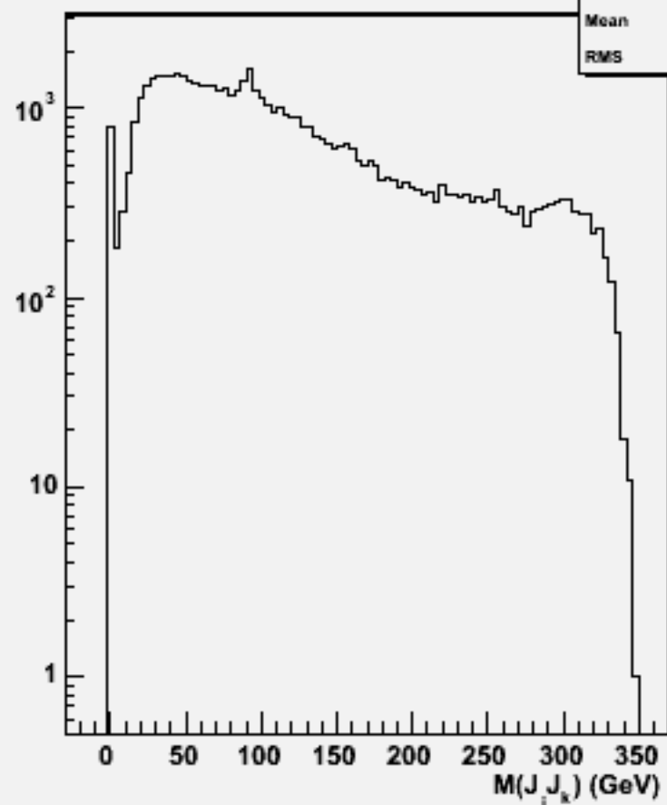
2jets mass(All comb)w103880 ae1_e1e1e1ss_o
