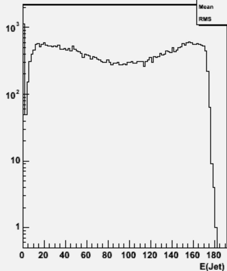
Jet energies(All jets)w103880 ae1_e1e1e1ss_o
