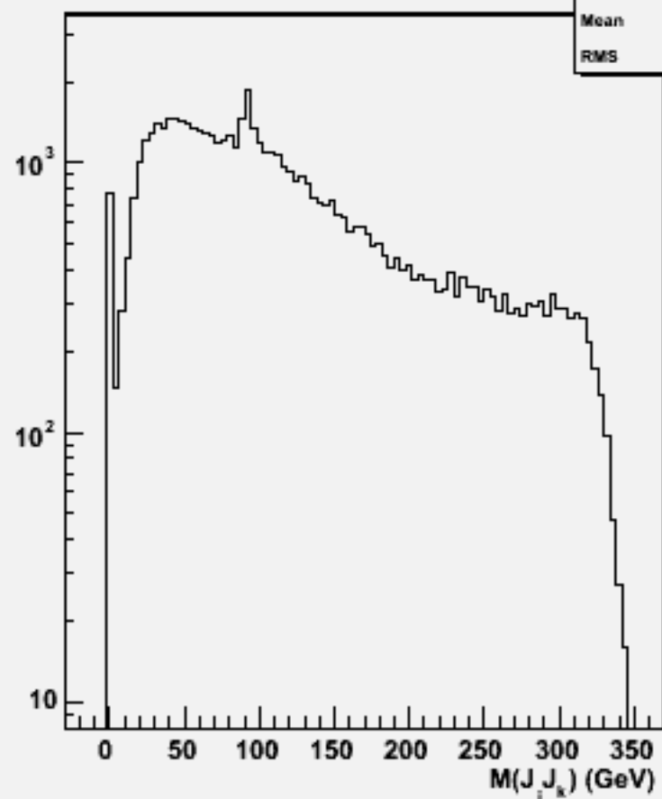
2jets mass(All comb)w103878 ae1_e1e1e1dd_o
