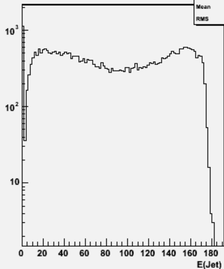
Jet energies(All jets)w103878 ae1_e1e1e1dd_o
