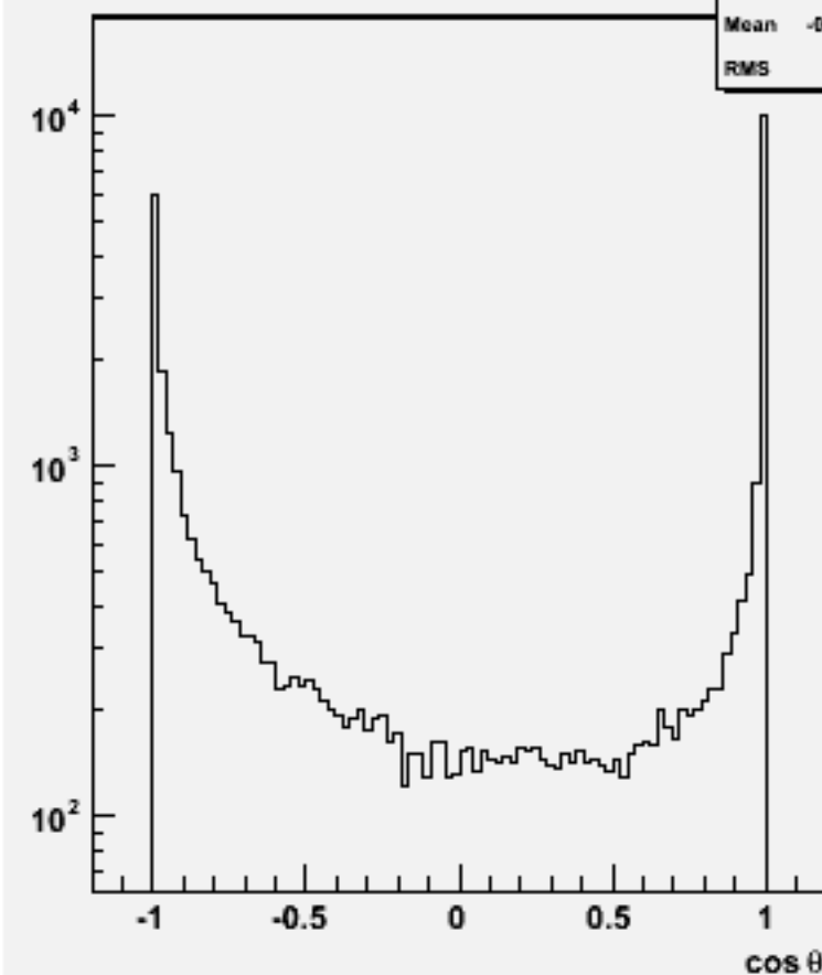
Jet cos \theta (All jets)w103878 ae1_e1e1e1dd_o
