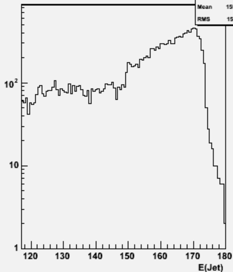
Jet energies(All jets)w103877 ae1_e1e1e1dd_o
