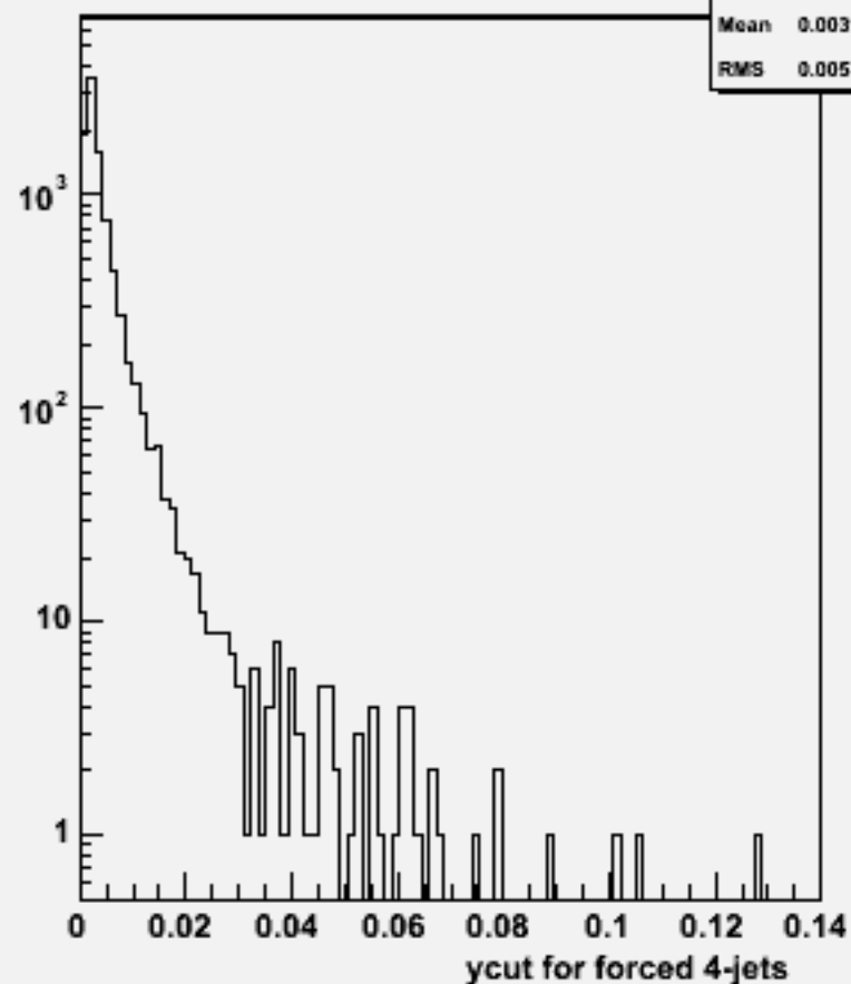
Ycut for 4-jets :w103877 ae1_e1e1e1dd_o
