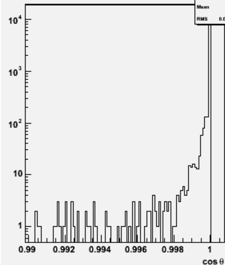
Jet cos \theta (All jets)w103877 ae1_e1e1e1dd_o
