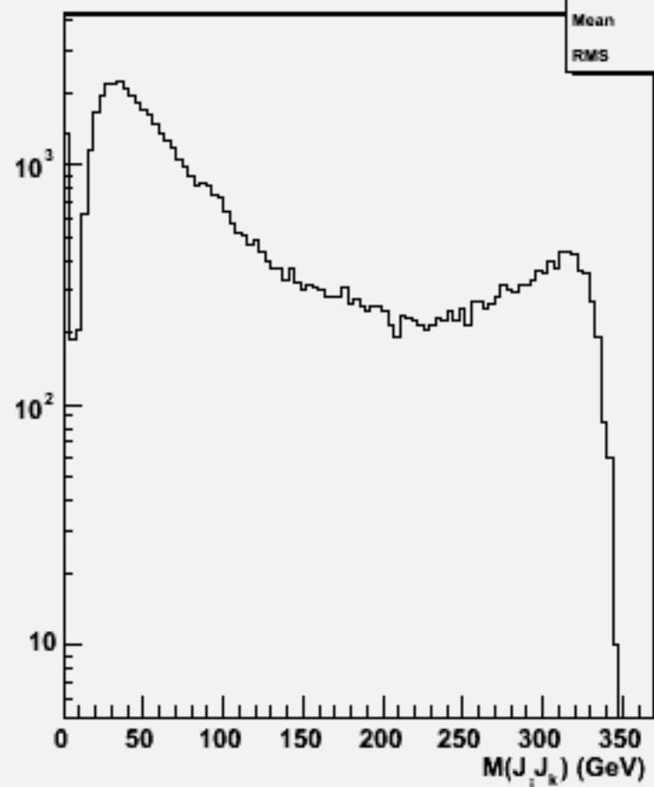
2jets mass(All comb)w103877 ae1_e1e1e1dd_o
