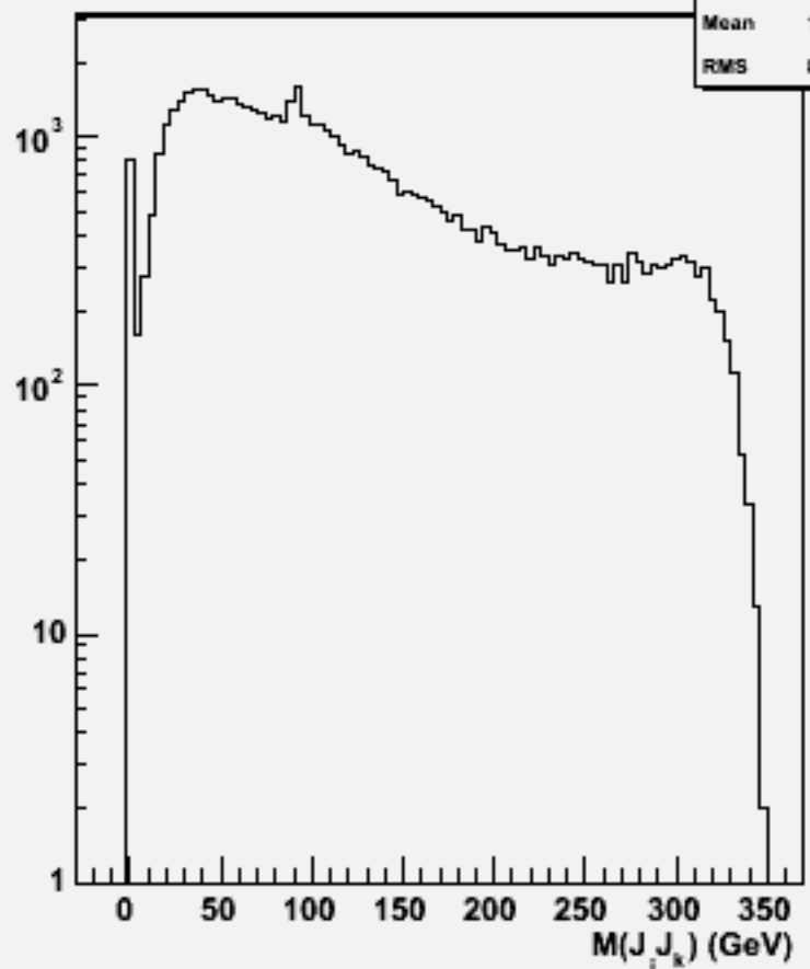
2jets mass(All comb)w103876 ae1_e1e1e1dd_o
