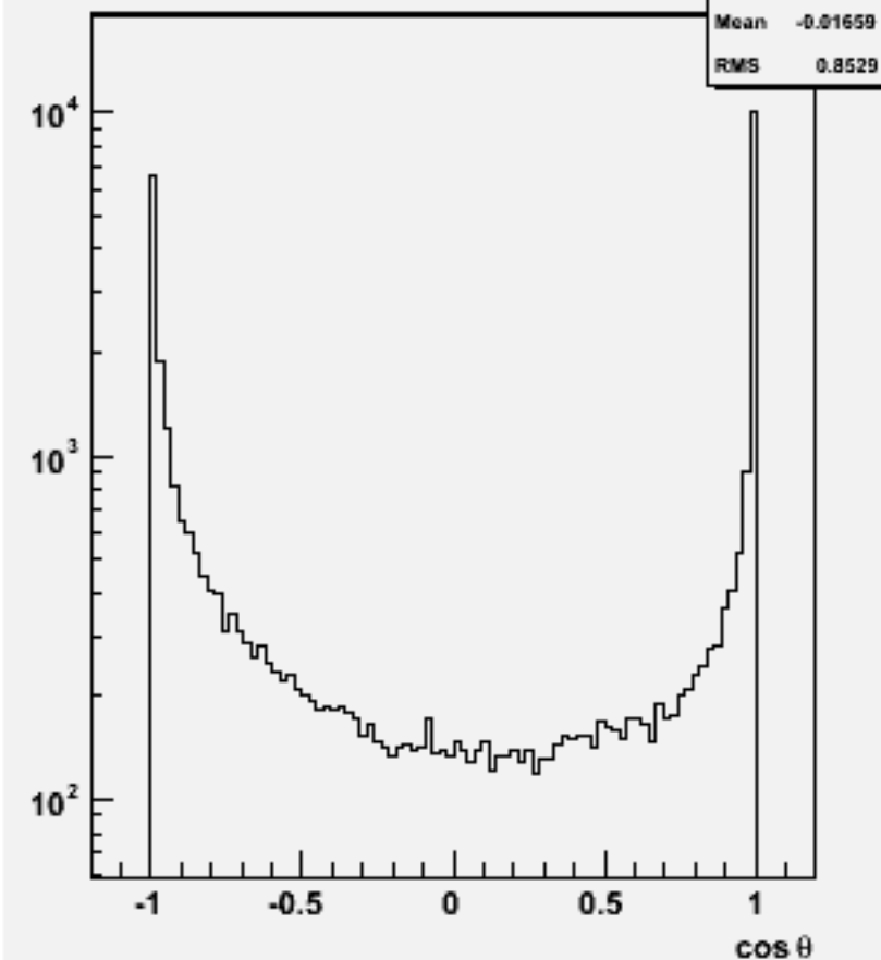
Jet cos theta (All jets)w103876 ae1_e1e1e1dd_o
