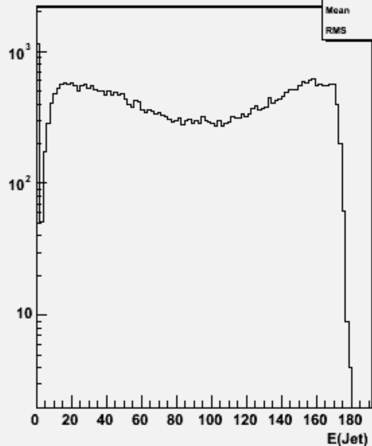
Jet energies(All jets)w103876 ae1_e1e1e1dd_o
