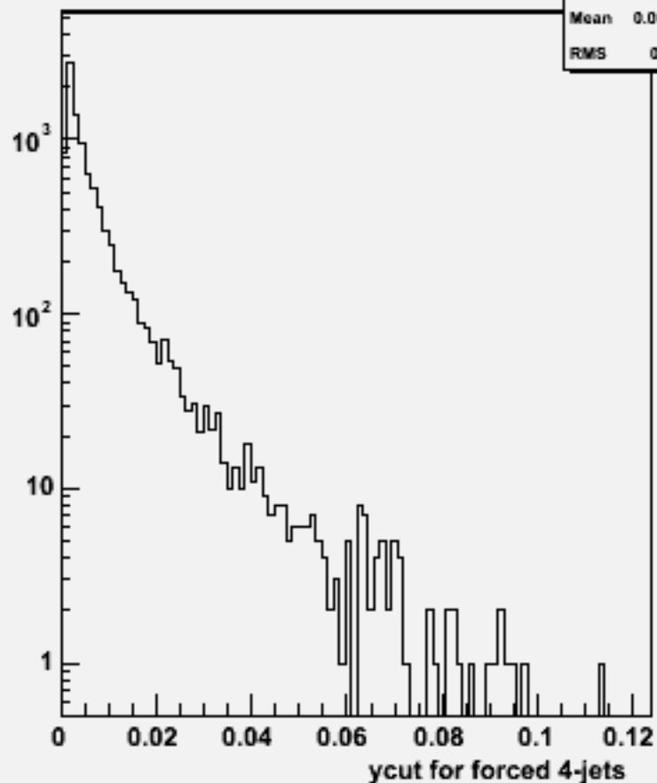
Ycut for 4-jets :w103876 ae1_e1e1e1dd_o
