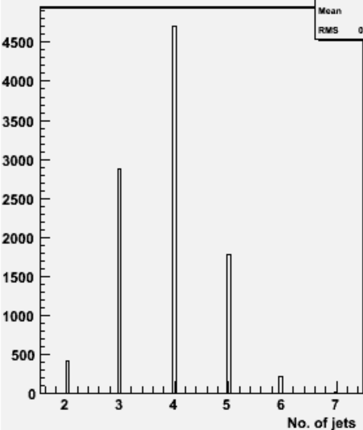
No. jets (ycut=0.001) : w103873 ae1_e1e1e1e3e3_o
