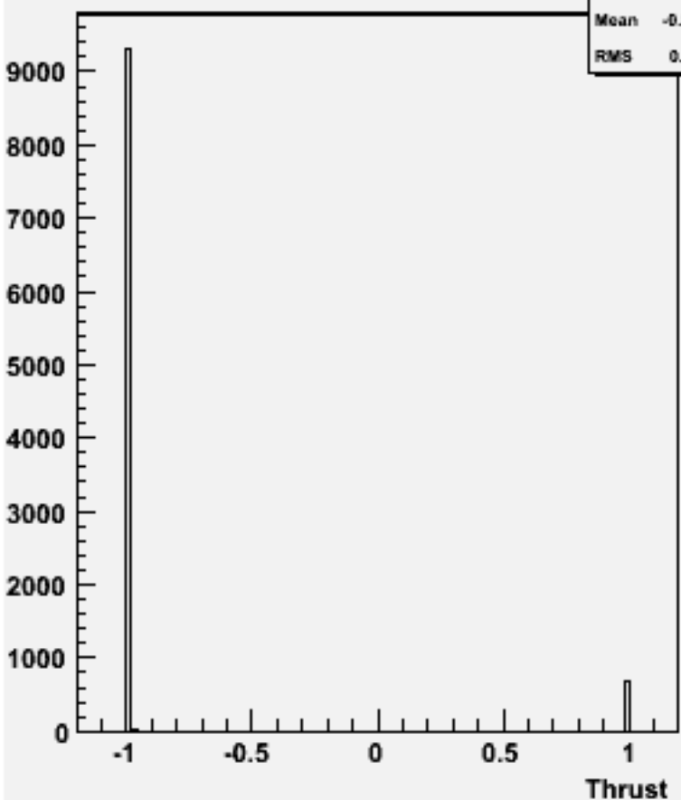
cos \Theta (thrust) w103873 ae1_e1e1e1e3e3_o
