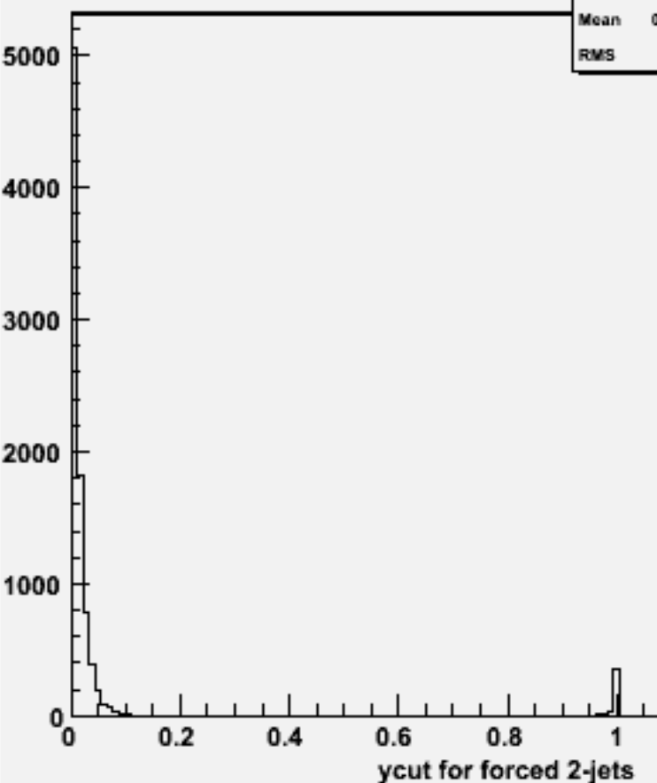
Ycut for 2-jets :w103873 ae1_e1e1e1e3e3_o
