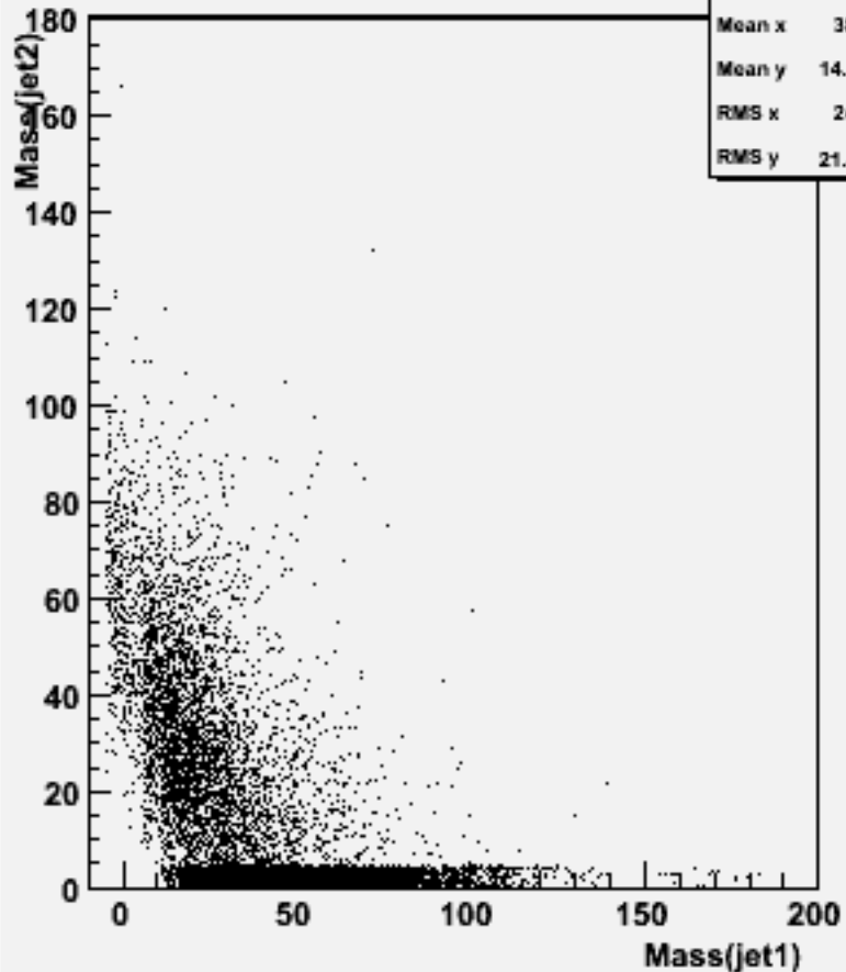
Jet mass for forced 2-jets : w103873 ae1_e1e1e1e3e3_o
