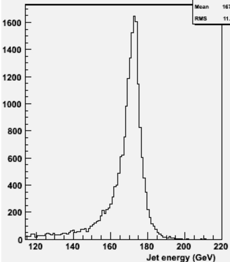
energy for 2-jets :w103873 ae1_e1e1e1e3e3_o
