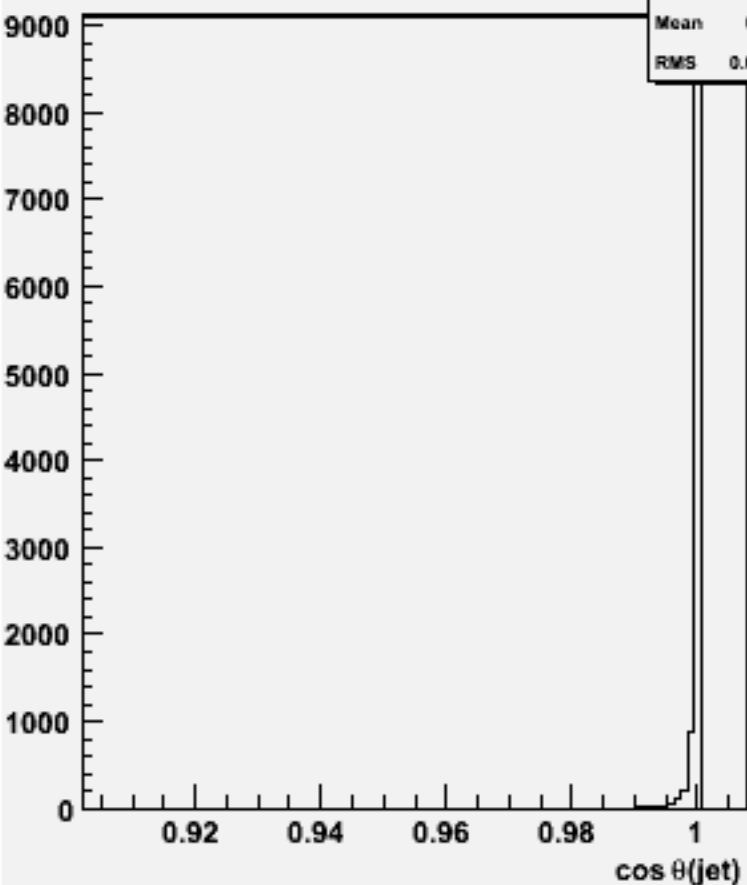
cos \Theta for 2-jets :w103873 ae1_e1e1e1e3e3_o
