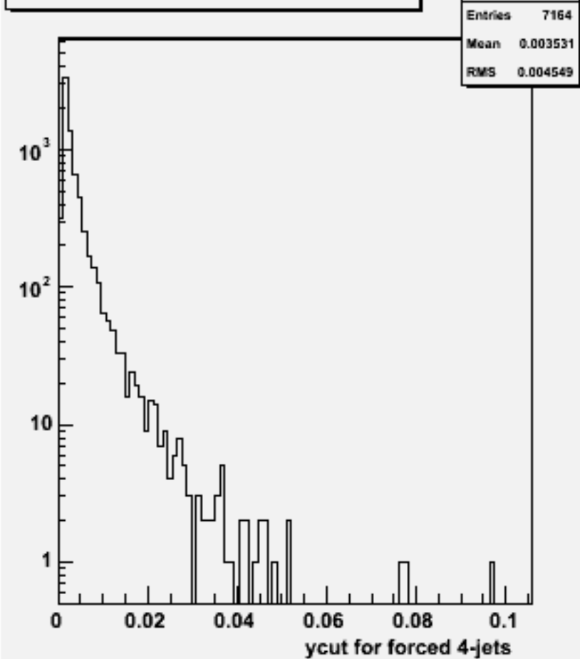
Ycut for 4-jets :w103872 ae1_e1e1e1e3e3_o
