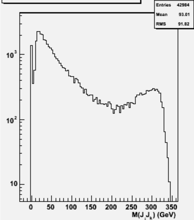
2jets mass(All comb)w103872 ae1_e1e1e1e3e3_o
