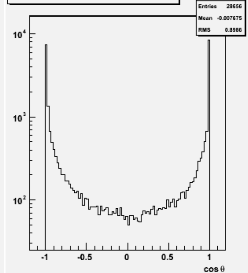
Jet cos theta (All jets)w103872 ae1_e1e1e1e3e3_o
