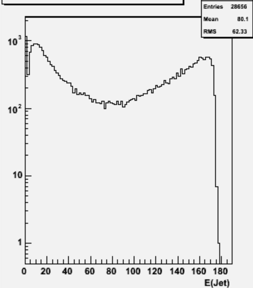
Jet energies(All jets)w103872 ae1_e1e1e1e3e3_o
