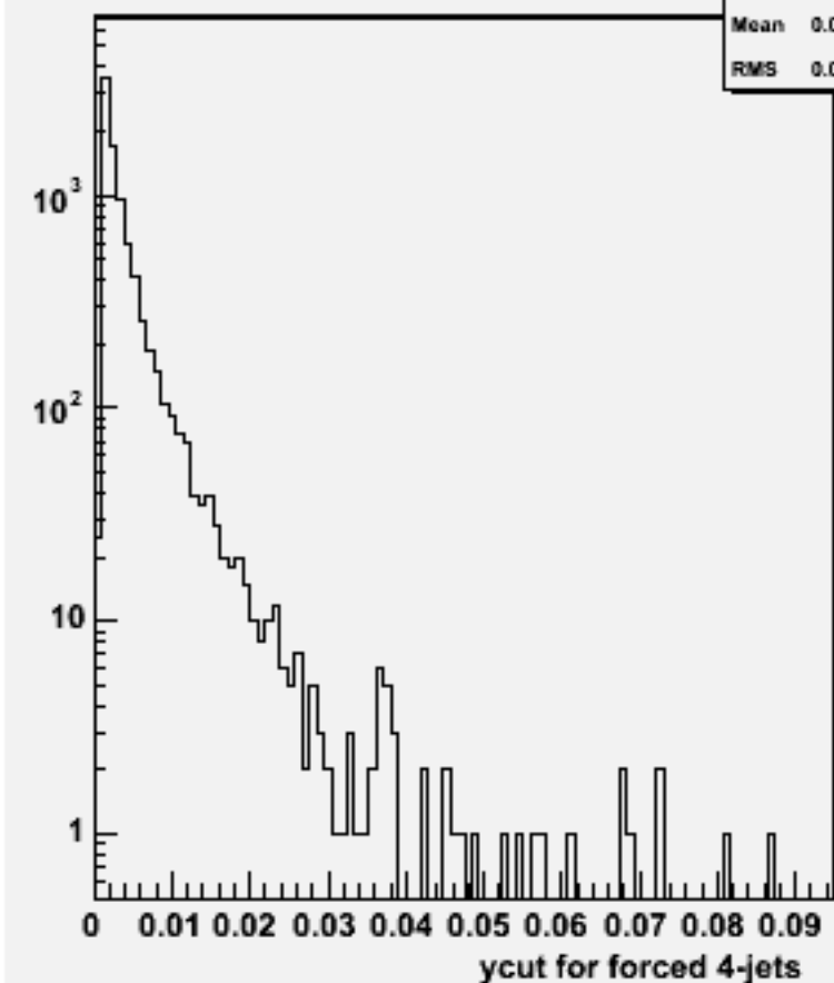
Ycut for 4-jets :w103870 ae1_e1e1e1e2e2_o
