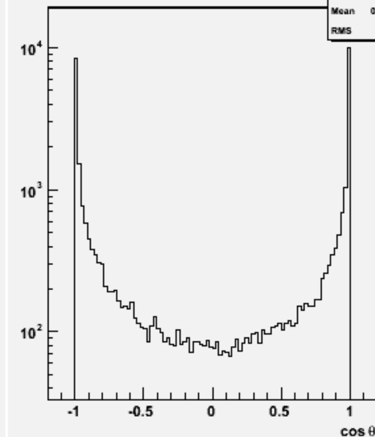
Jet cos θ (All jets)w103870 ae1_e1e1e1e2e2_o
