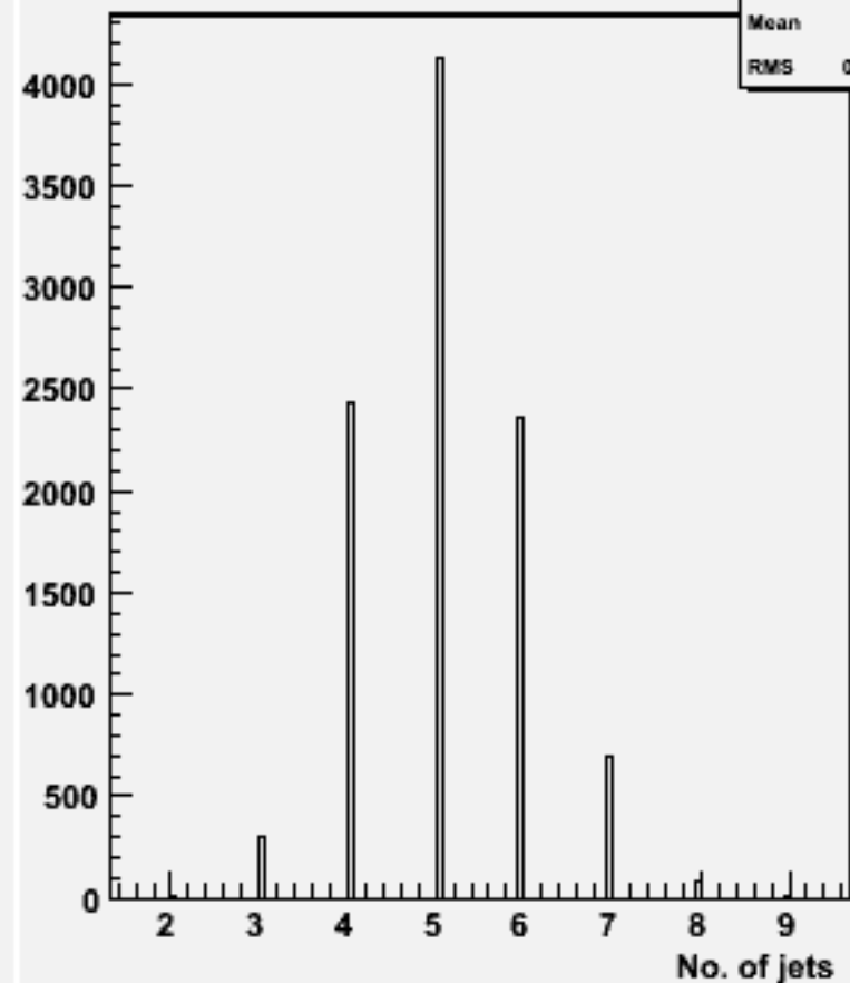
No. jets (ycut=0.001) : w103863 ae1_e1ccbb_o
