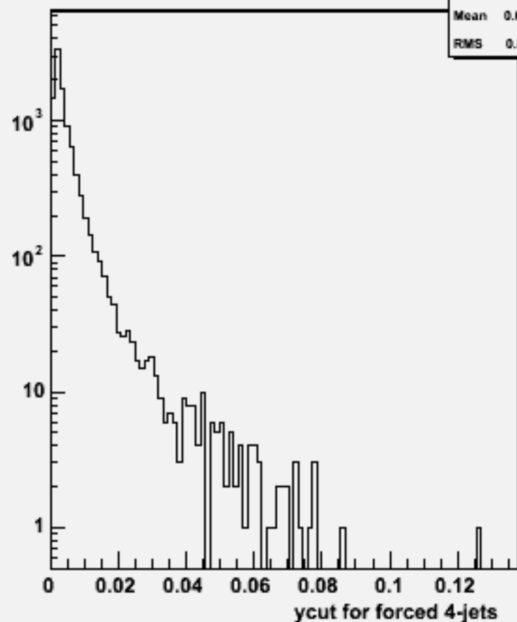
Ycut for 4-jets :w103863 ae1_e1ccbb_o
