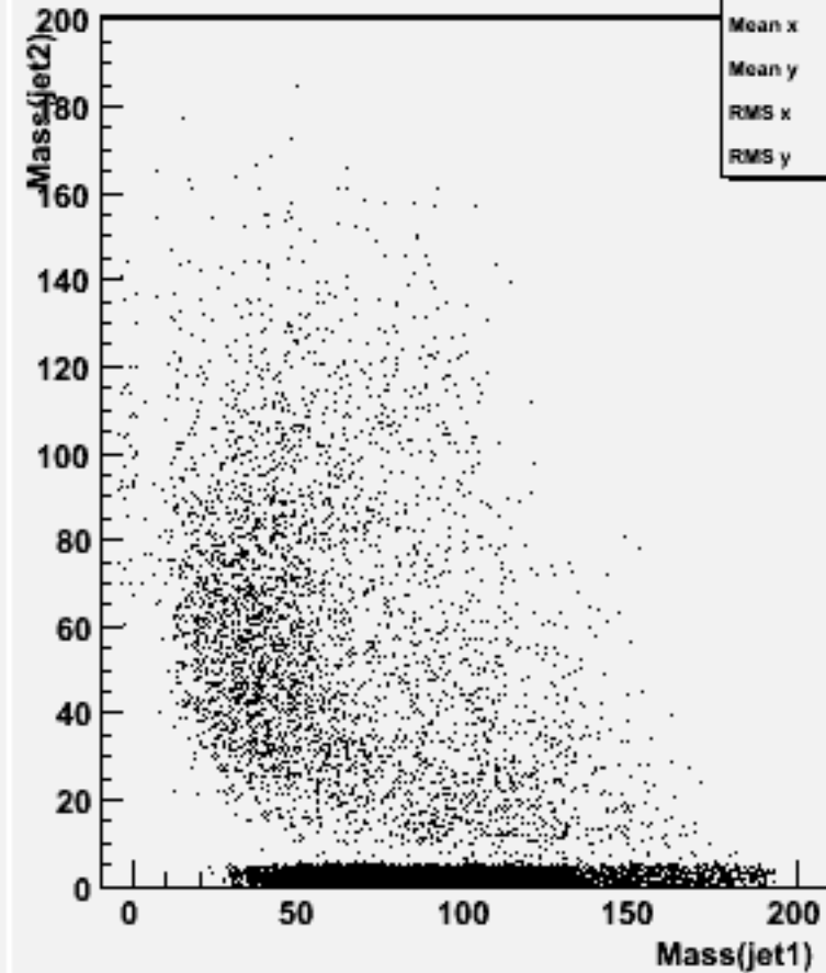
Jet mass for forced 2-jets : w103863 ae1_e1ccbb_o
