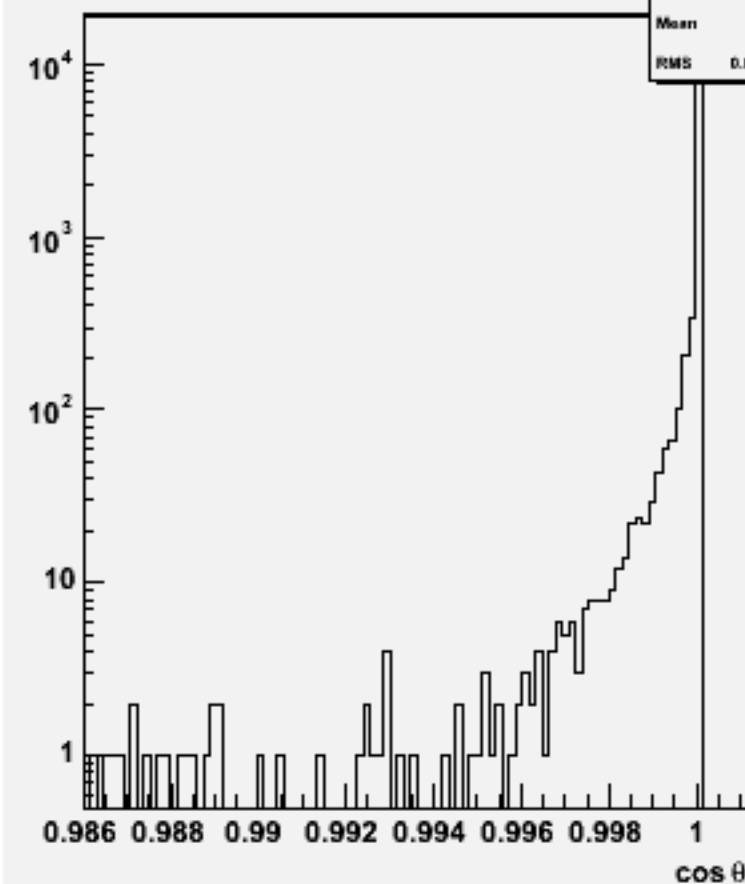
Jet cos \theta (All jets)w103863 ae1_e1ccbb_o
