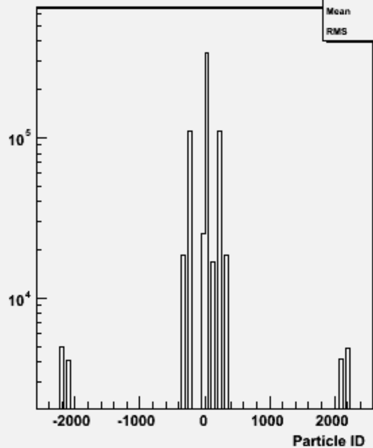
Particle ID : w103863 ae1_e1ccbb_o
