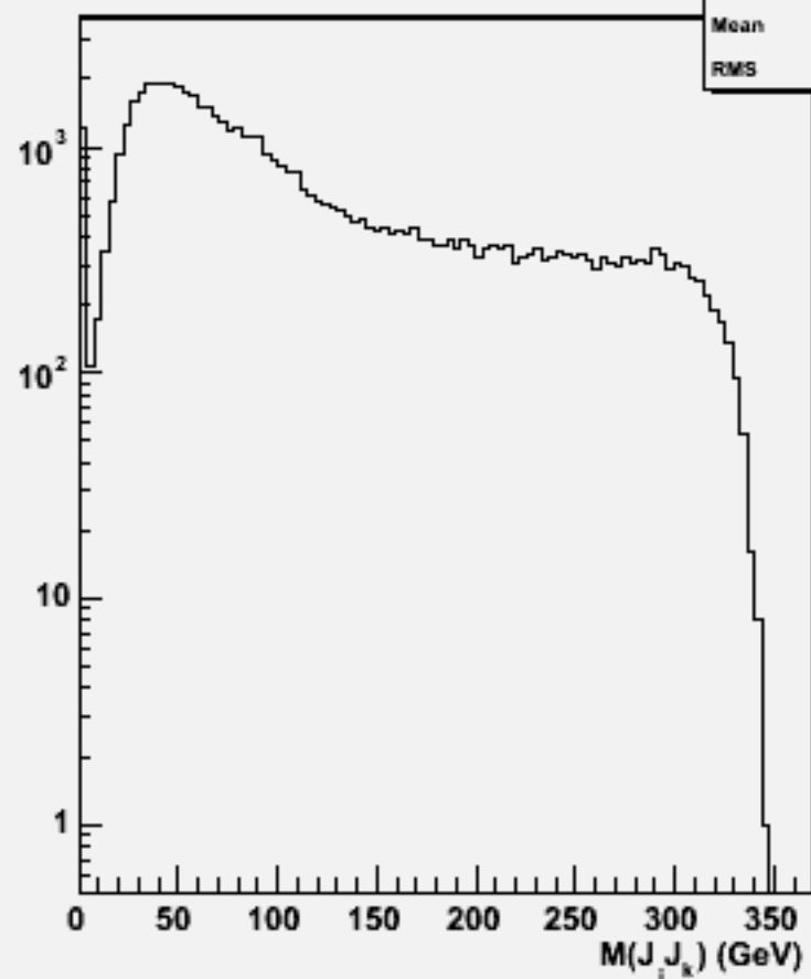
2jets mass(All comb)w103863 ae1_e1ccbb_o
