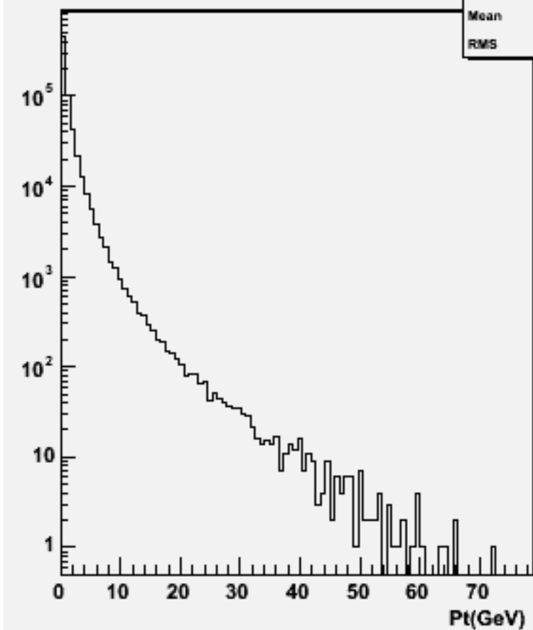
Particle Pt : w103863 ae1_e1ccbb_o
