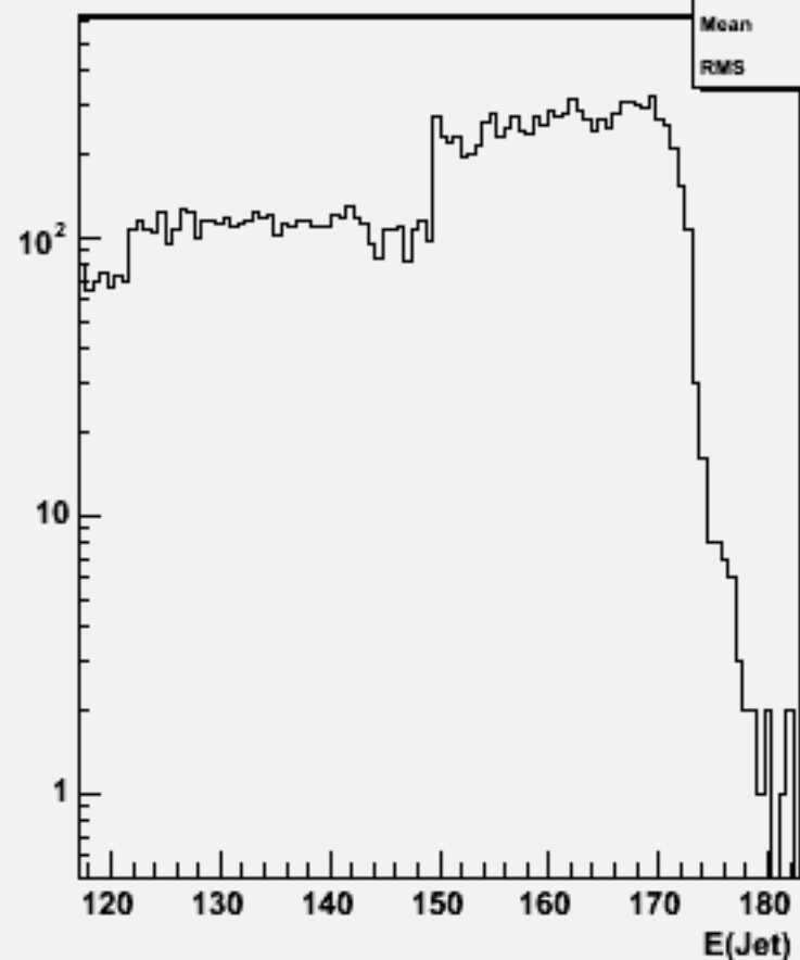
Jet energies(All jets)w103863 ae1_e1ccbb_o
