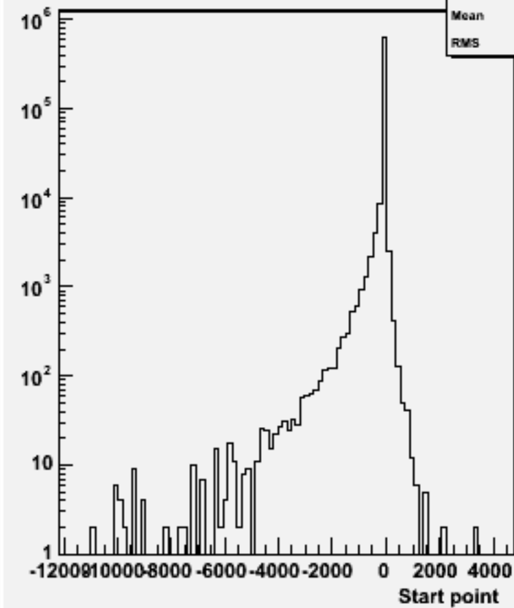
Start point Z : w103863 ae1_e1ccbb_o
