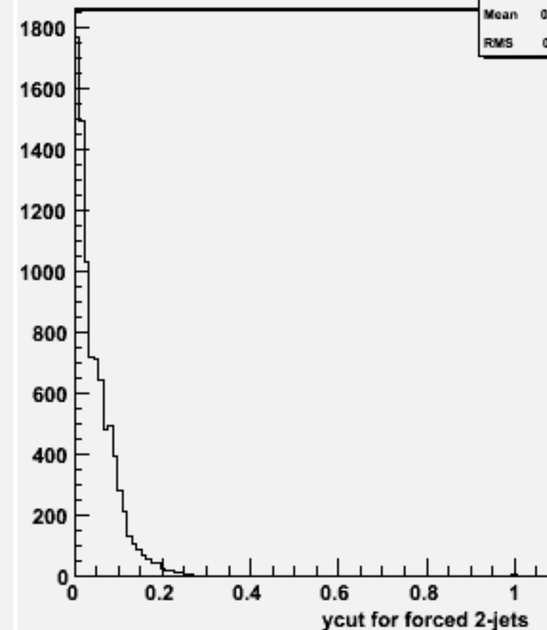
Ycut for 2-jets :w103863 ae1_e1ccbb_o
