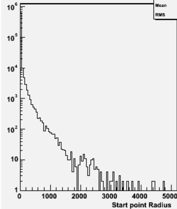
Start point R : w103863 ae1_e1ccbb_o
