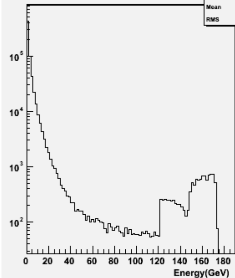
Particle Energy : w103863 ae1_e1ccbb_o
