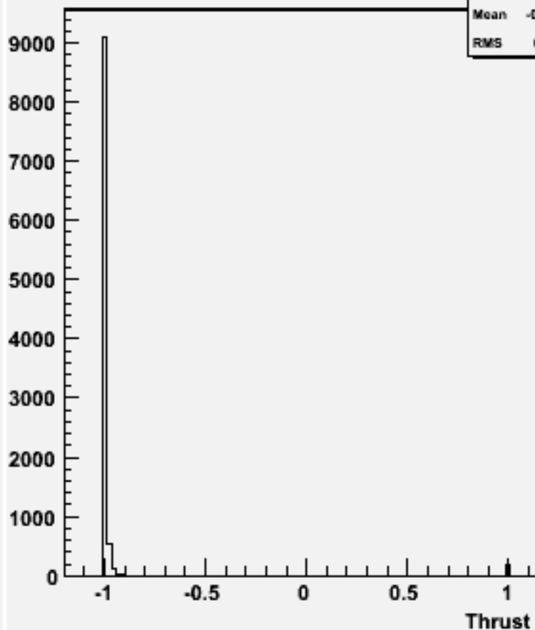
cos \Theta (thrust) w103863 ae1_e1ccbb_o
