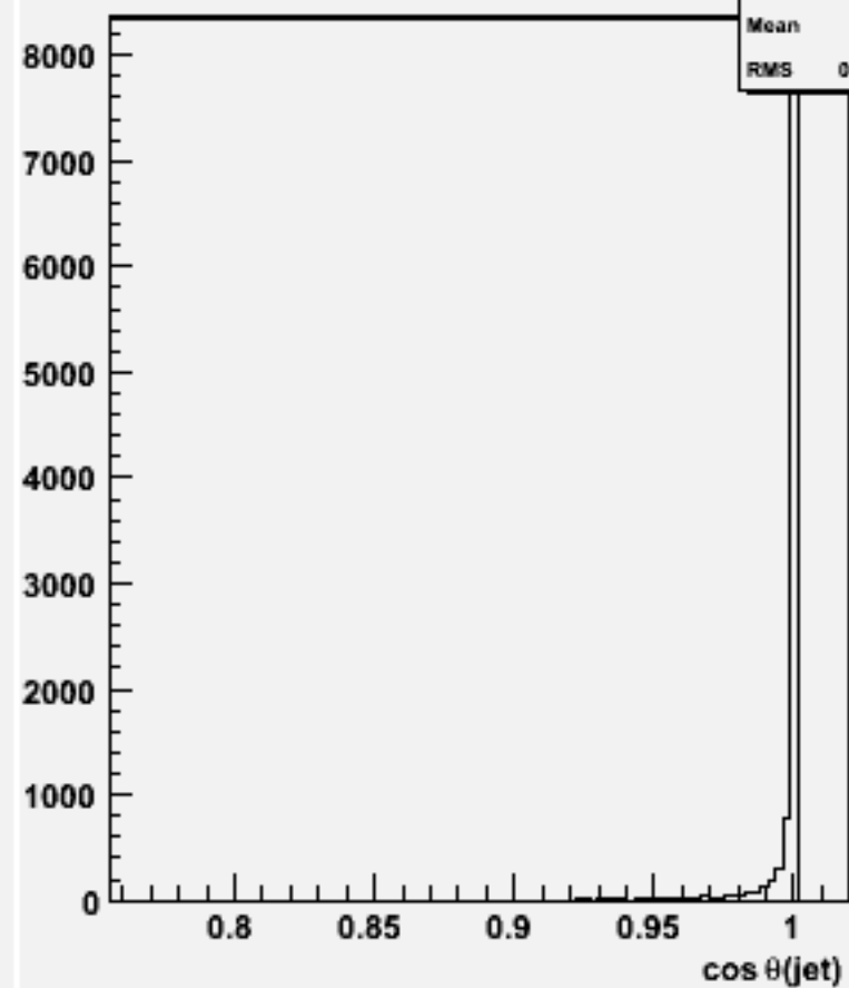
cos \Theta for 2-jets :w103863 ae1_e1ccbb_o
