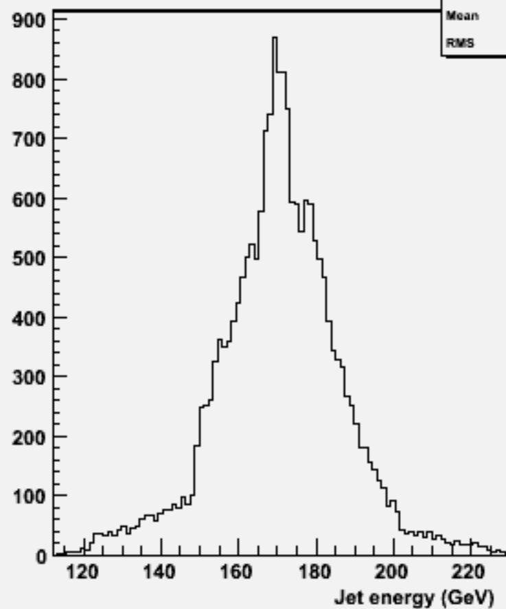
energy for 2-jets :w103863 ae1_e1ccbb_o
