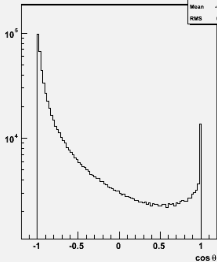
Particle cos \theta : w103863 ae1_e1ccbb_o
