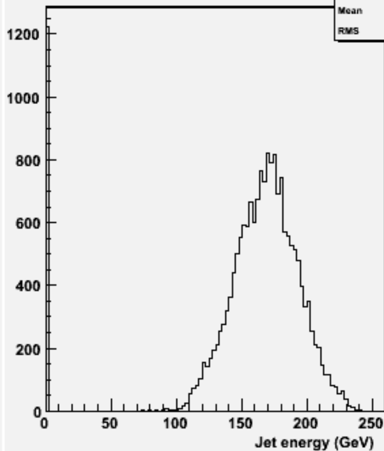
energy for 2-jets :w103862 ae1_e1ccbb_o
