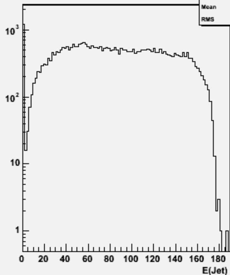
Jet energies(All jets)w103862 ae1_e1ccbb_o
