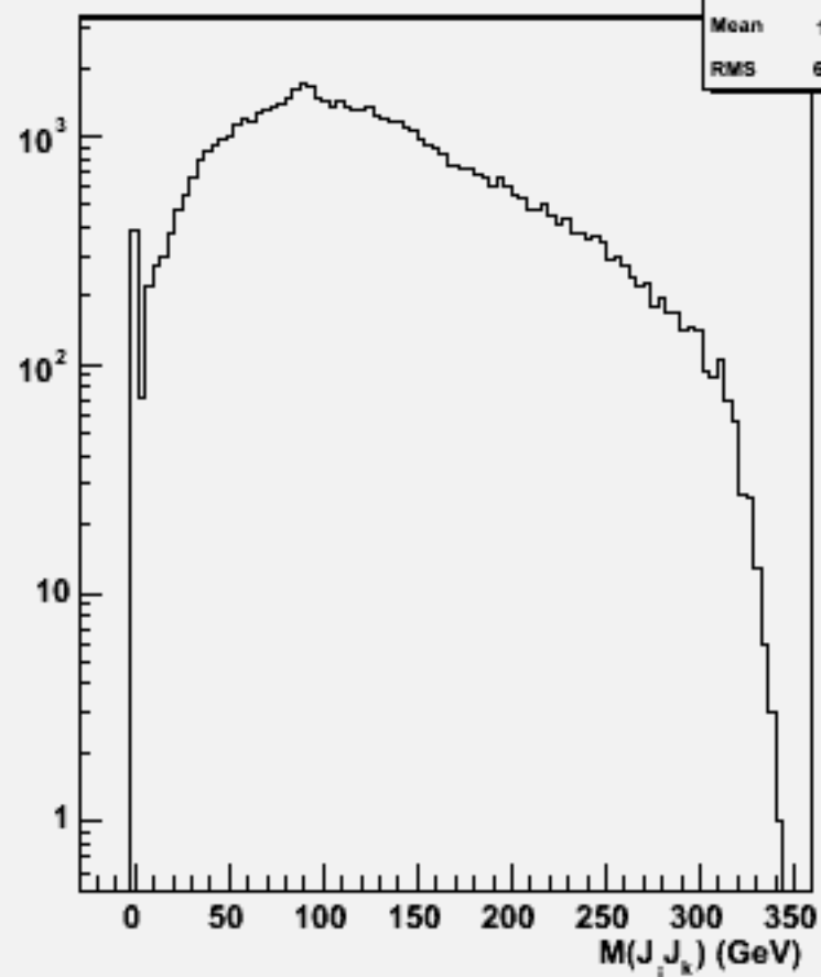
2jets mass(All comb)w103862 ae1_e1ccbb_o
