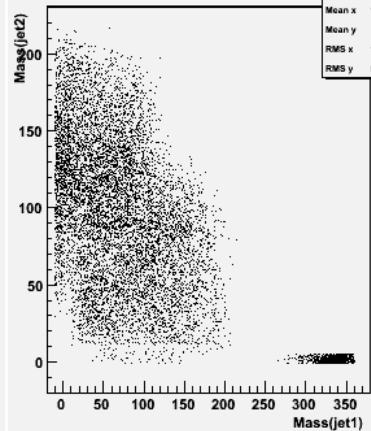
Jet mass for forced 2-jets : w103862 ae1_e1ccbb_o
