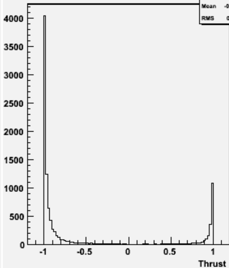
cos \Theta (thrust) w103862 ae1_e1ccbb_o
