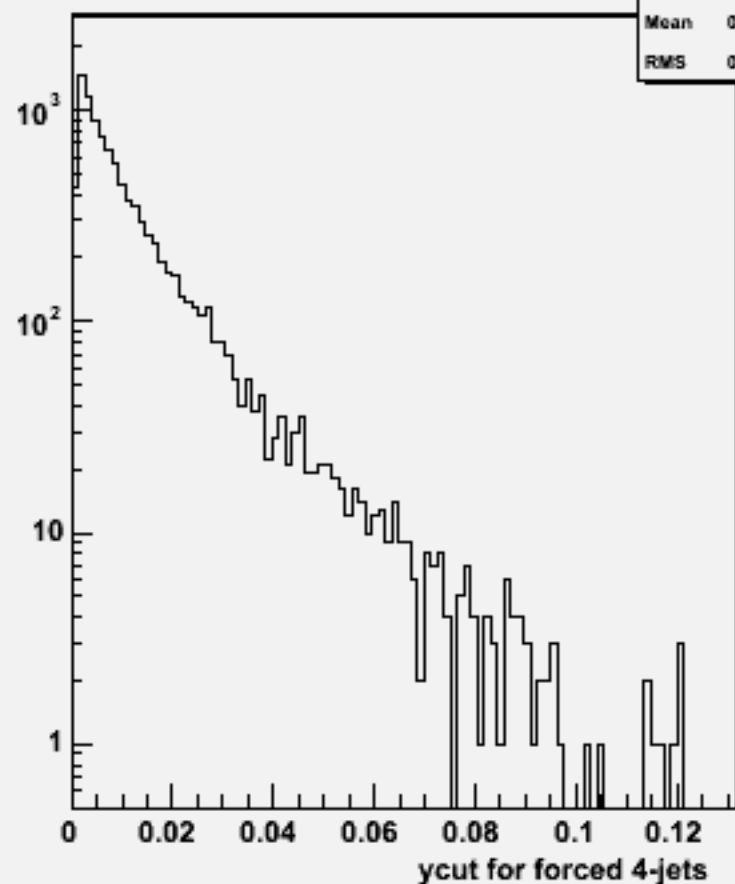
Ycut for 4-jets :w103862 ae1_e1ccbb_o
