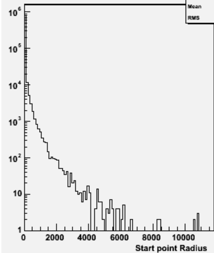
Start point R : w103862 ae1_e1ccbb_o
