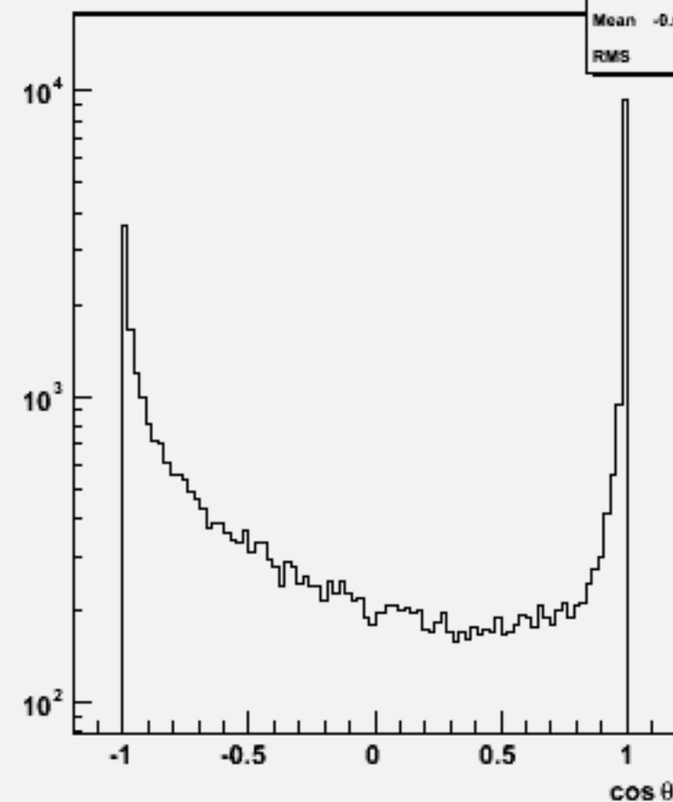
Jet cos \theta (All jets)w103862 ae1_e1ccbb_o
