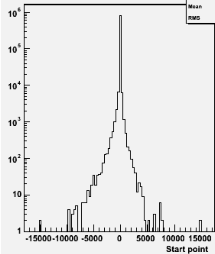
Start point Z : w103862 ae1_e1ccbb_o
