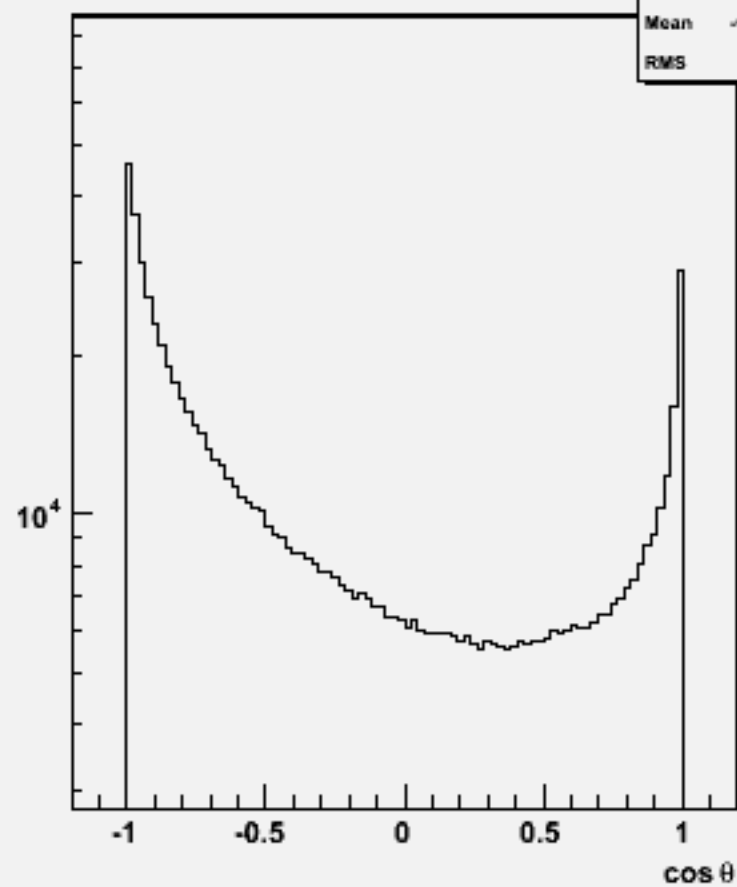
Particle cos \theta : w103862 ae1_e1ccbb_o
