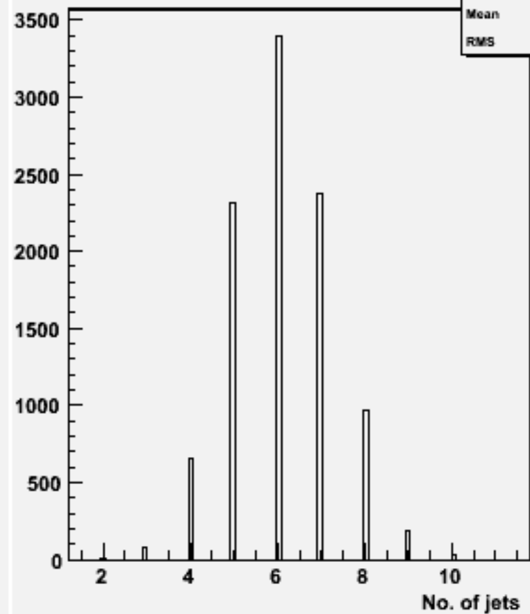
No. jets (ycut=0.001) : w103862 ae1_e1ccbb_o
