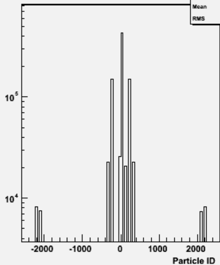
Particle ID : w103862 ae1_e1ccbb_o
