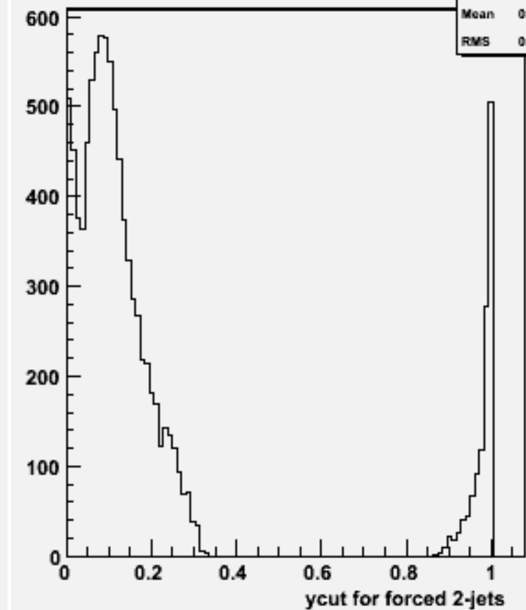
Ycut for 2-jets :w103862 ae1_e1ccbb_o
