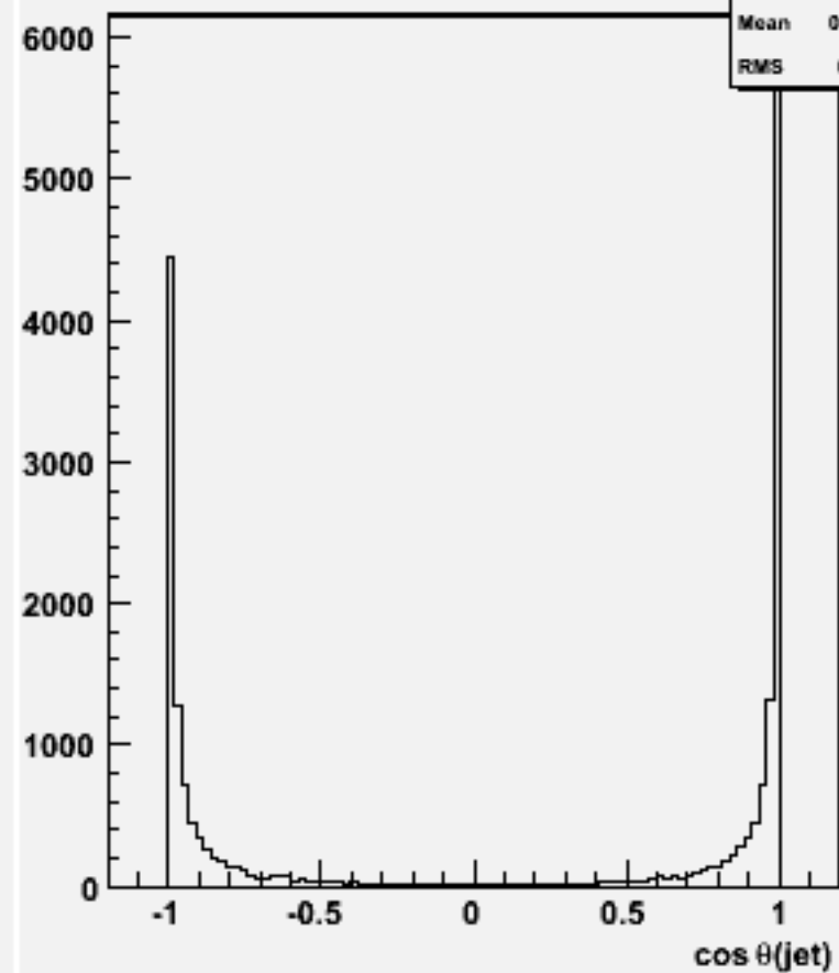
cos \theta for 2-jets :w103862 ae1_e1ccbb_o
