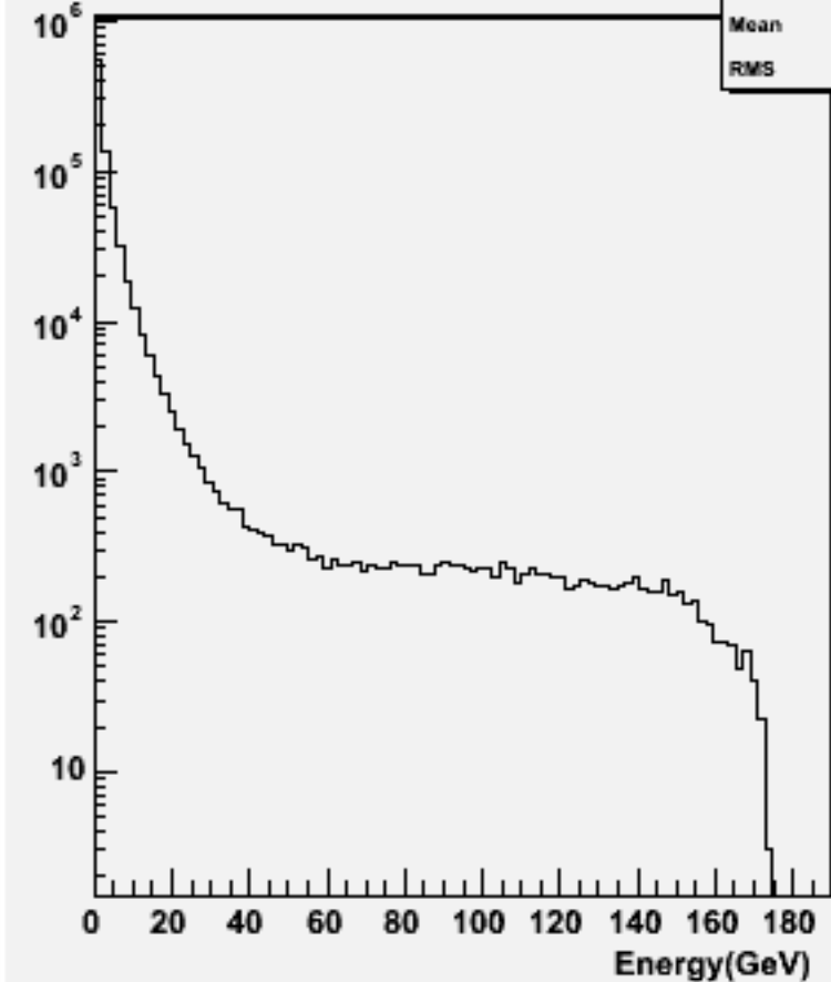
Particle Energy : w103862 ae1_e1ccbb_o
