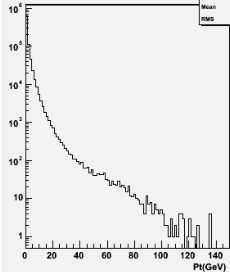
Particle Pt : w103862 ae1_e1ccbb_o
