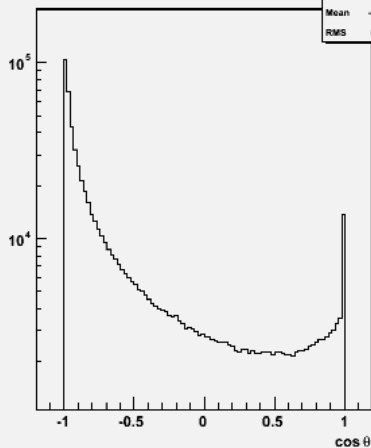
Particle cosθ : w103861 ae1_e1ccbb_o
