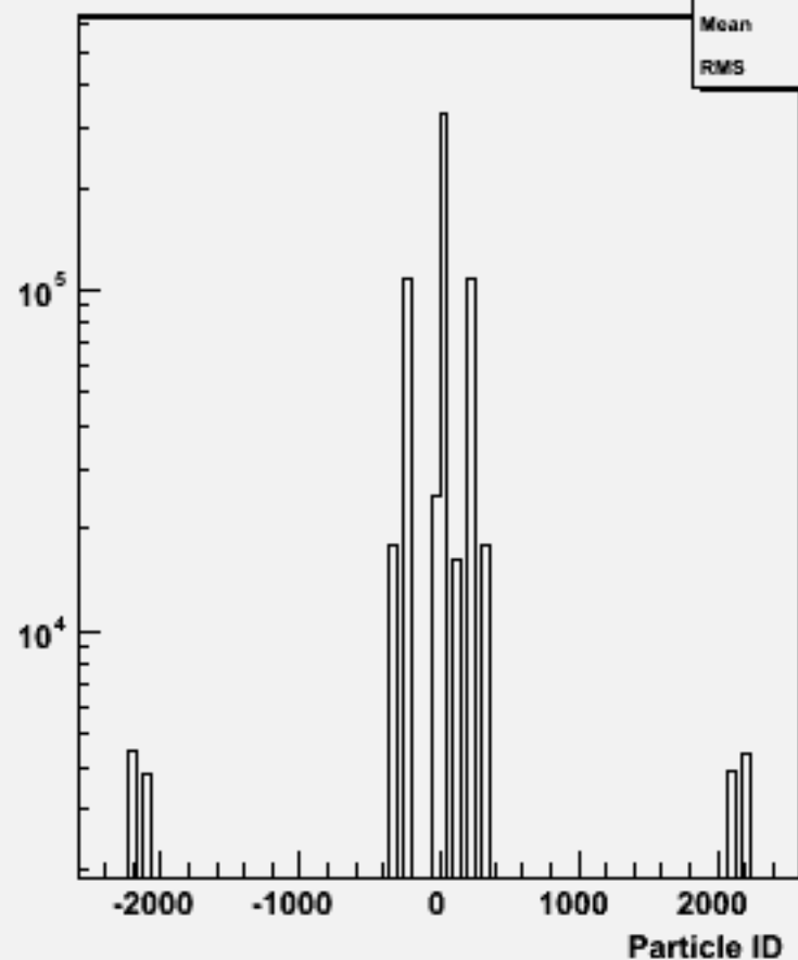
Particle ID : w103861 ae1_e1ccbb_o
