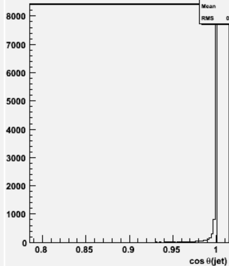
cos \Theta for 2-jets :w103861 ae1_e1ccbb_o
