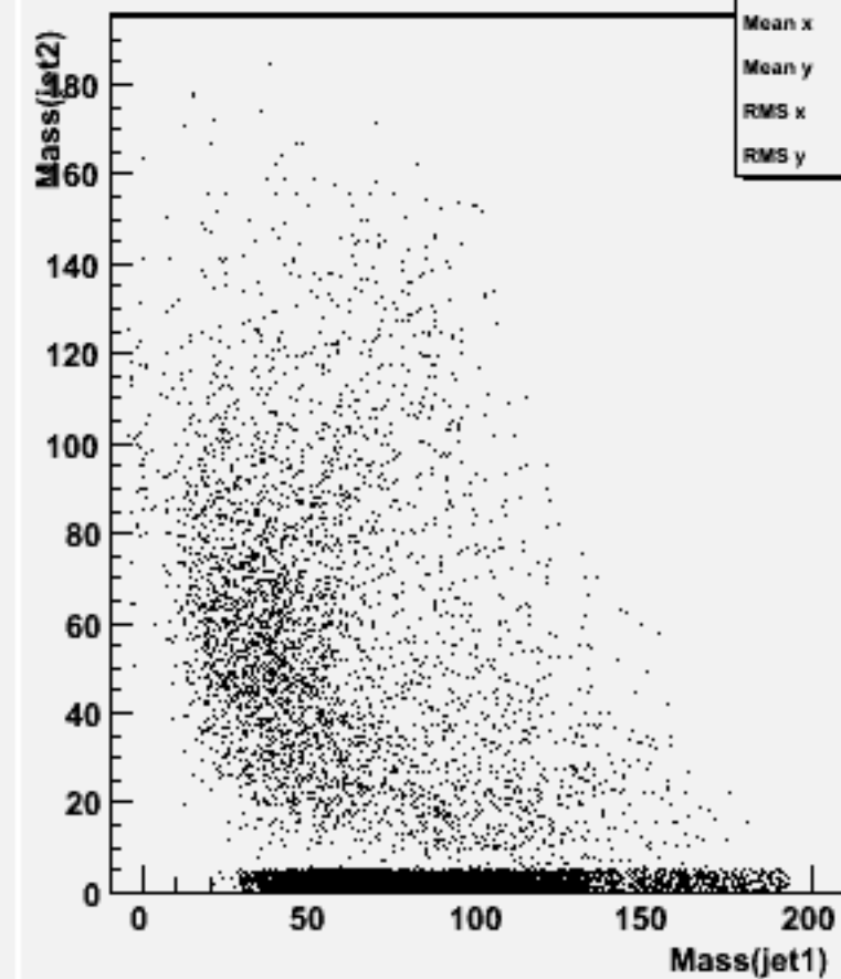
Jet mass for forced 2-jets : w103861 ae1_e1ccbb_o
