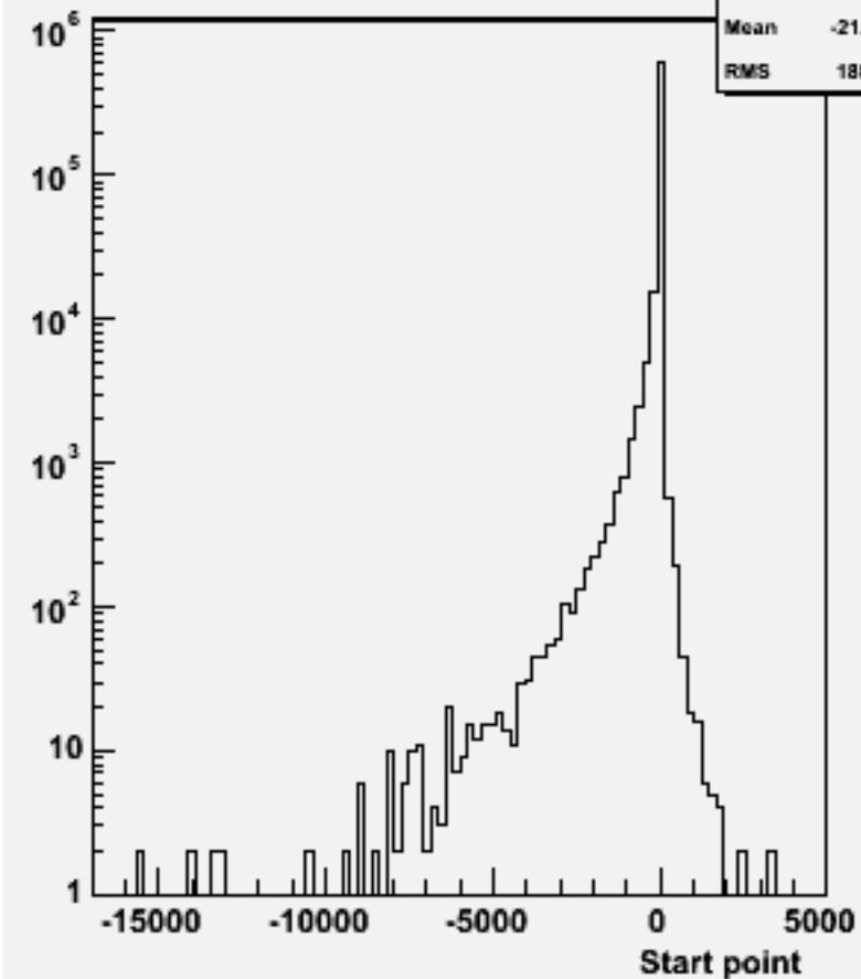
Start point Z : w103861 ae1_e1ccbb_o
