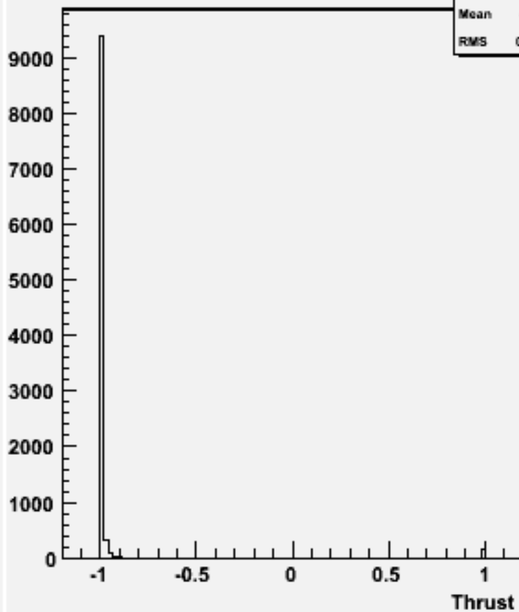
cos \Theta (thrust) w103861 ae1_e1ccbb_o
