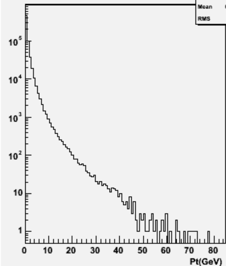
Particle Pt : w103861 ae1_e1ccbb_o
