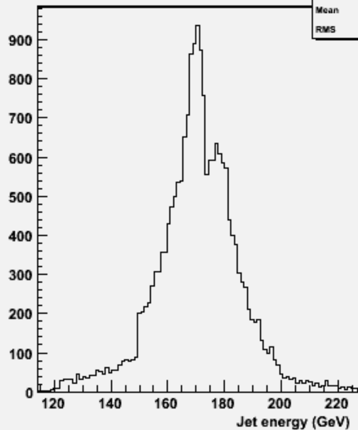
energy for 2-jets :w103861 ae1_e1ccbb_o
