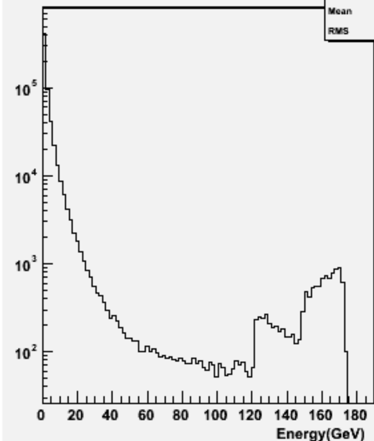
Particle Energy : w103861 ae1_e1ccbb_o
