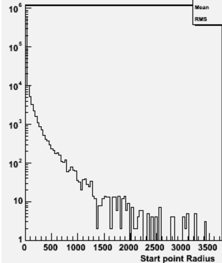
Start point R : w103861 ae1_e1ccbb_o
