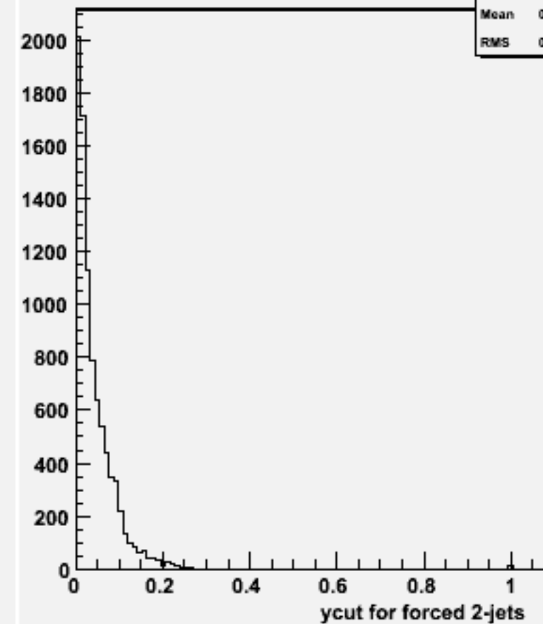
Ycut for 2-jets :w103861 ae1_e1ccbb_o
