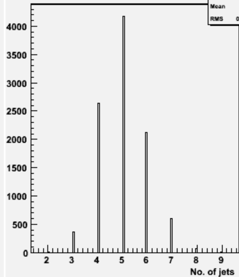
No. jets (ycut=0.001) : w103861 ae1_e1ccbb_o
