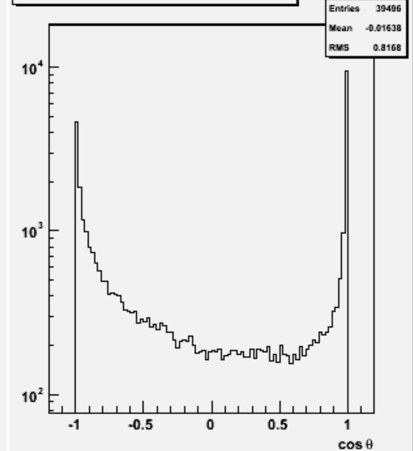
Jet cos \theta (All jets)w103860 ae1_e1ccbb_o
