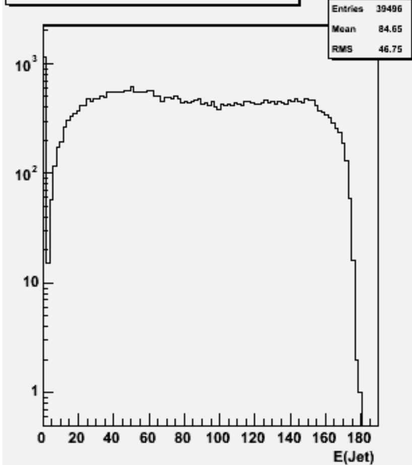
Jet energies(All jets)w103860 ae1_e1ccbb_o
