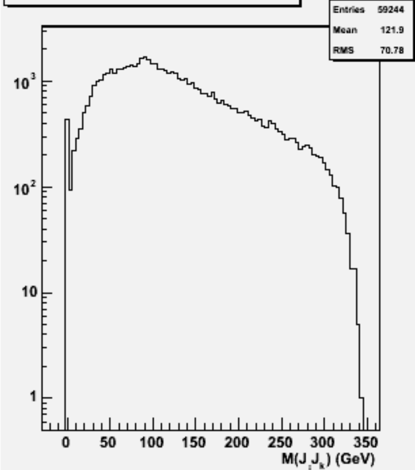
2jets mass(All comb)w103860 ae1_e1ccbb_o
