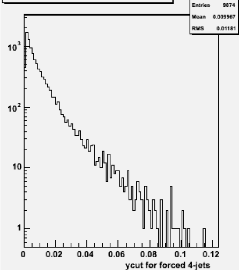
Ycut for 4-jets :w103860 ae1_e1ccbb_o
