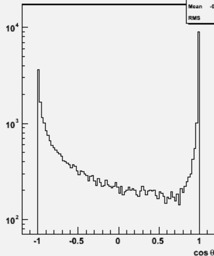
Jet cos \theta (All jets)w103858 ae1_e1ccdd_o
