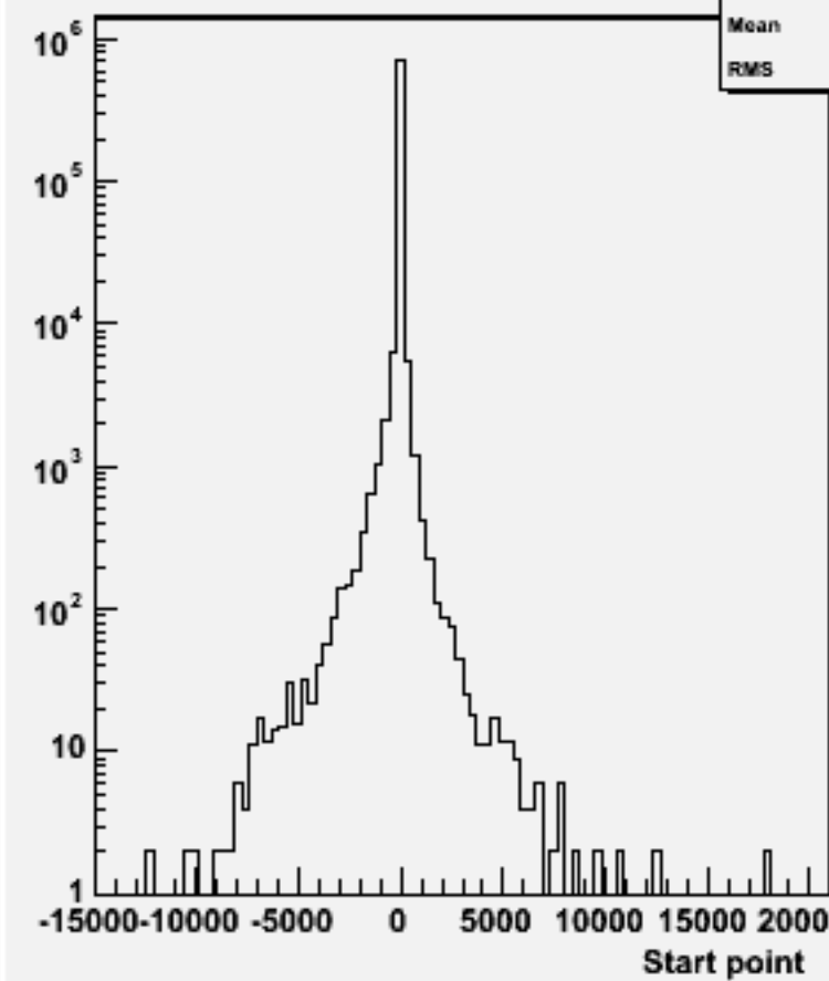
Start point Z : w103858 ae1_e1ccdd_o
