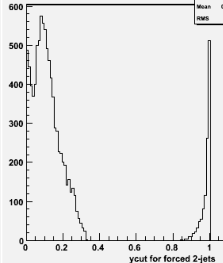
Ycut for 2-jets :w103858 ae1_e1ccdd_o
