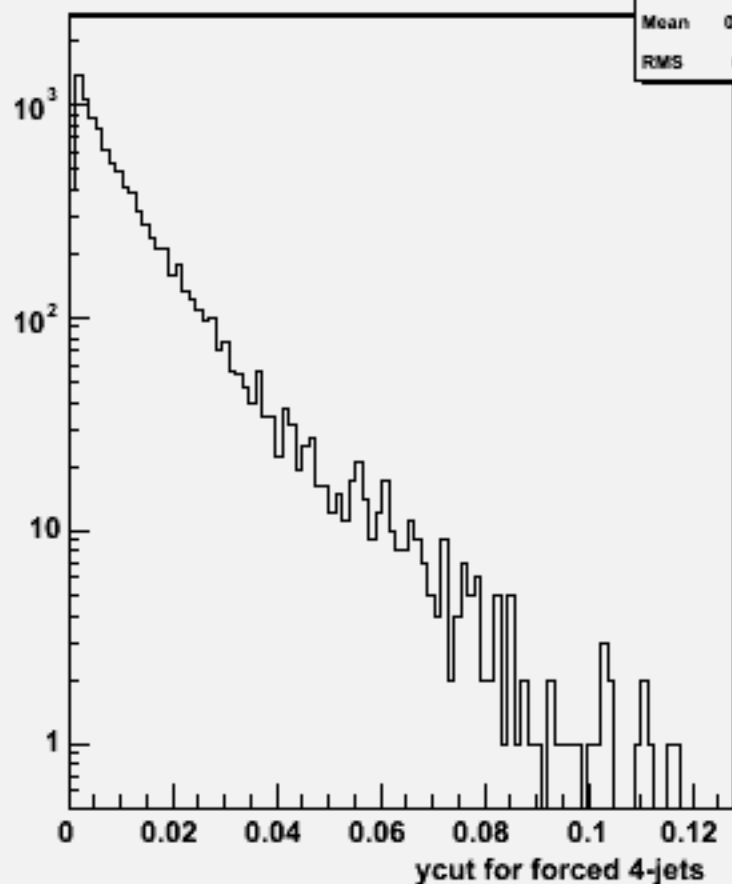
Ycut for 4-jets :w103858 ae1_e1ccdd_o
