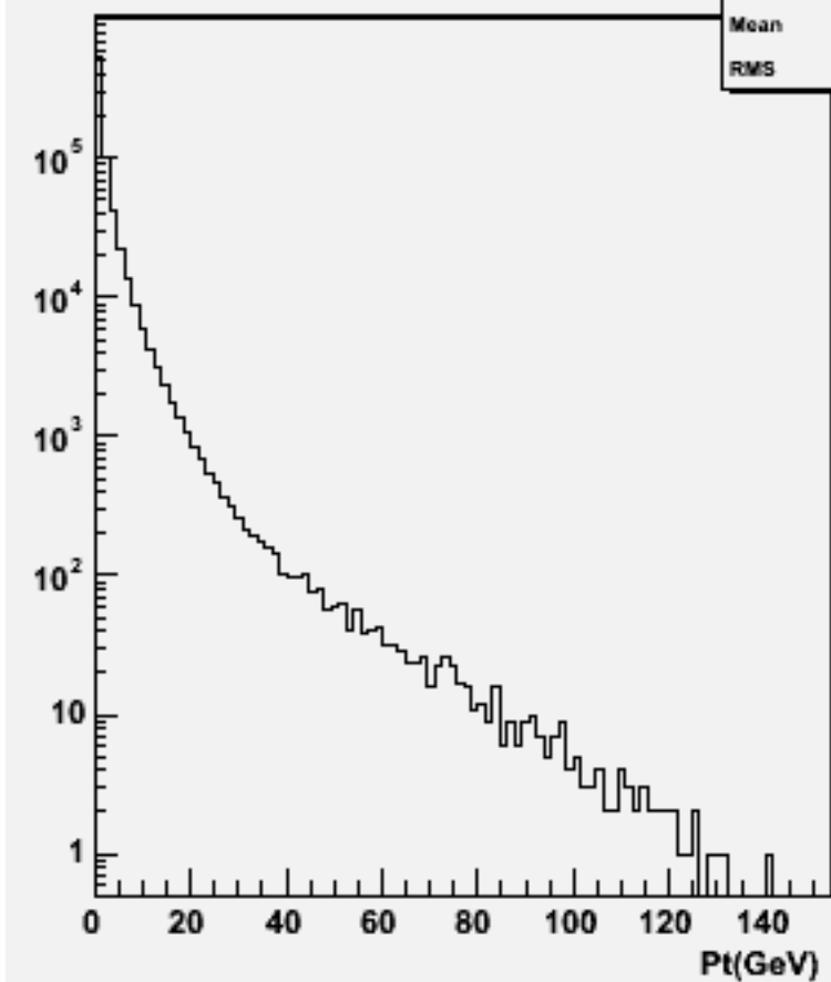
Particle Pt : w103858 ae1_e1ccdd_o
