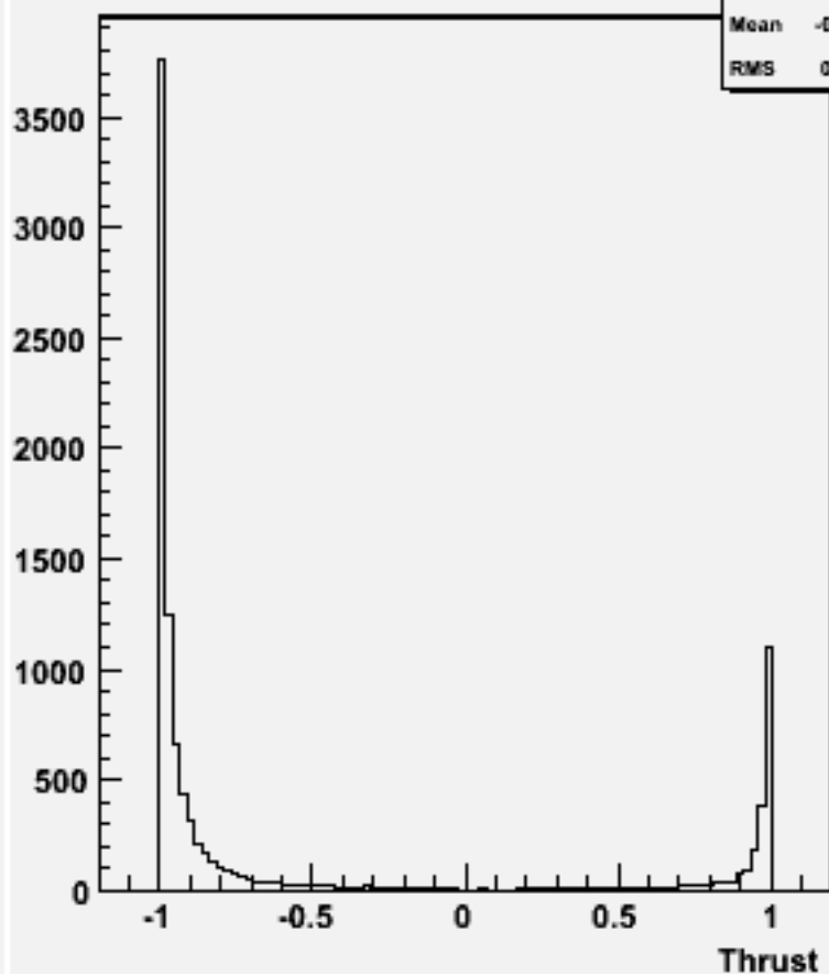
cos \Theta (thrust) w103858 ae1_e1ccdd_o
