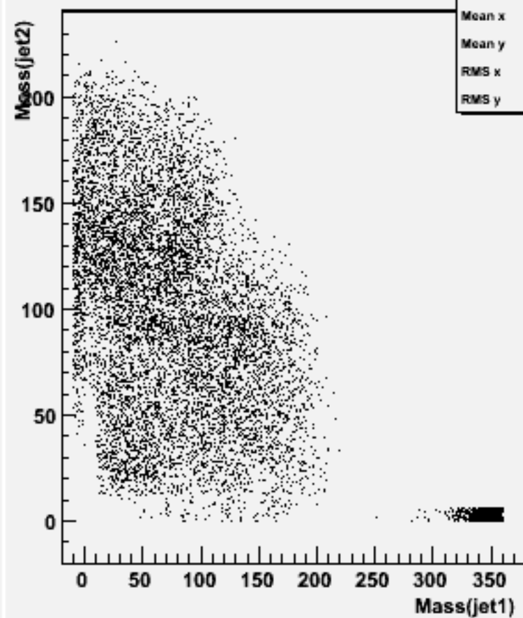
Jet mass for forced 2-jets : w103858 ae1_e1ccdd_o
