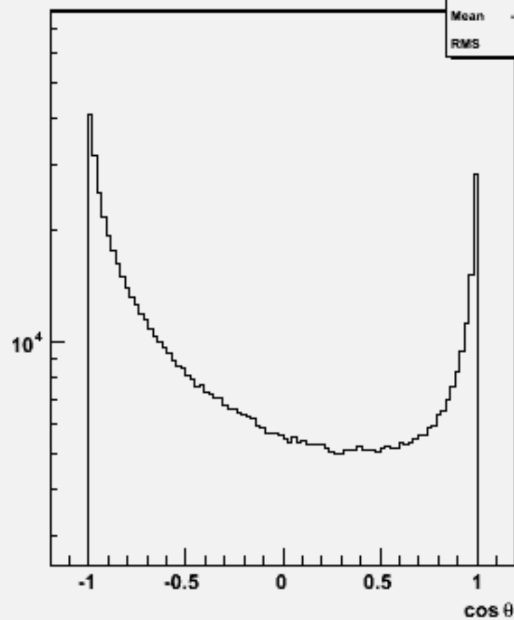
Particle cos \theta : w103858 ae1_e1ccdd_o
