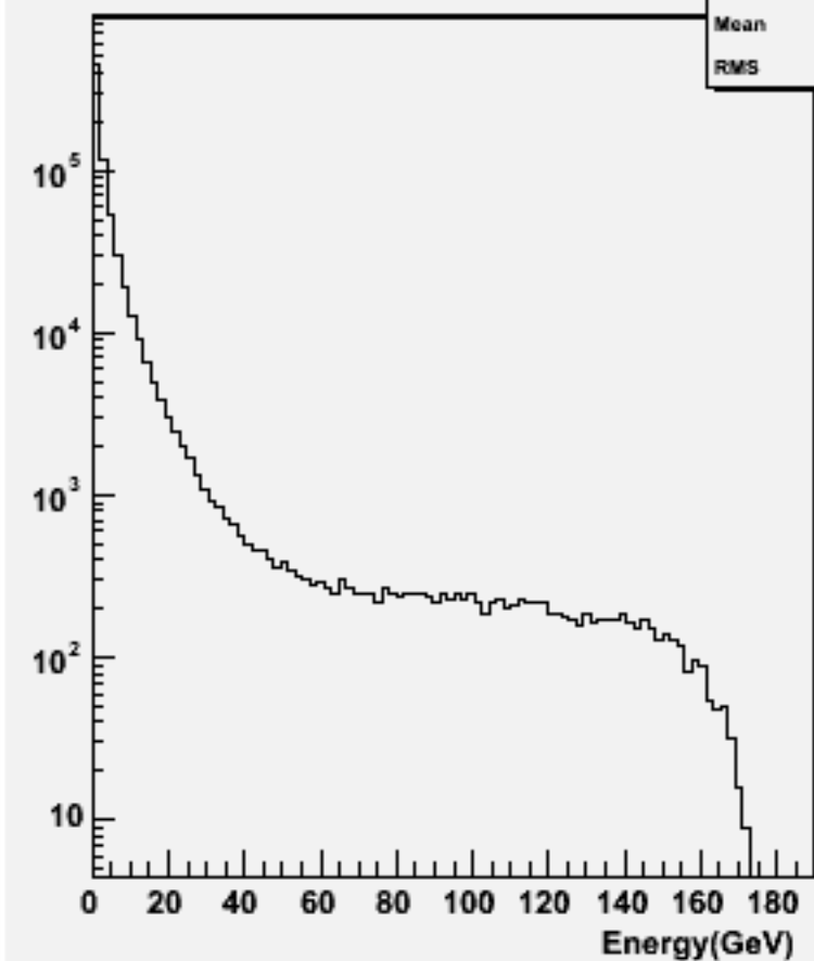
Particle Energy : w103858 ae1_e1ccdd_o
