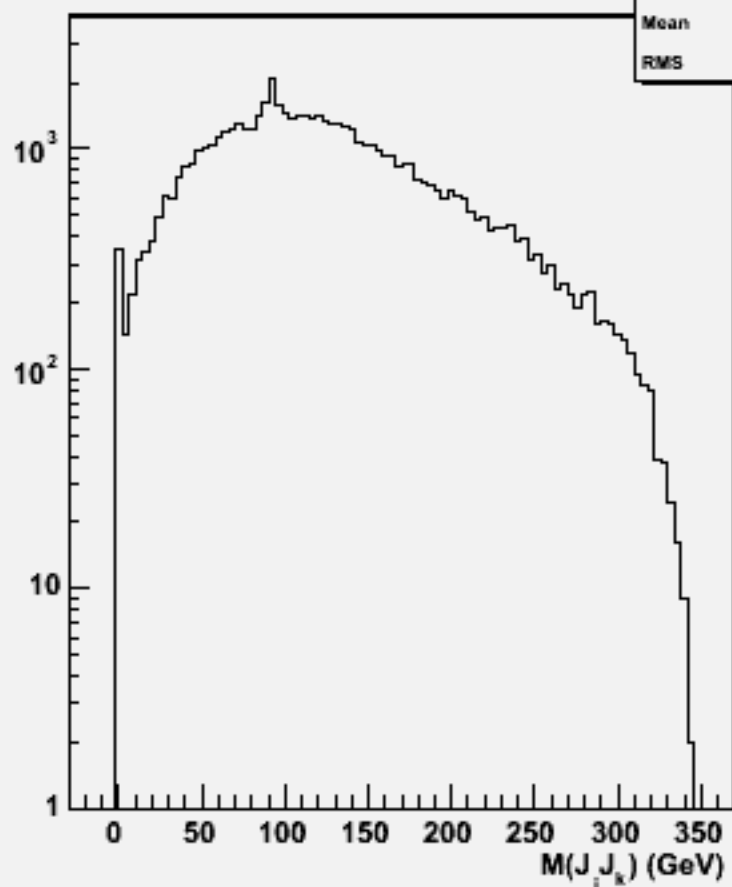
2jets mass(All comb)w103858 ae1_e1ccdd_o
