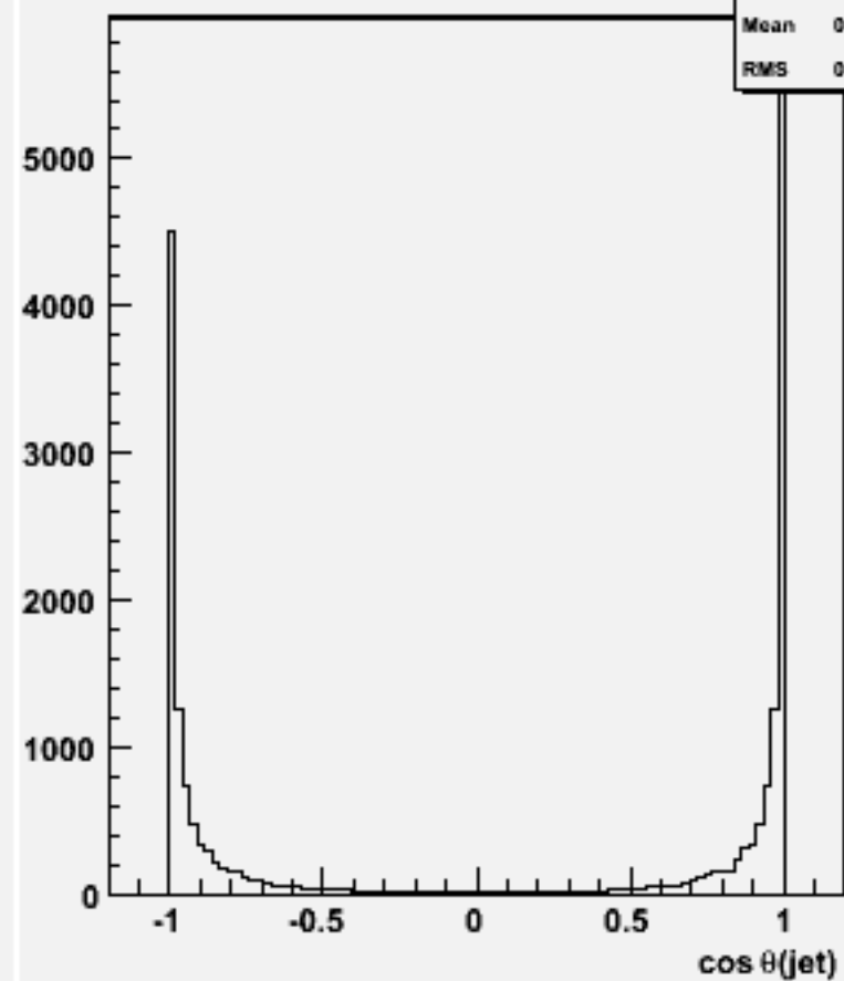
cos \theta for 2-jets :w103858 ae1_e1ccdd_o
