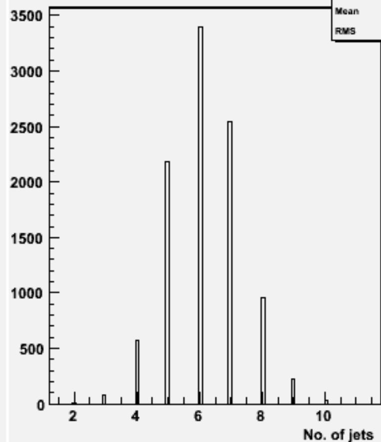
No. jets (ycut=0.001) : w103858 ae1_e1ccdd_o
