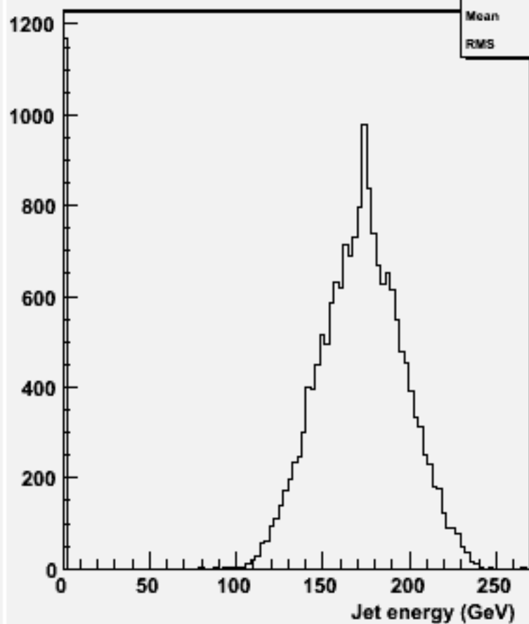
energy for 2-jets :w103858 ae1_e1ccdd_o
