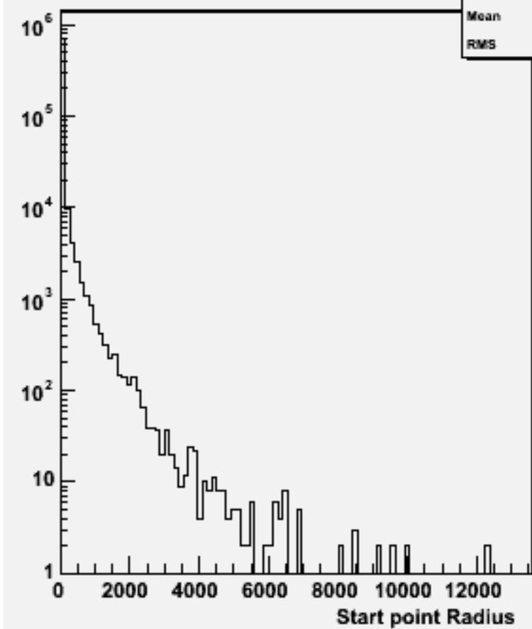
Start point R : w103858 ae1_e1ccdd_o
