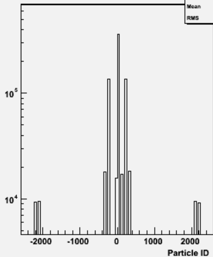
Particle ID : w103858 ae1_e1ccdd_o
