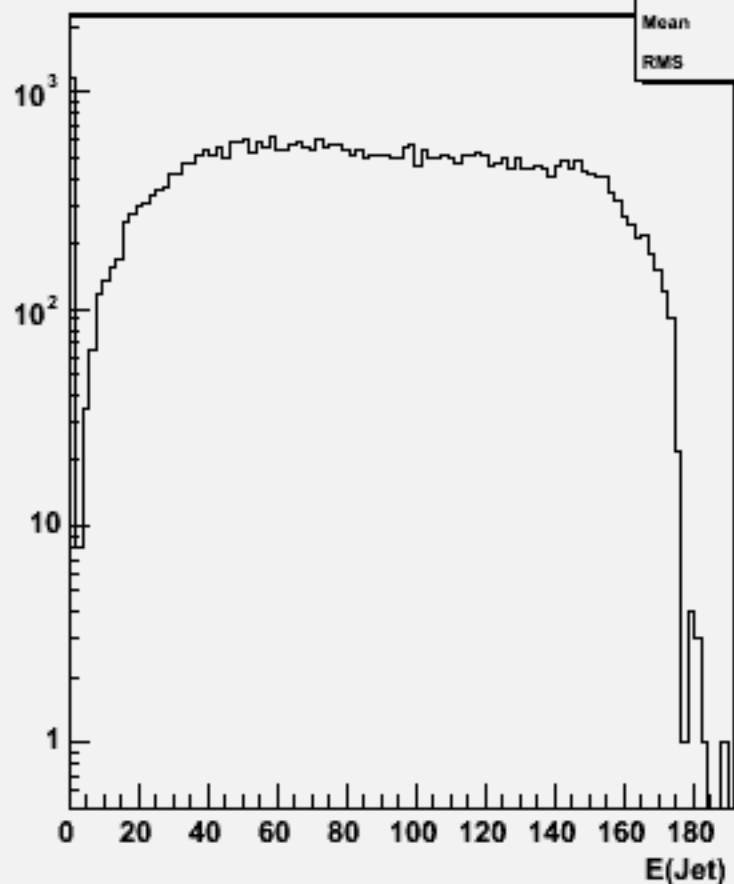
Jet energies(All jets)w103858 ae1_e1ccdd_o
