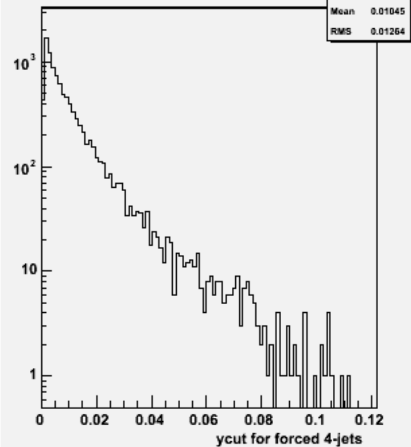
Ycut for 4-jets :w103856 ae1_e1ccdd_o
