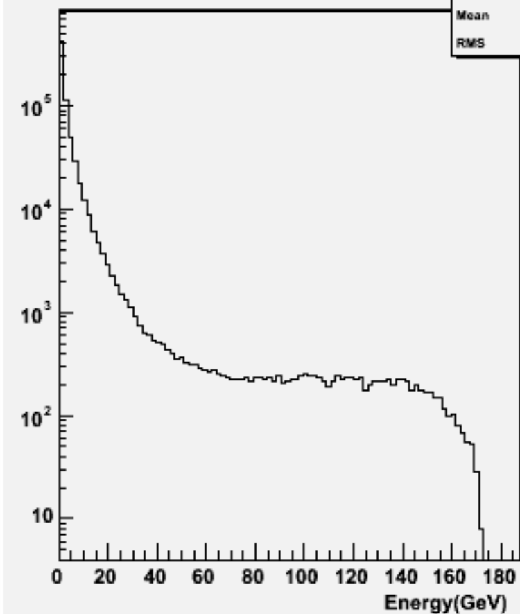
Particle Energy : w103856 ae1_e1ccdd_o
