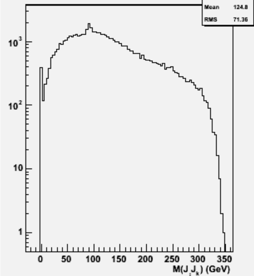
2jets mass(All comb)w103856 ae1_e1ccdd_o
