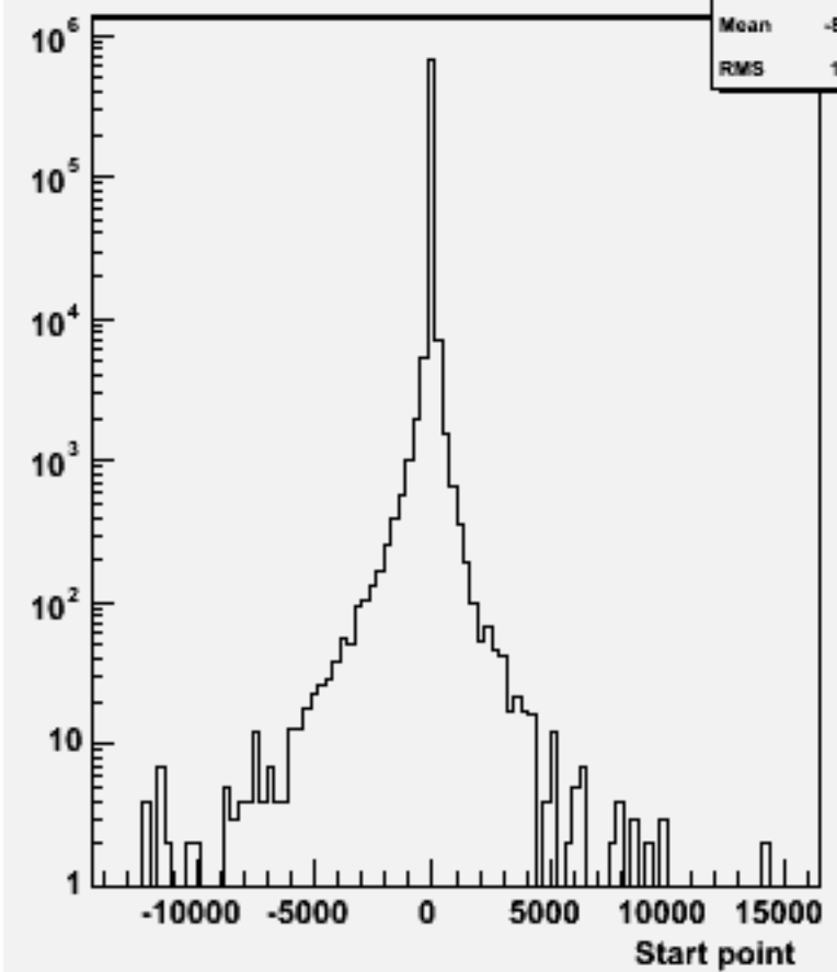
Start point Z : w103856 ae1_e1ccdd_o
