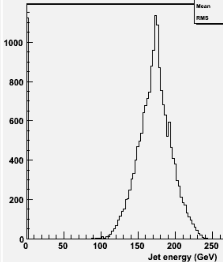
energy for 2-jets :w103856 ae1_e1ccdd_o
