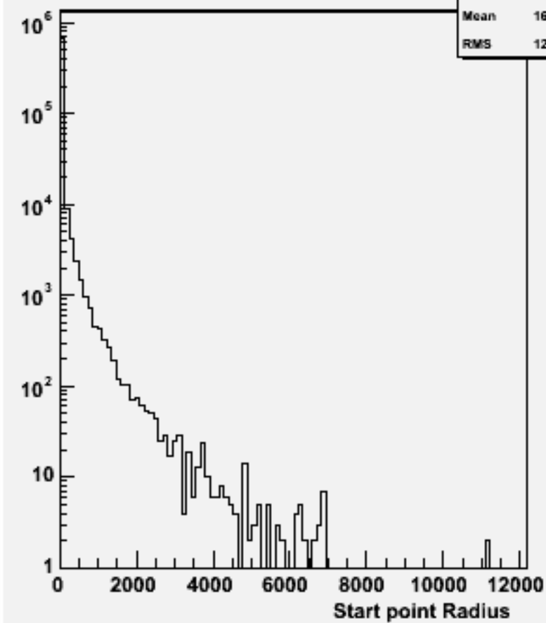
Start point R : w103856 ae1_e1ccdd_o
