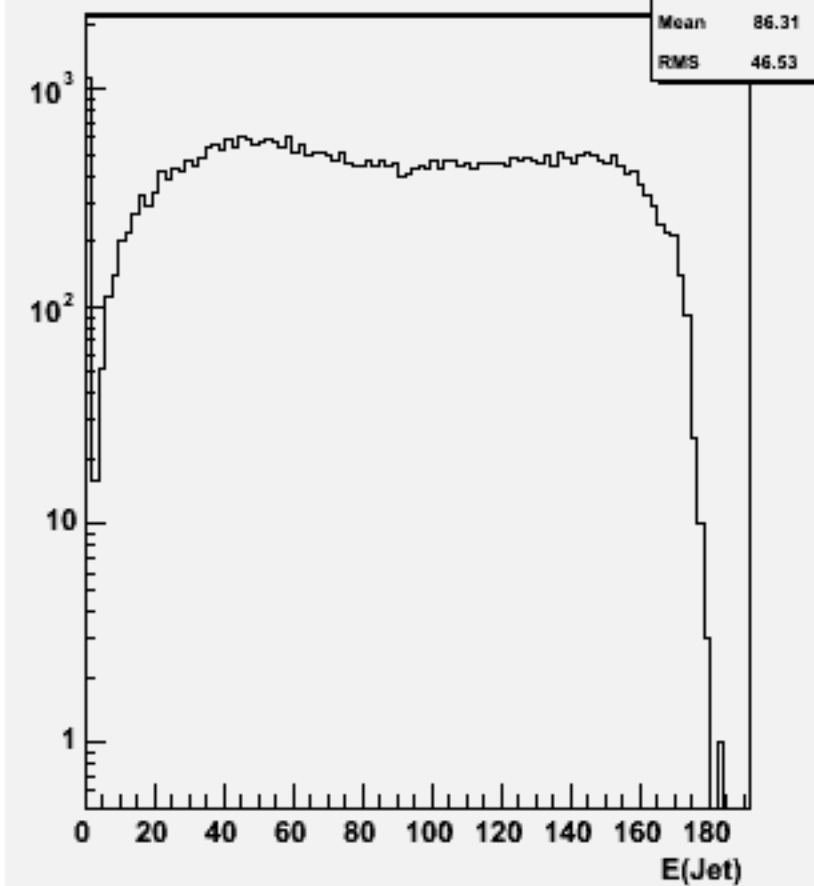
Jet energies(All jets)w103856 ae1_e1ccdd_o
