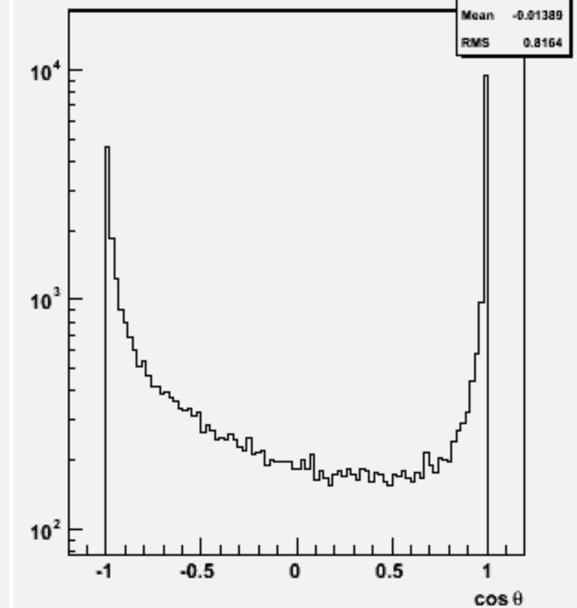
Jet cos \theta (All jets)w103856 ae1_e1ccdd_o
