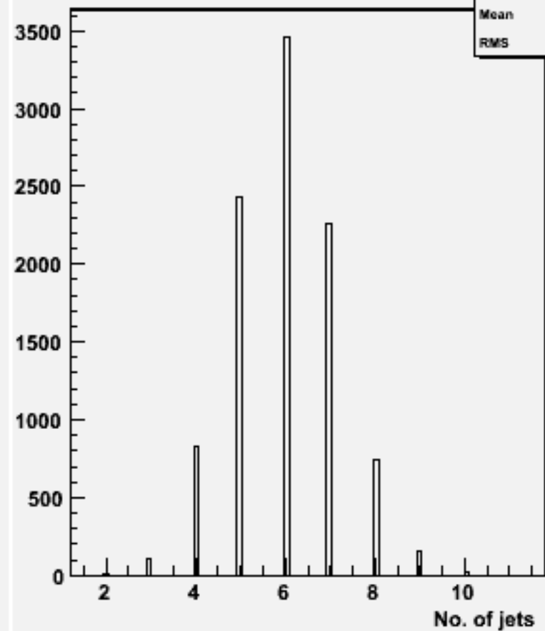
No. jets (ycut=0.001) : w103856 ae1_e1ccdd_o
