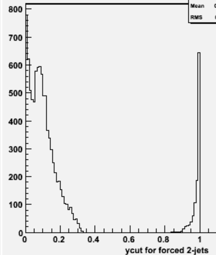
Ycut for 2-jets :w103856 ae1_e1ccdd_o
