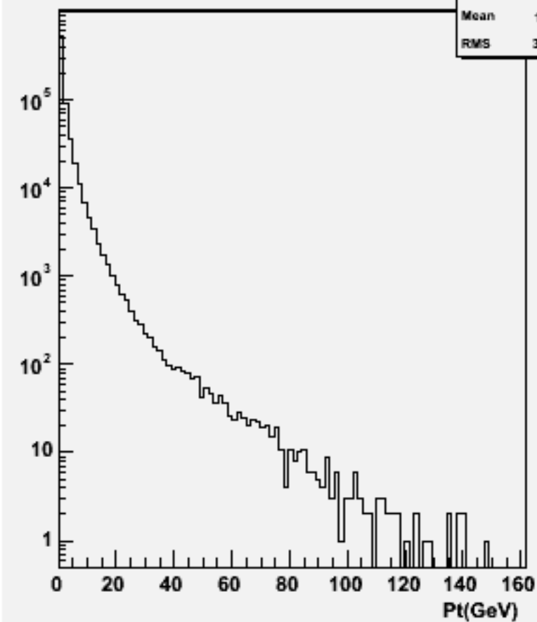
Particle Pt : w103856 ae1_e1ccdd_o
