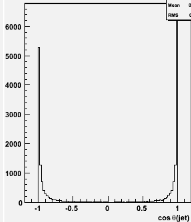
cos \theta for 2-jets :w103856 ae1_e1ccdd_o
