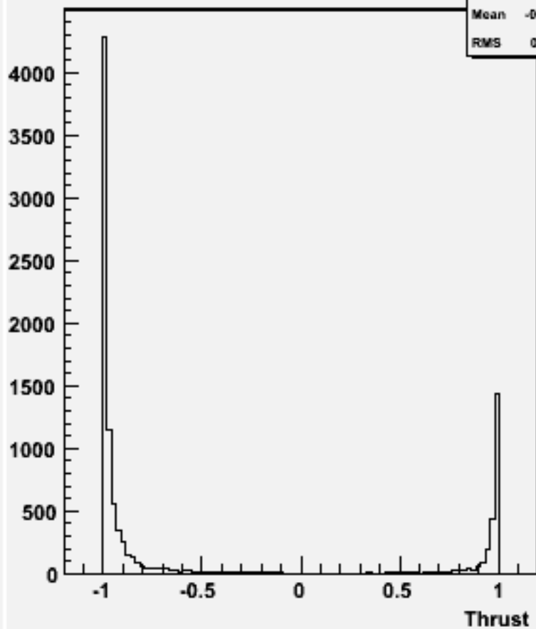
cos \Theta (thrust) w103856 ae1_e1ccdd_o
