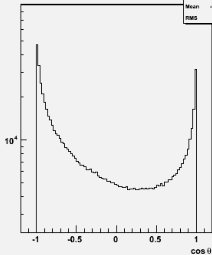
Particle \cos\theta : w103856 ae1_e1ccdd_o
