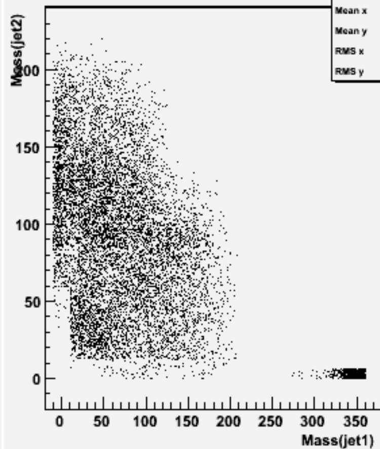
Jet mass for forced 2-jets : w103856 ae1_e1ccdd_o
