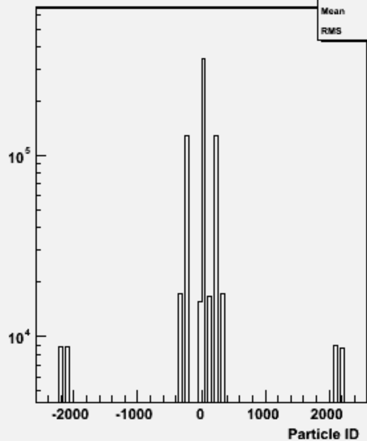
Particle ID : w103856 ae1_e1ccdd_o
