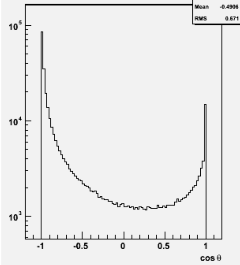
Particle cos θ : w103855 ae1_e1cce3e3_o
