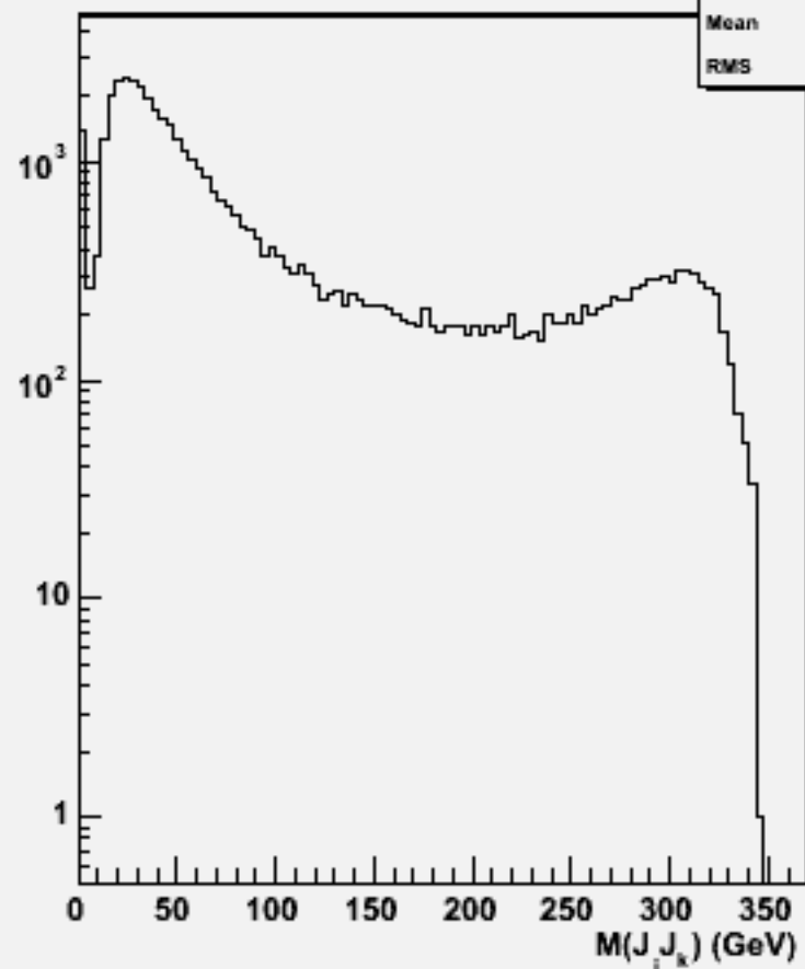
2jets mass(All comb)w103855 ae1_e1cce3e3_o
