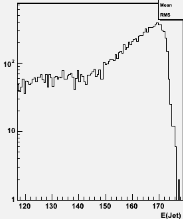
Jet energies(All jets)w103855 ae1_e1cce3e3_o
