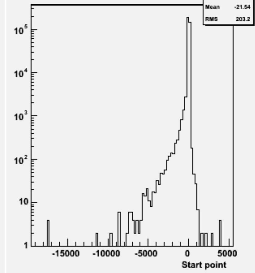
Start point Z : w103855 ae1_e1cce3e3_o
