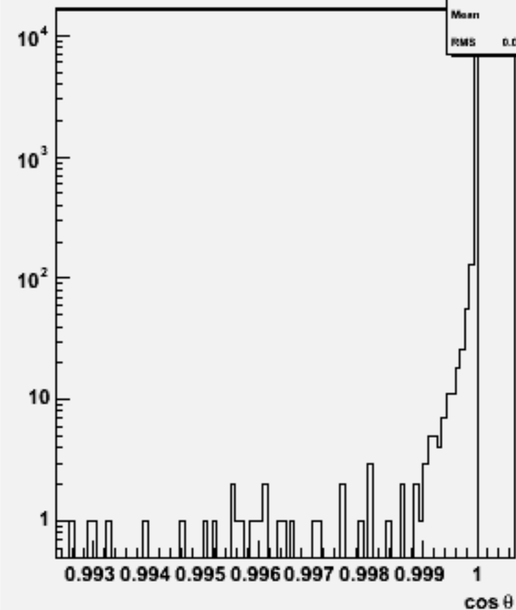
Jet cos \theta (All jets)w103855 ae1_e1cce3e3_o
