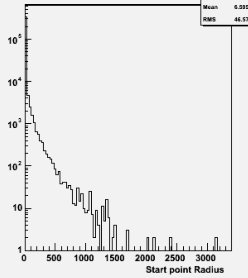
Start point R : w103855 ae1_e1cce3e3_o
