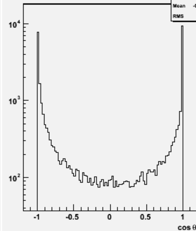
Jet cos \theta (All jets)w103854 ae1_e1cce3e3_o
