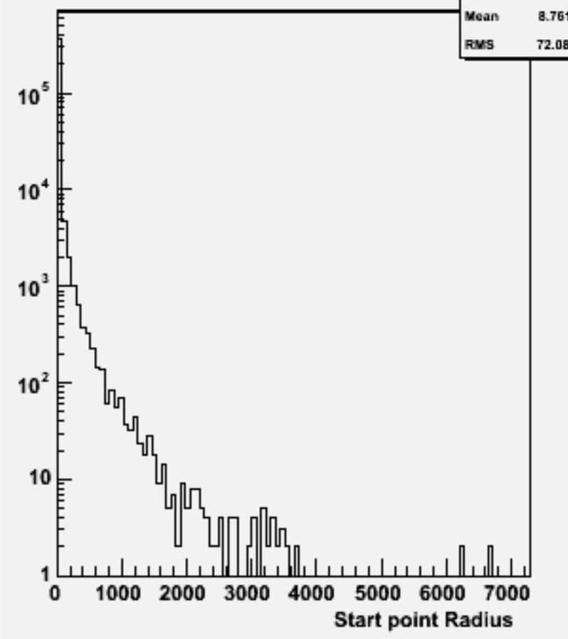
Start point R : w103854 ae1_e1cce3e3_o
