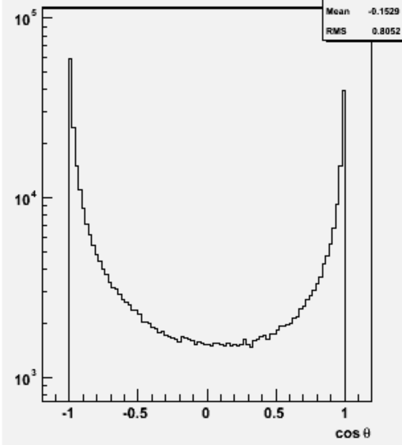
Particle cos \theta : w103854 ae1_e1cce3e3_o
