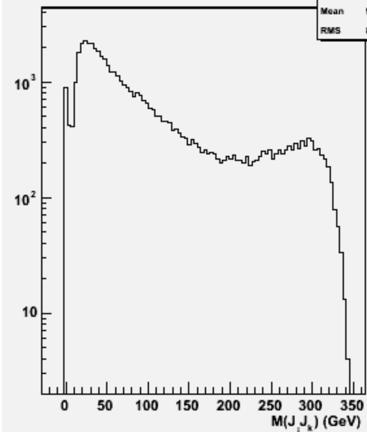
2jets mass(All comb)w103854 ae1_e1cce3e3_o
