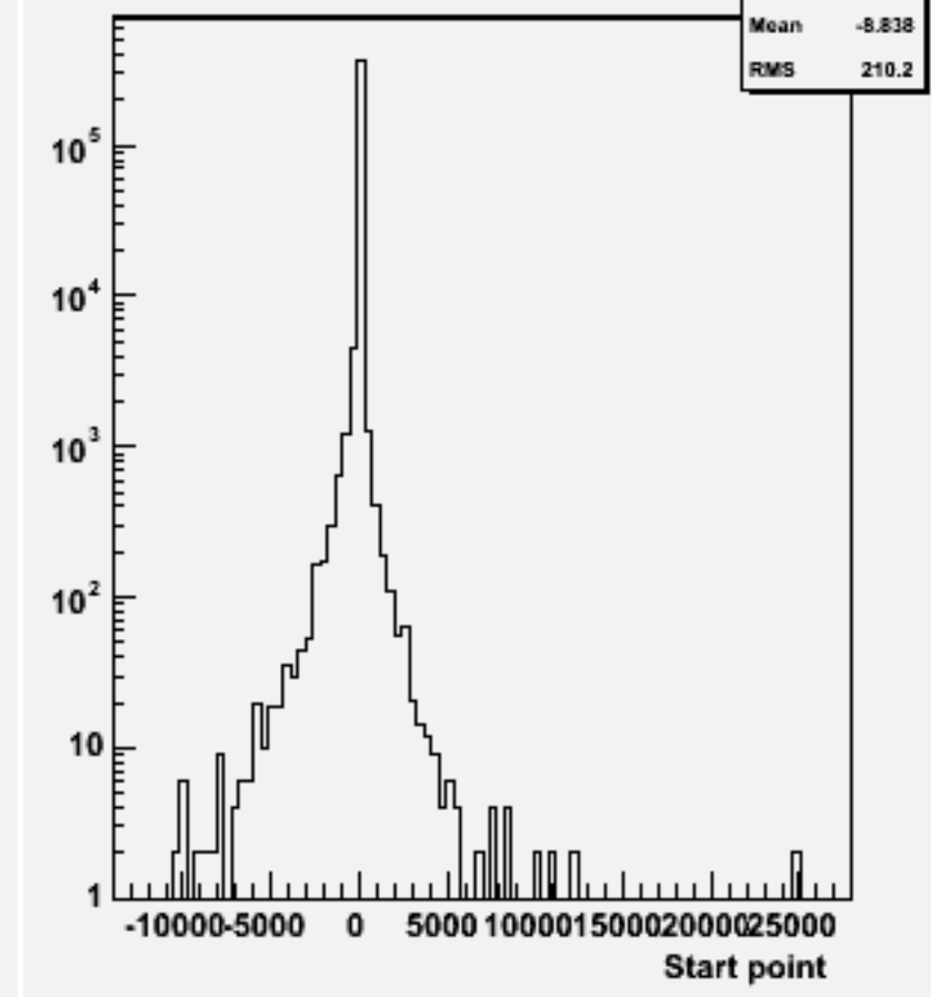
Start point Z : w103854 ae1_e1cce3e3_o
