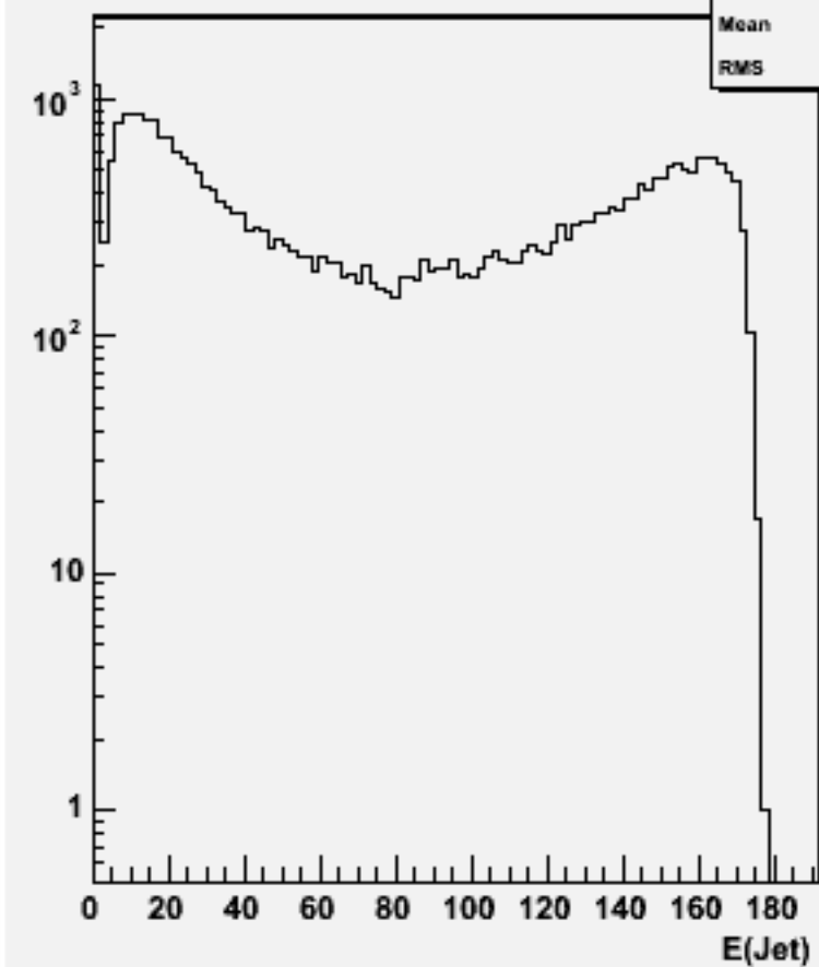
Jet energies(All jets)w103854 ae1_e1cce3e3_o
