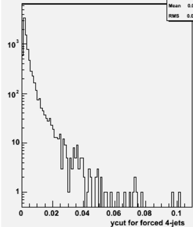
Ycut for 4-jets :w103854 ae1_e1cce3e3_o
