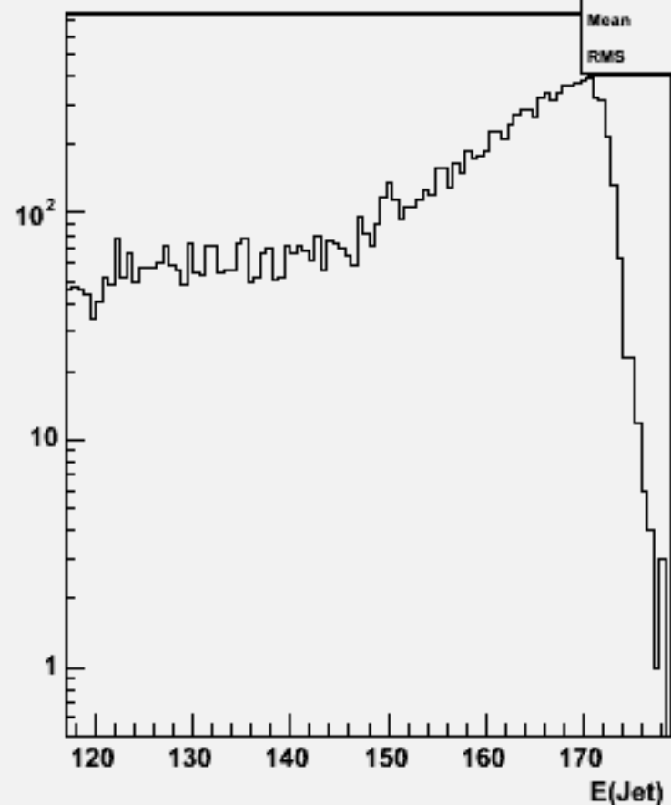
Jet energies(All jets)w103853 ae1_e1cce3e3_o
