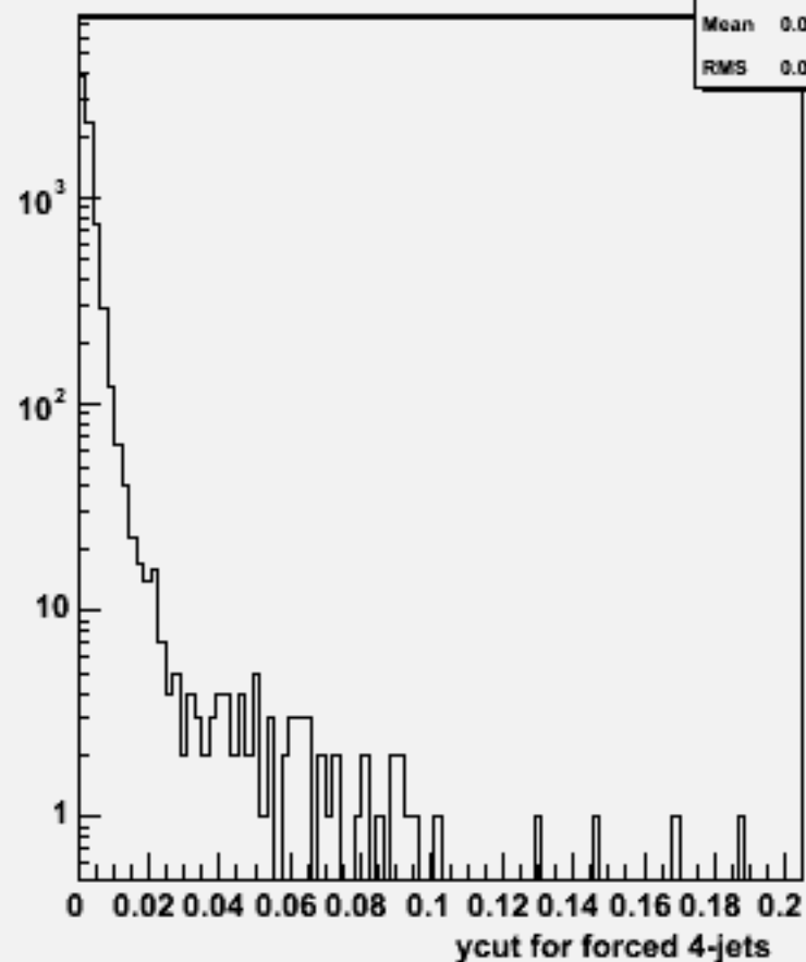
Ycut for 4-jets :w103853 ae1_e1cce3e3_o
