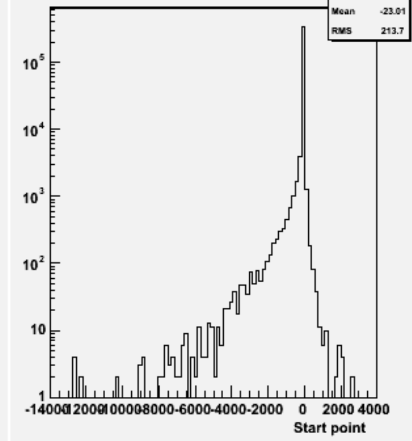
Start point Z : w103853 ae1_e1cce3e3_o
