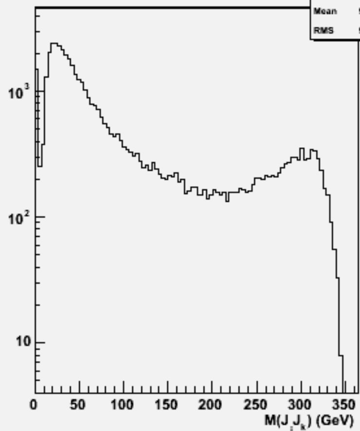
2jets mass(All comb)w103853 ae1_e1cce3e3_o
