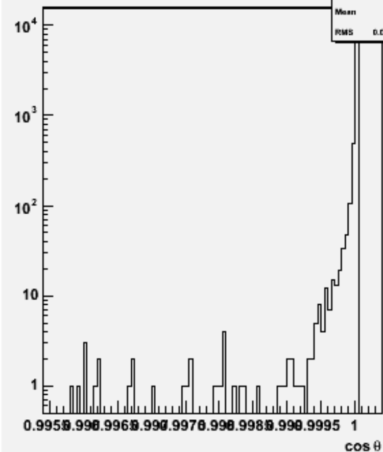
Jet cos \theta (All jets)w103853 ae1_e1cce3e3_o
