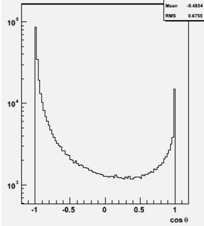
Particle cos \theta : w103853 ae1_e1cce3e3_o
