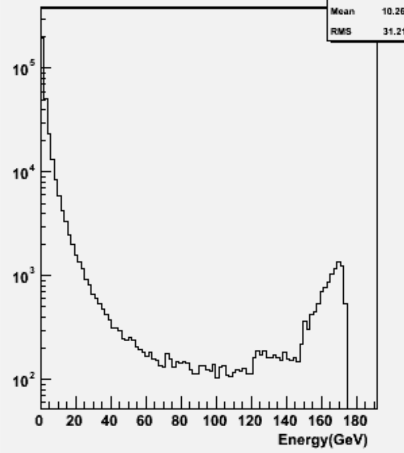
Start point R : w103853 ae1_e1cce3e3_o
