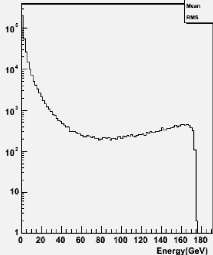
Start point R : w103852 ae1_e1cce3e3_o
