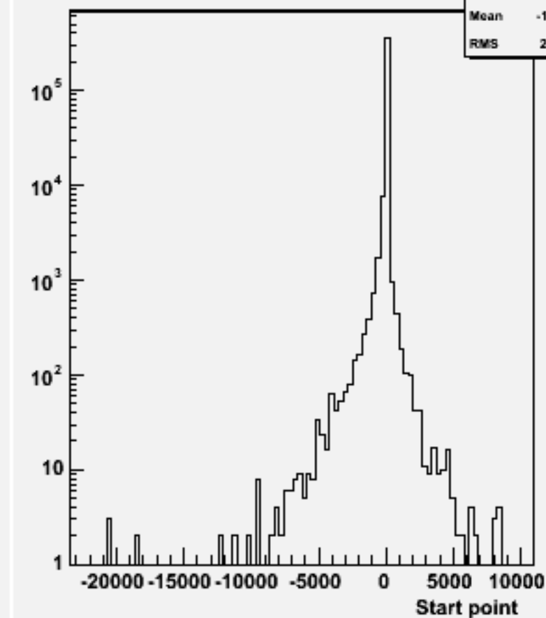
Start point Z : w103852 ae1_e1cce3e3_o
