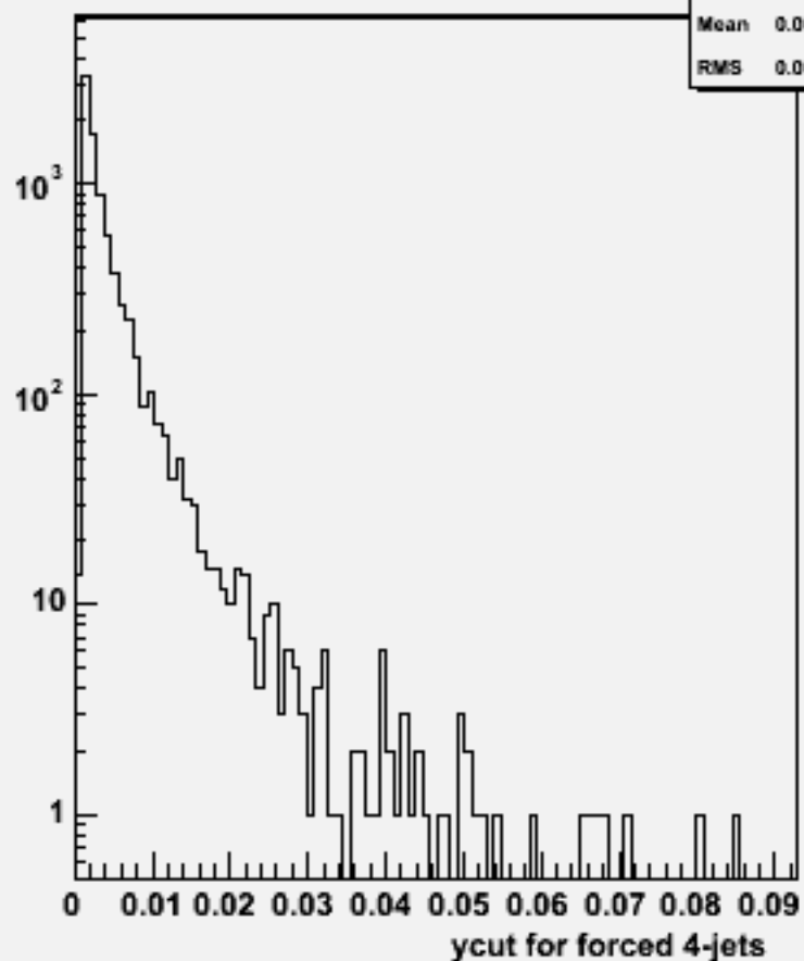
Ycut for 4-jets :w103852 ae1_e1cce3e3_o
