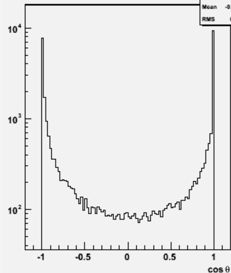
Jet cos \theta (All jets)w103852 ae1_e1cce3e3_o
