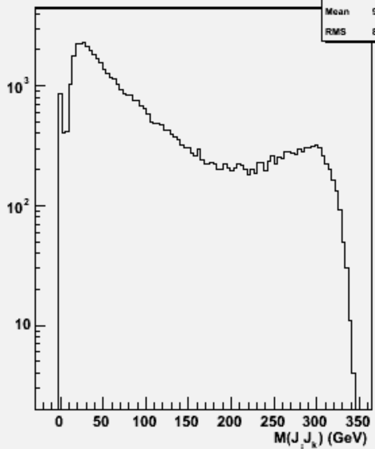
2jets mass(All comb)w103852 ae1_e1cce3e3_o
