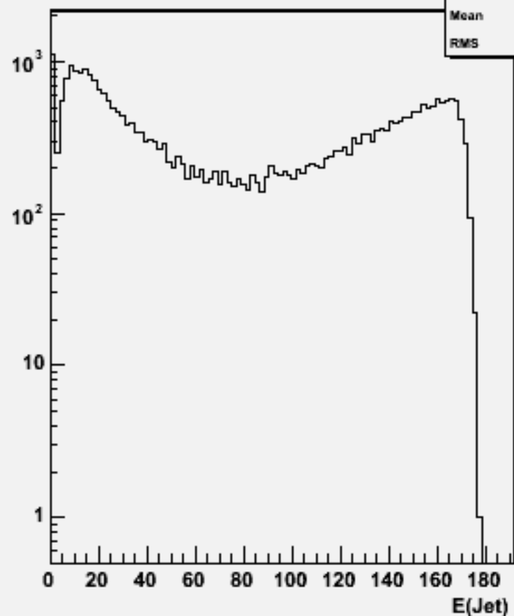
Jet energies(All jets)w103852 ae1_e1cce3e3_o
