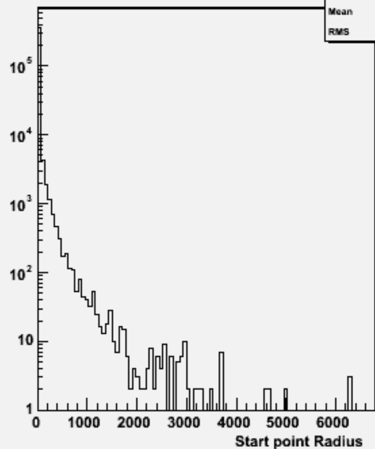
Start point R : w103852 ae1_e1cce3e3_o
