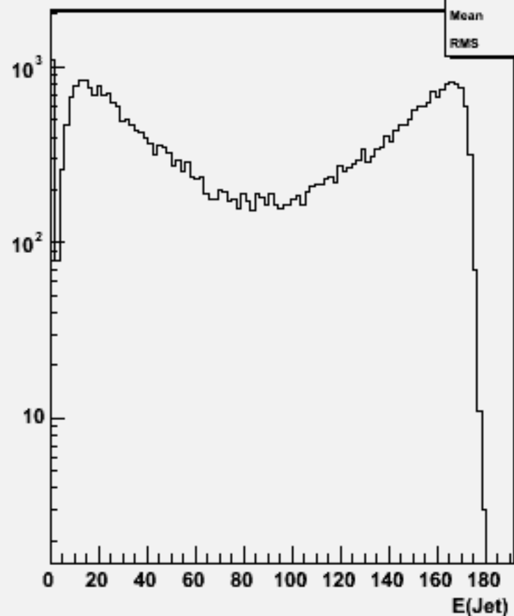
Jet energies(All jets)w103850 ae1_e1cce2e2_o
