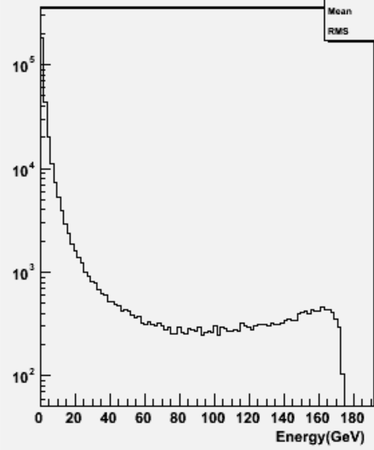
Start point R : w103850 ae1_e1cce2e2_o
