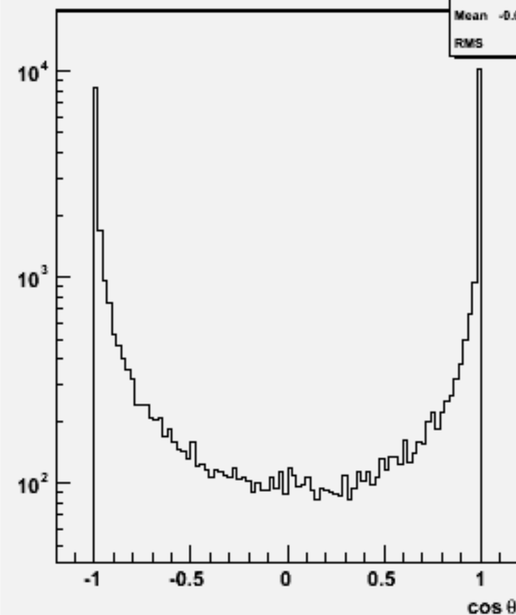
Jet cos \theta (All jets)w103850 ae1_e1cce2e2_o
