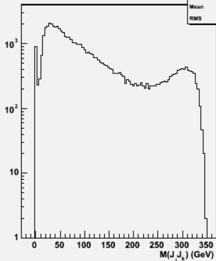
2jets mass(All comb)w103850 ae1_e1cce2e2_o
