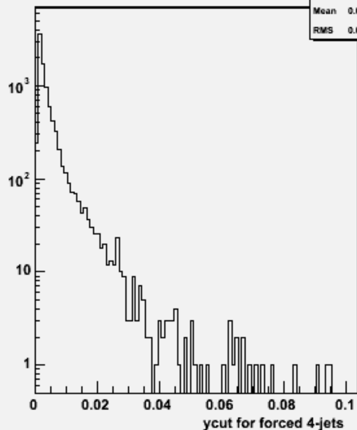
Ycut for 4-jets :w103850 ae1_e1cce2e2_o
