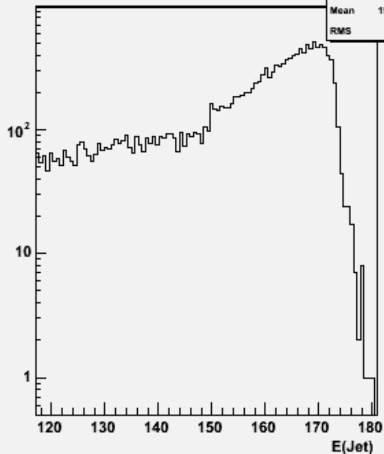
Jet energies(All jets)w103849 ae1_e1cce2e2_o
