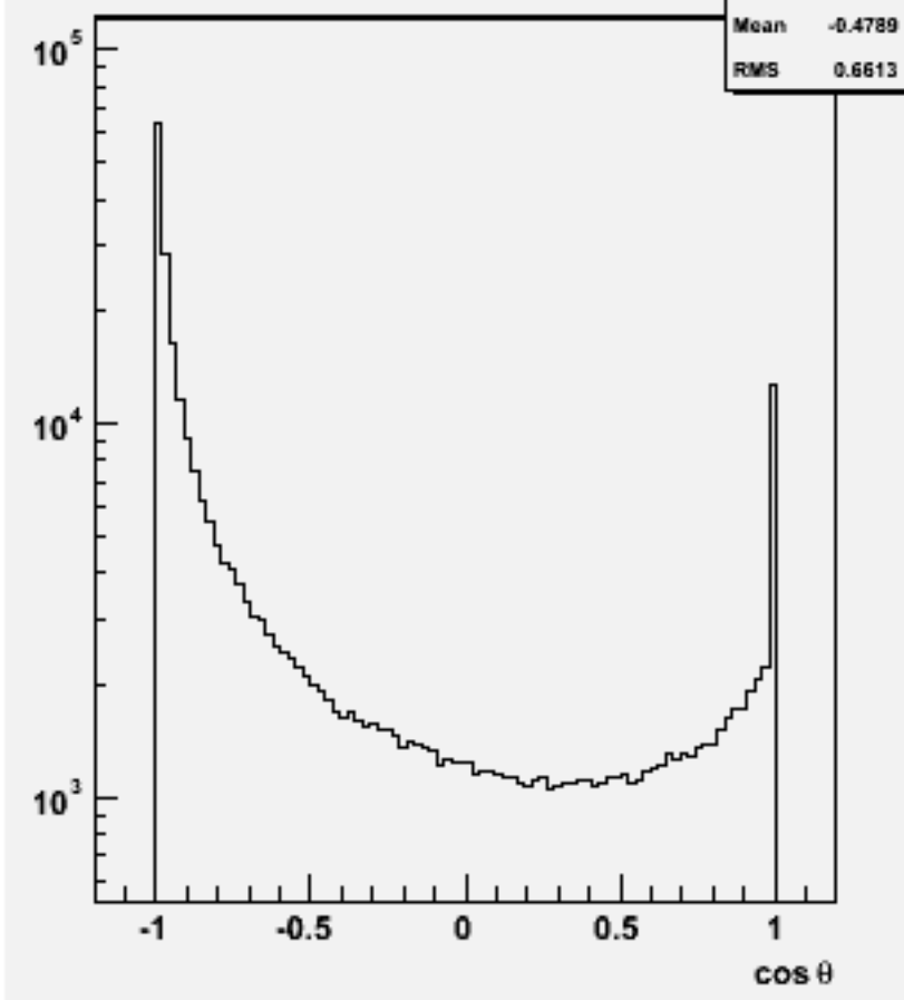
Particle cos \theta : w103849 ae1_e1cce2e2_o
