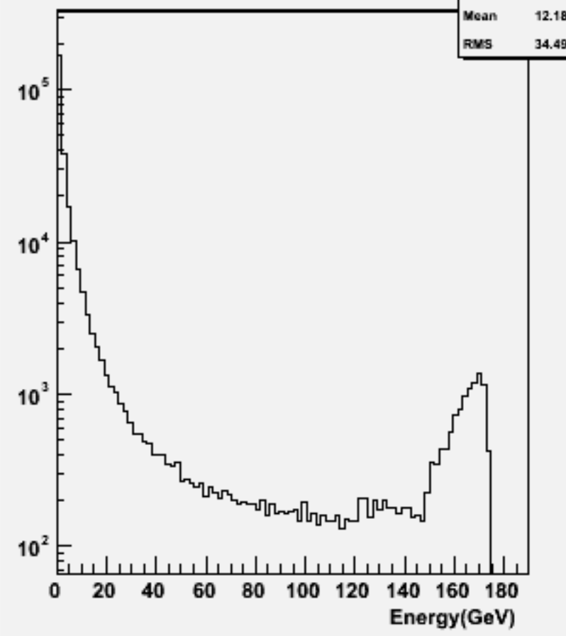
Start point R : w103849 ae1_e1cce2e2_o
