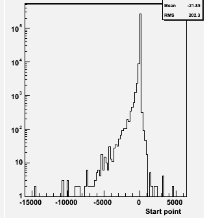
Start point Z : w103849 ae1_e1cce2e2_o
