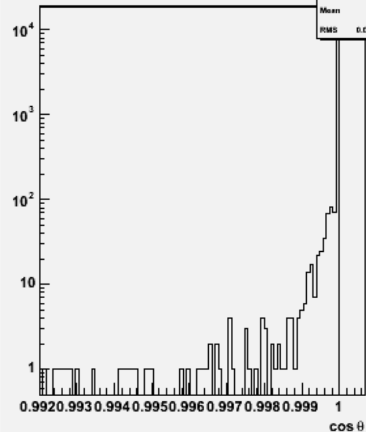
Jet cos \theta (All jets)w103849 ae1_e1cce2e2_o
