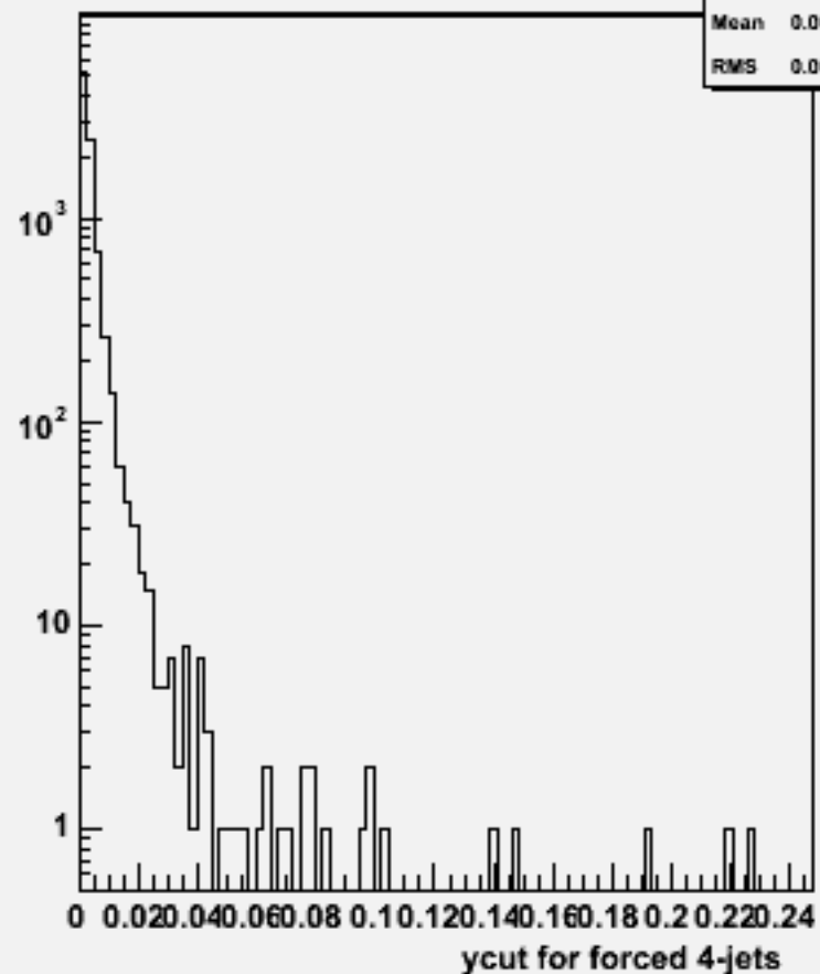
Ycut for 4-jets :w103849 ae1_e1cce2e2_o
