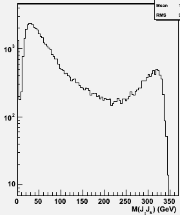
2jets mass(All comb)w103849 ae1_e1cce2e2_o
