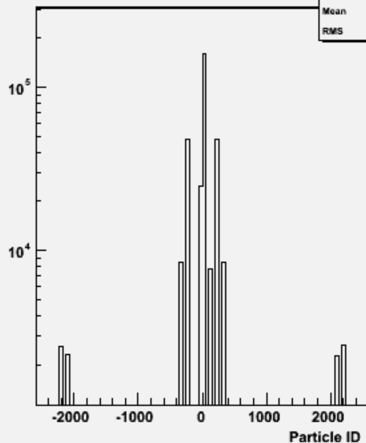
Particle ID : w103848 ae1_e1cce2e2_o
