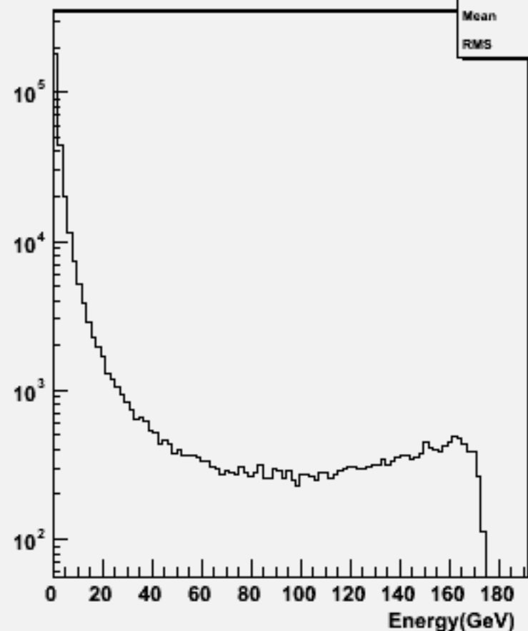
Particle Energy : w103848 ae1_e1cce2e2_o
