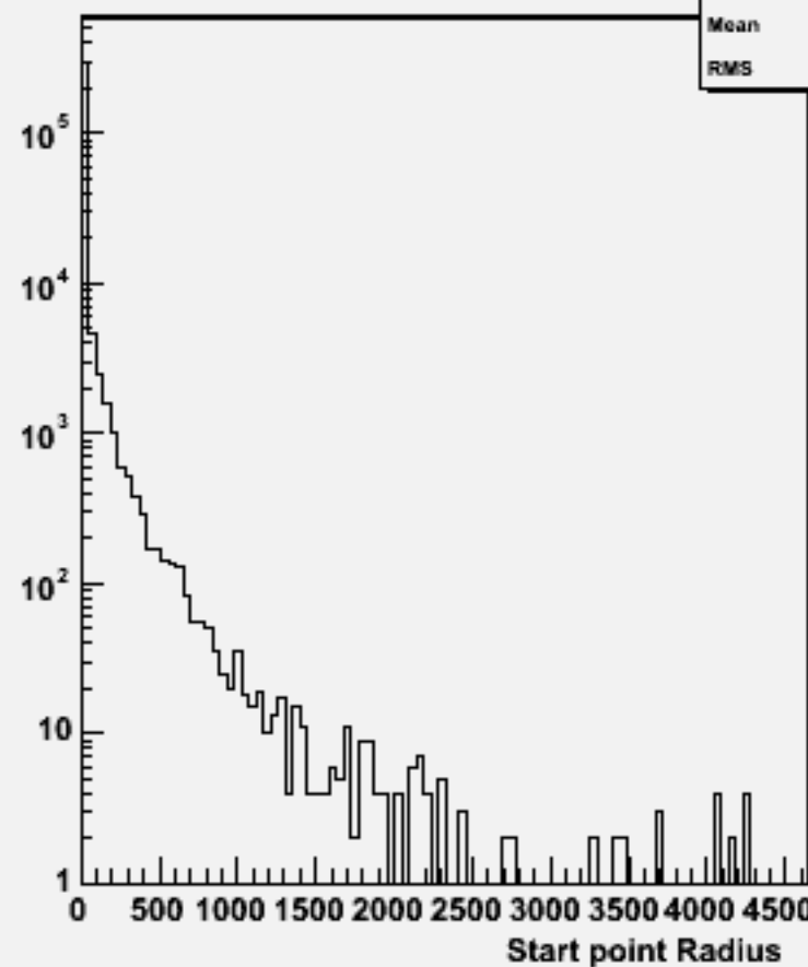
Start point R : w103848 ae1_e1cce2e2_o
