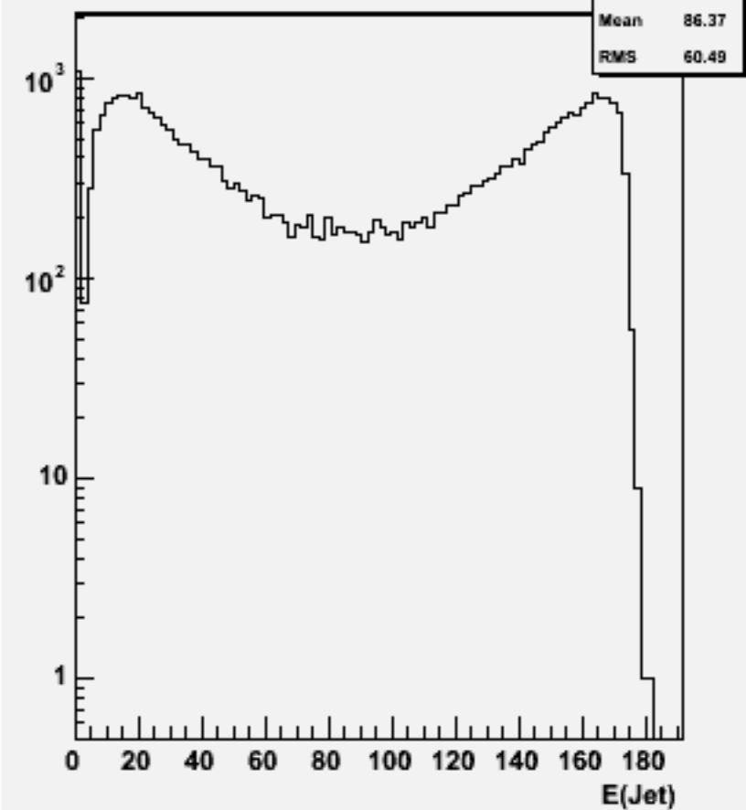
Jet energies(All jets)w103848 ae1_e1cce2e2_o
