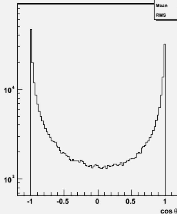
Particle cos \theta : w103848 ae1_e1cce2e2_o
