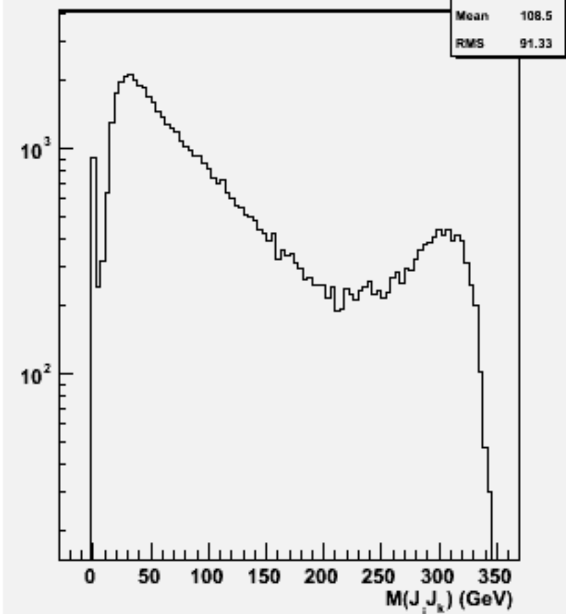
2jets mass(All comb)w103848 ae1_e1cce2e2_o
