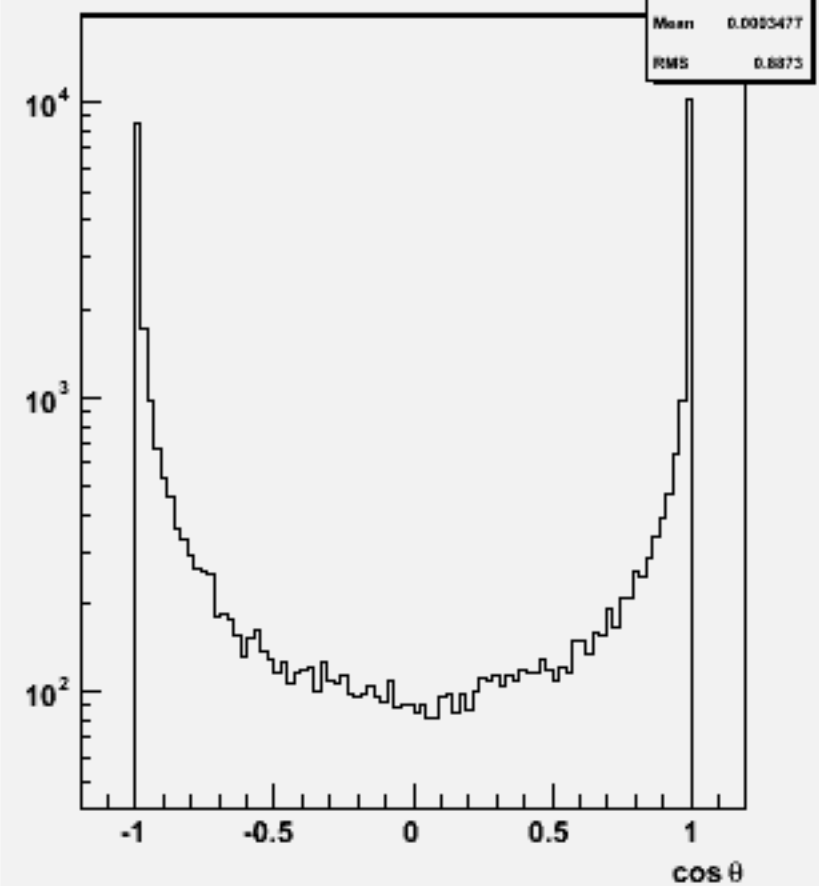
Jet cos \theta (All jets)w103848 ae1_e1cce2e2_o
