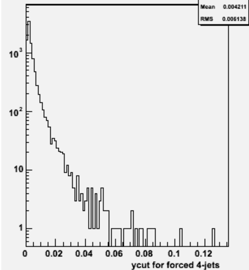
Ycut for 4-jets :w103848 ae1_e1cce2e2_o
