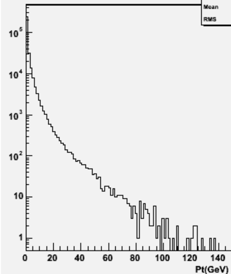
Particle Pt : w103848 ae1_e1cce2e2_o
