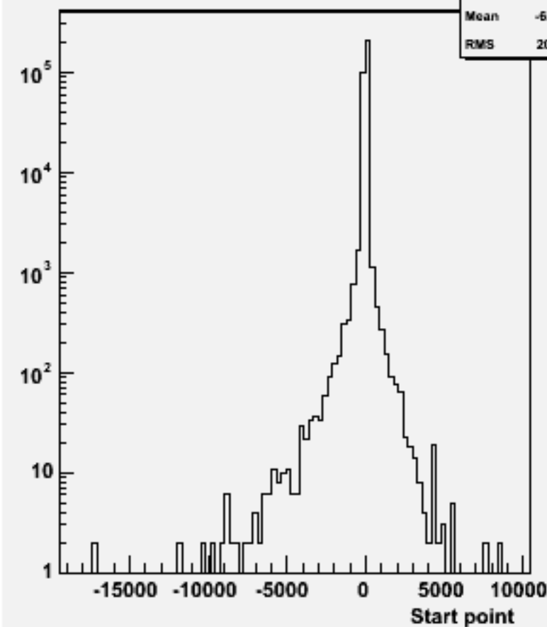
Start point Z : w103848 ae1_e1cce2e2_o
