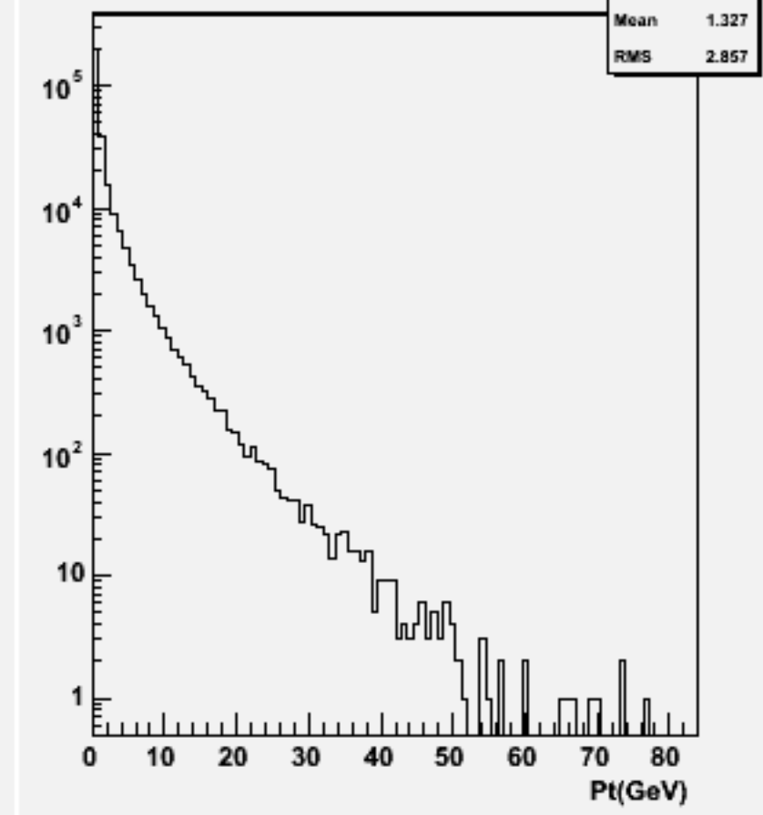
Start point Z : w103847 ae1_e1cce1e1_o
