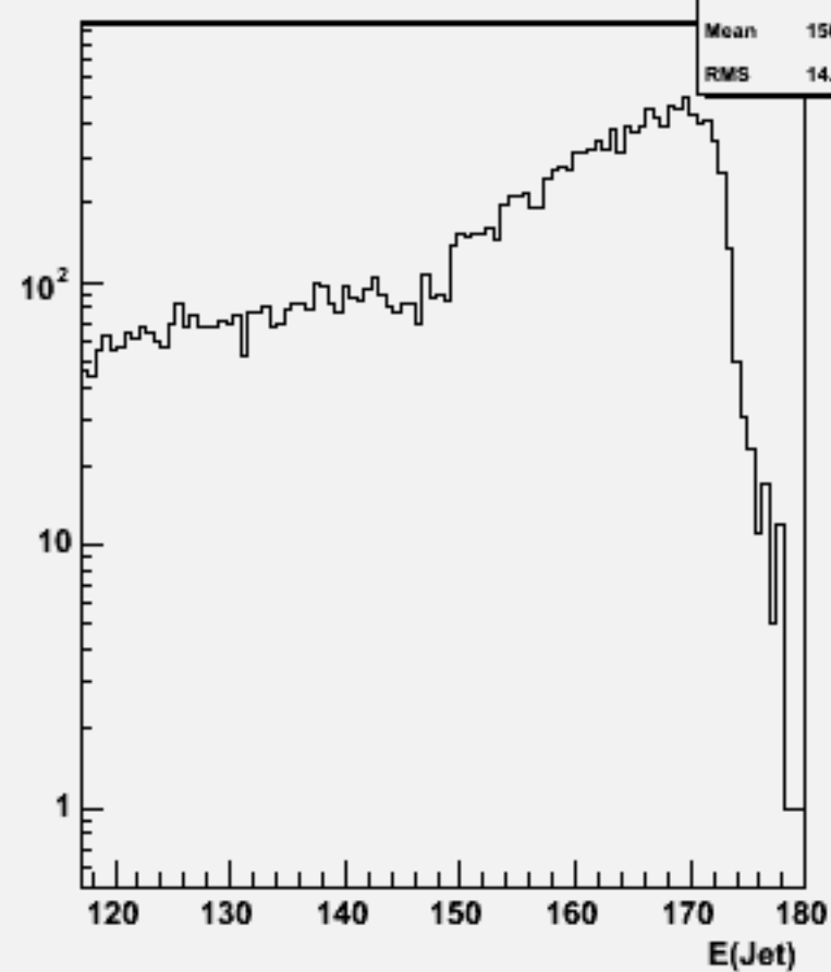
Jet energies(All jets)w103847 ae1_e1cce1e1_o
