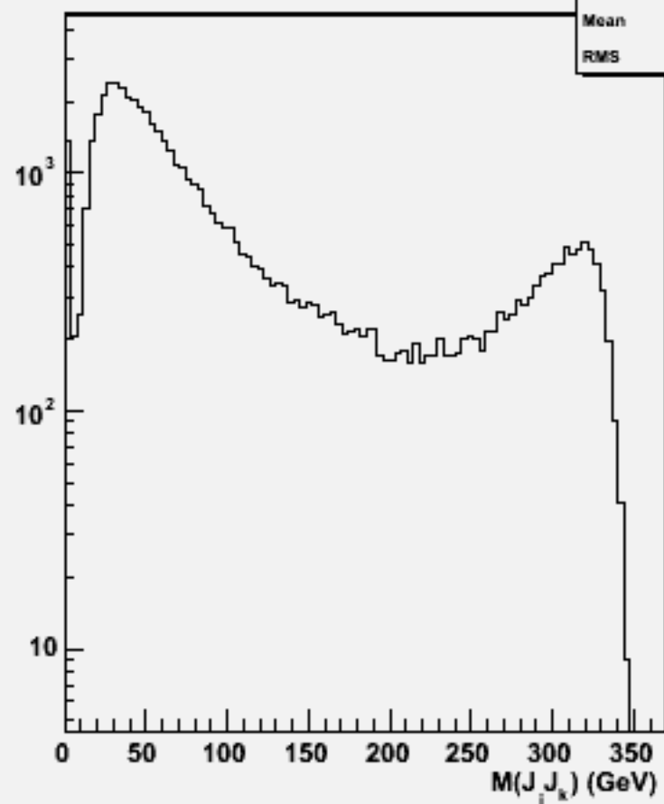
2jets mass(All comb)w103847 ae1_e1cce1e1_o
