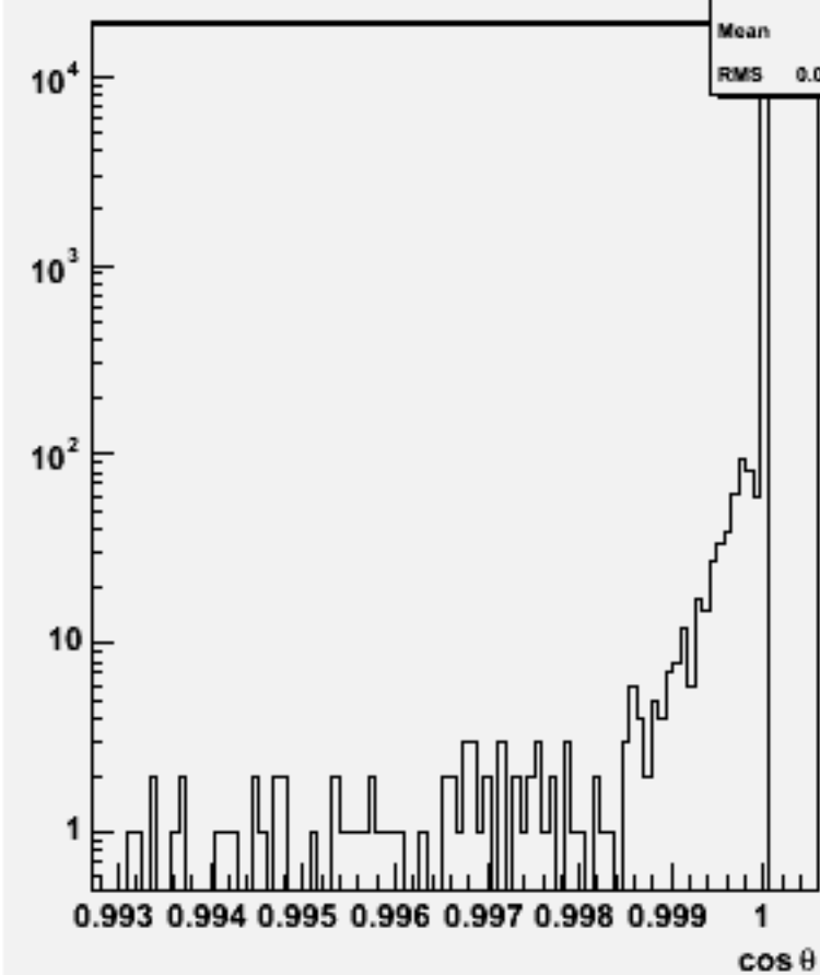
Jet cos \theta (All jets)w103847 ae1_e1cce1e1_o
