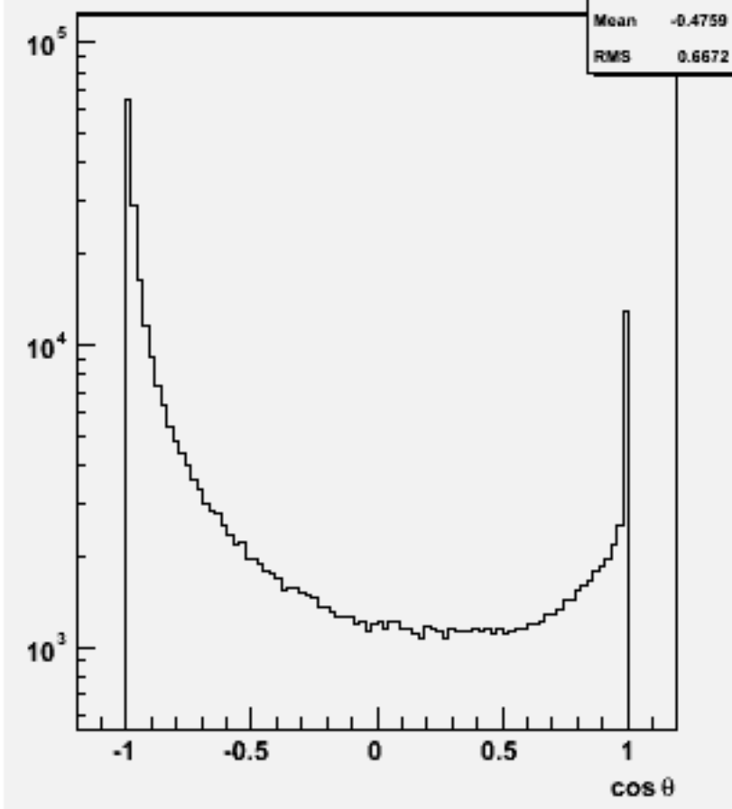
Particle cos \theta : w103847 ae1_e1cce1e1_o
