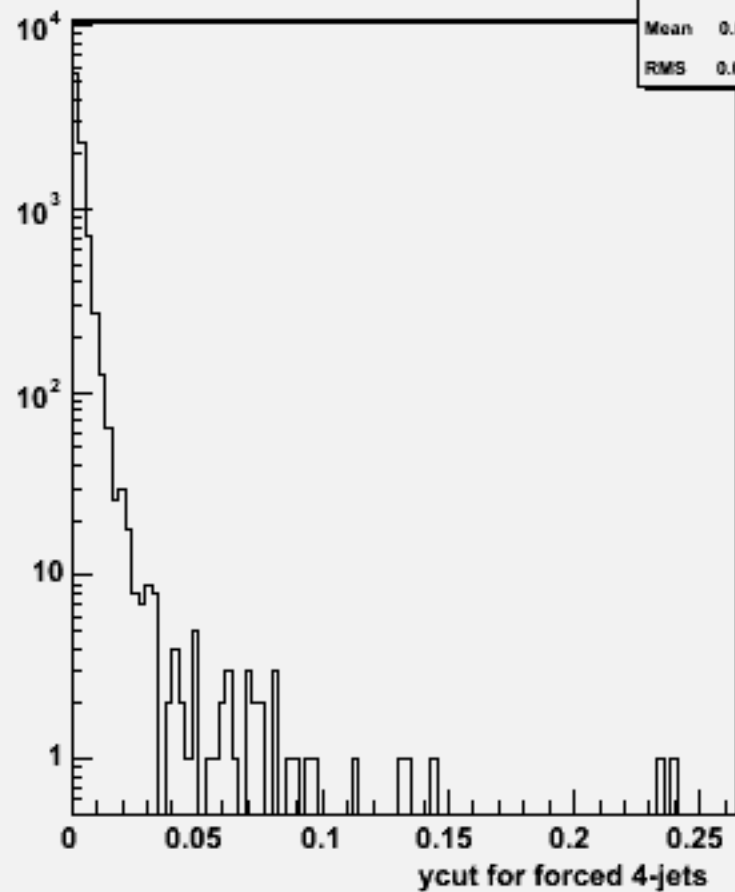
Ycut for 4-jets :w103847 ae1_e1cce1e1_o
