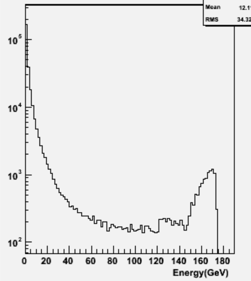
Start point R : w103847 ae1_e1cce1e1_o
