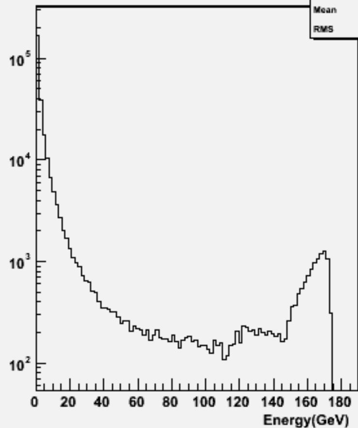
Start point R : w103845 ae1_e1cce1e1_o
