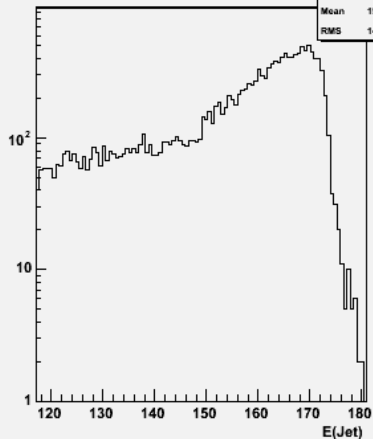
Jet energies(All jets)w103845 ae1_e1cce1e1_o
