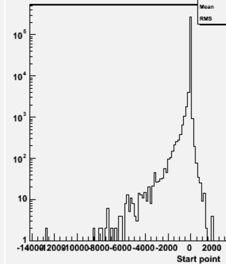
Start point Z : w103845 ae1_e1cce1e1_o
