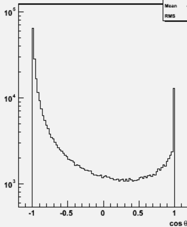
Particle cos \theta : w103845 ae1_e1cce1e1_o
