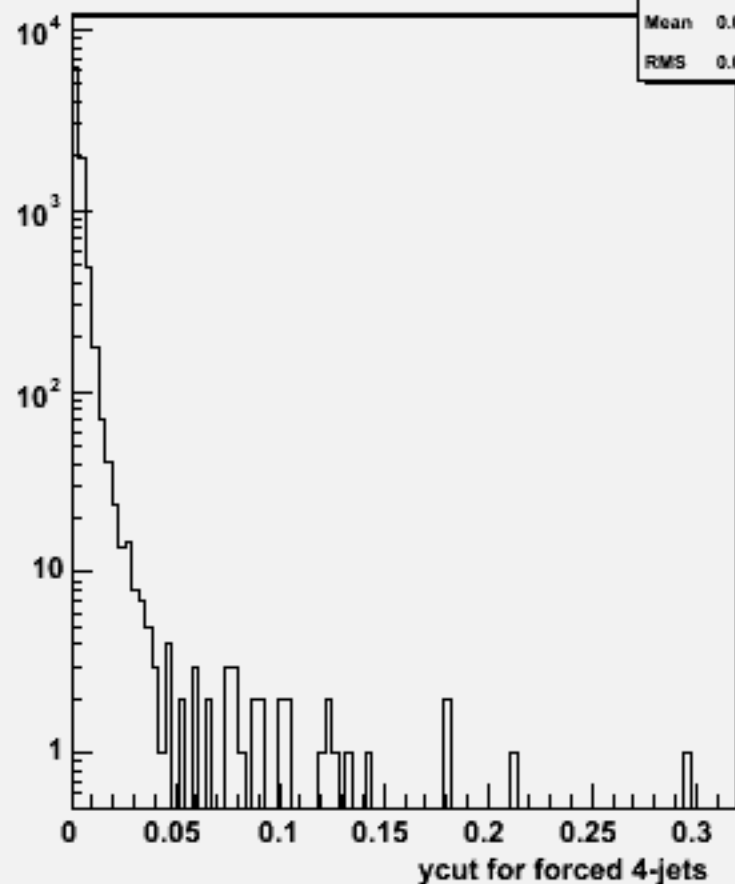
Ycut for 4-jets :w103845 ae1_e1cce1e1_o
