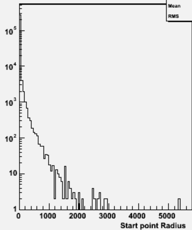
Start point R : w103845 ae1_e1cce1e1_o
