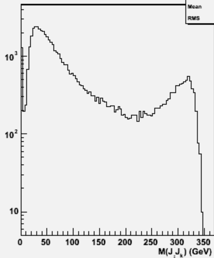
2jets mass(All comb)w103845 ae1_e1cce1e1_o
