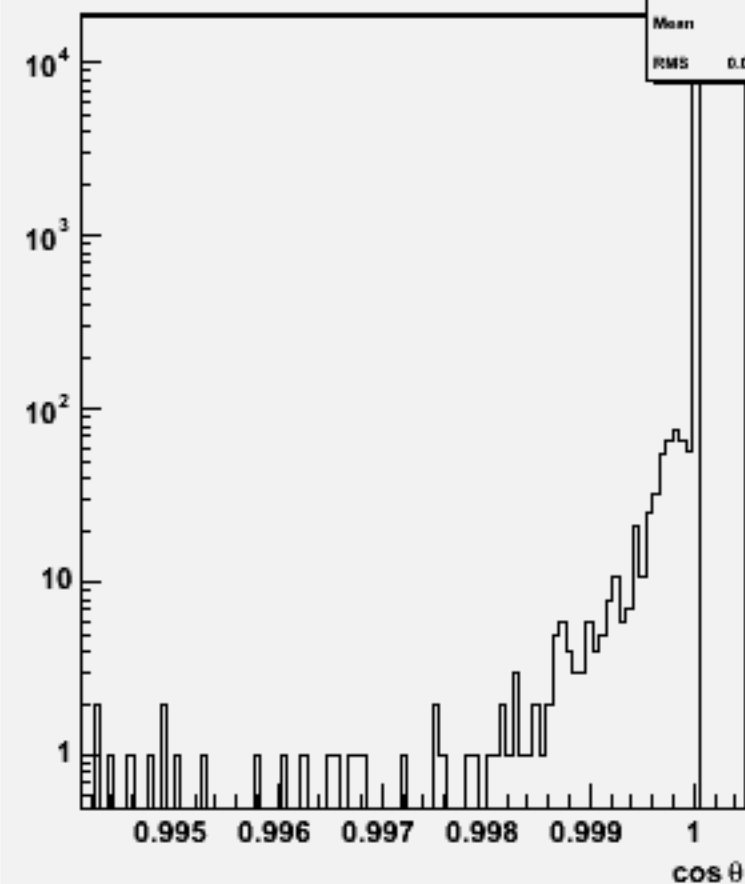
Jet cos \theta (All jets)w103845 ae1_e1cce1e1_o
