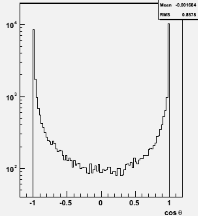
Jet cos theta (All jets)w103844 ae1_e1cce1e1_o
