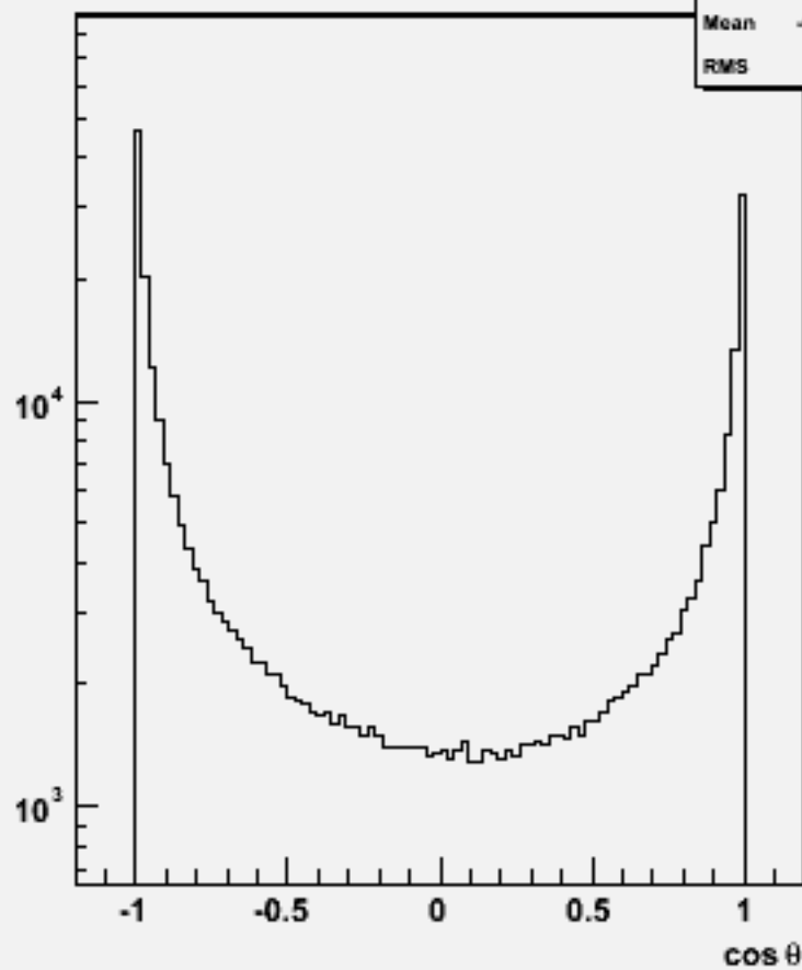
Particle cos \theta : w103844 ae1_e1cce1e1_o
