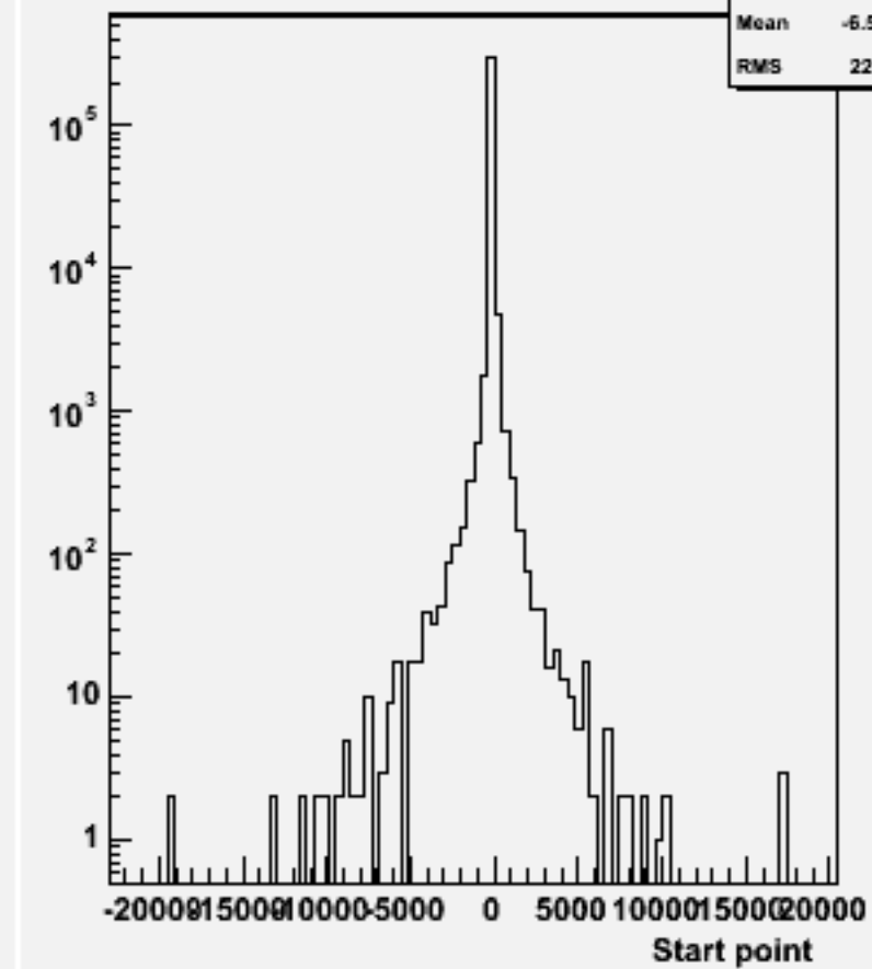
Start point Z : w103844 ae1_e1cce1e1_o
