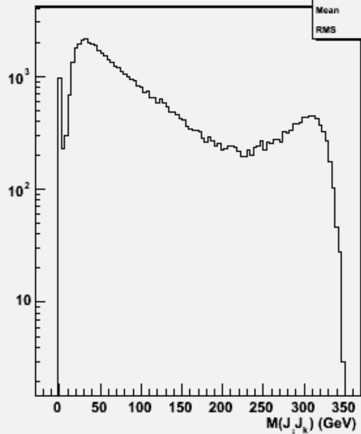
2jets mass(All comb)w103844 ae1_e1cce1e1_o
