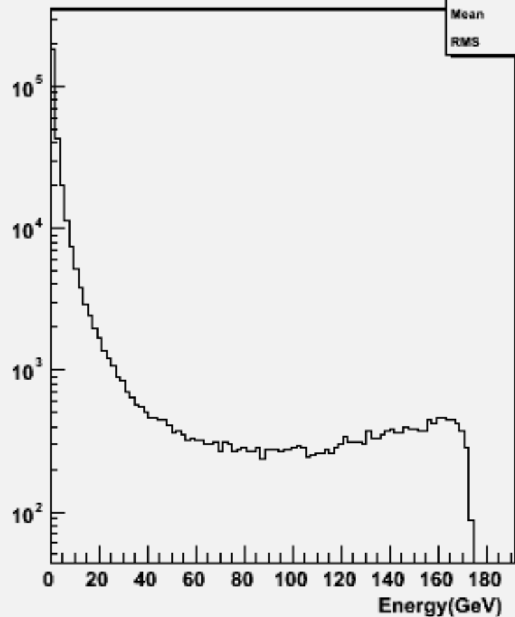
Start point R : w103844 ae1_e1cce1e1_o
