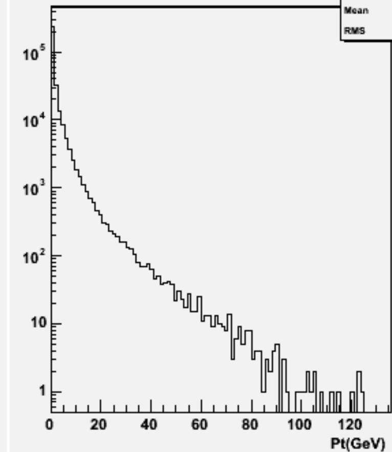
Start point Z : w103844 ae1_e1cce1e1_o
