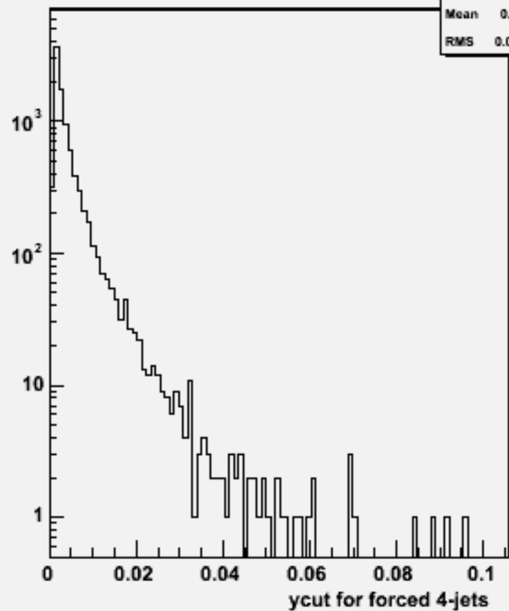
Ycut for 4-jets :w103844 ae1_e1cce1e1_o
