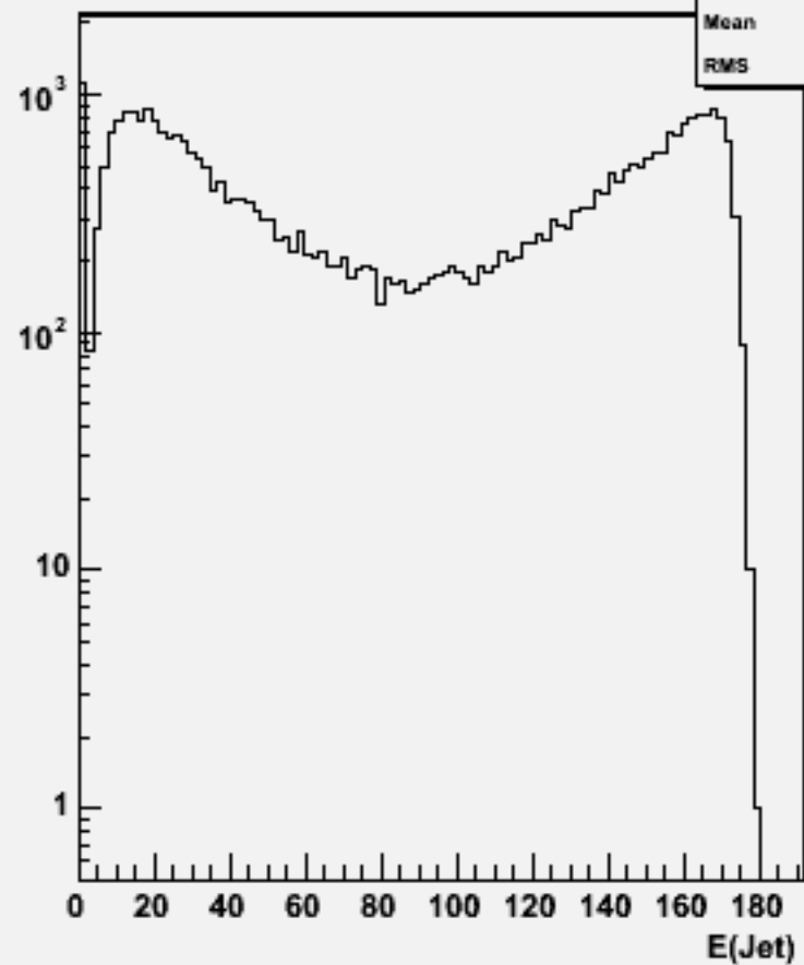
Jet energies(All jets)w103844 ae1_e1cce1e1_o
