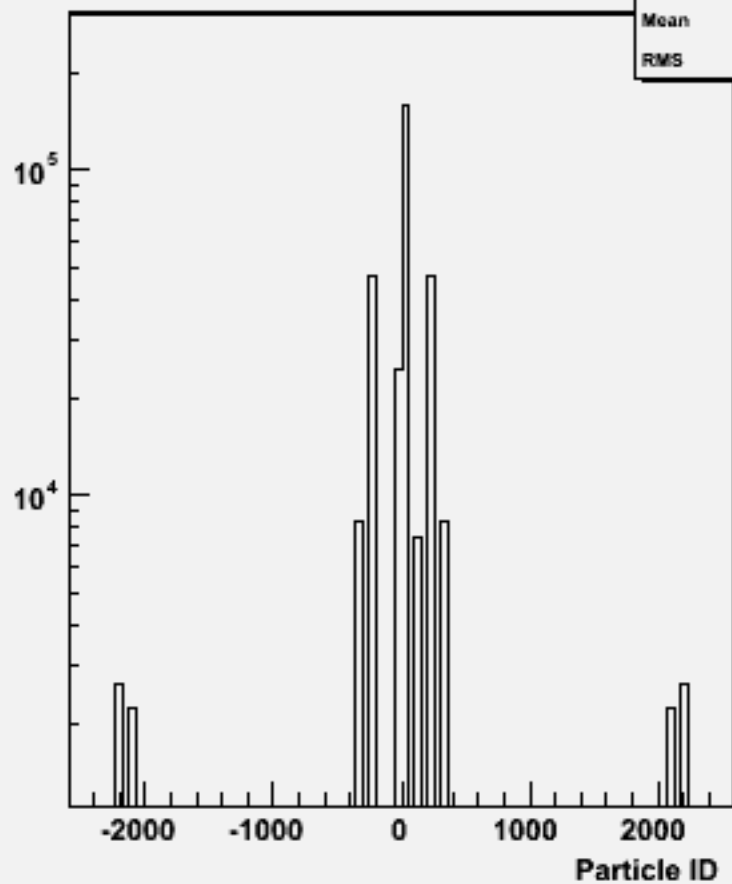
Particle ID : w103844 ae1_e1cce1e1_o
