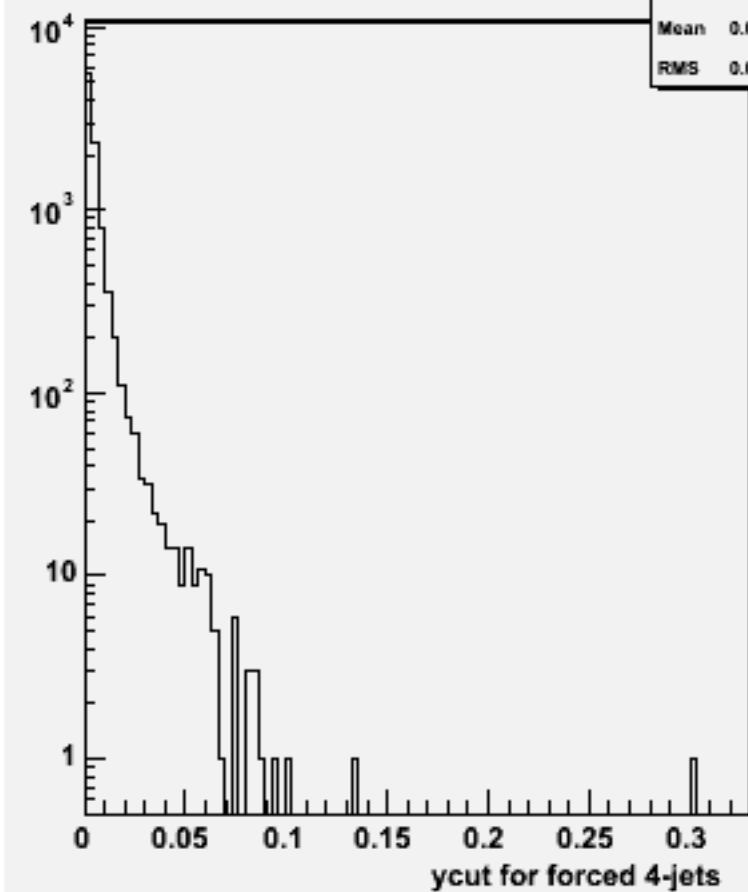
Ycut for 4-jets :w103843 ae1_e1uubb_o
