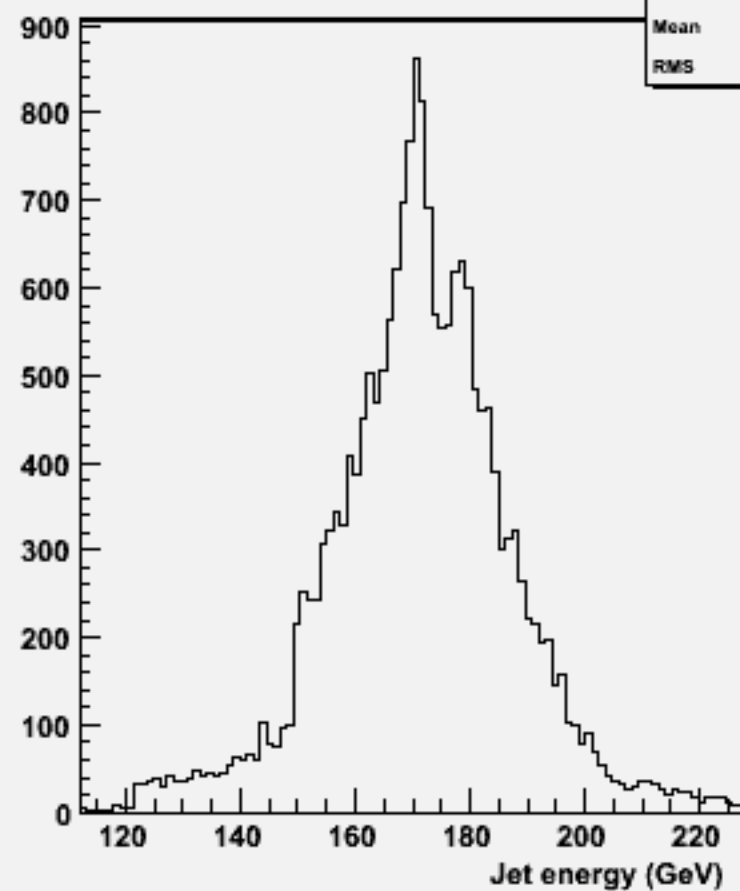
energy for 2-jets :w103843 ae1_e1uubb_o
