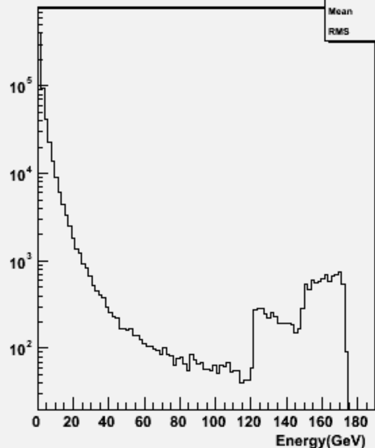
Start point R : w103843 ae1_e1uubb_o
