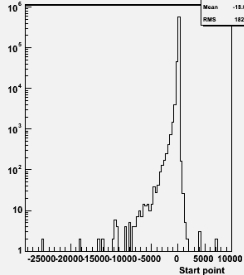
Start point Z : w103843 ae1_e1uubb_o
