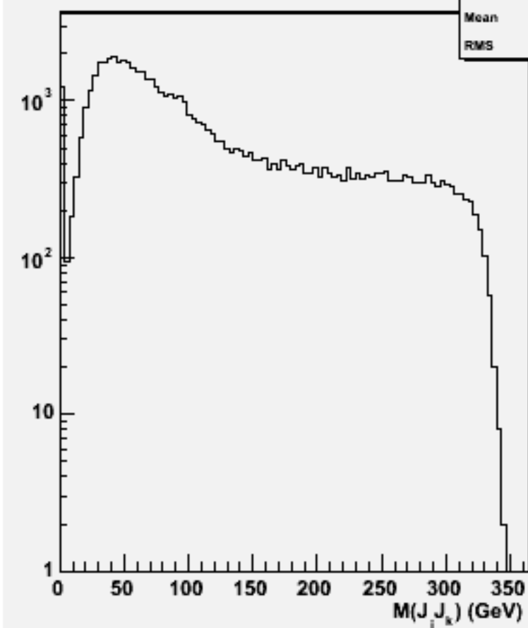
2jets mass(All comb)w103843 ae1_e1uubb_o
