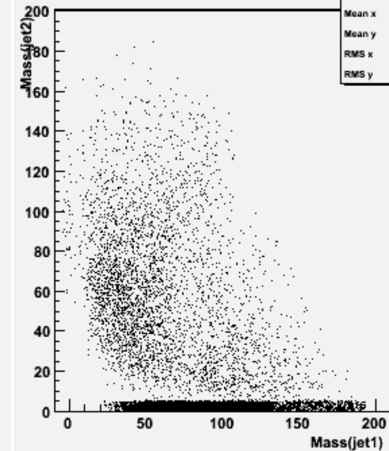
Jet mass for forced 2-jets : w103843 ae1_e1uubb_o
