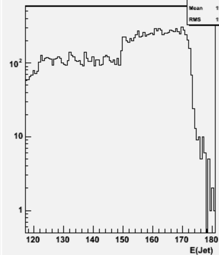
Jet energies(All jets)w103843 ae1_e1uubb_o
