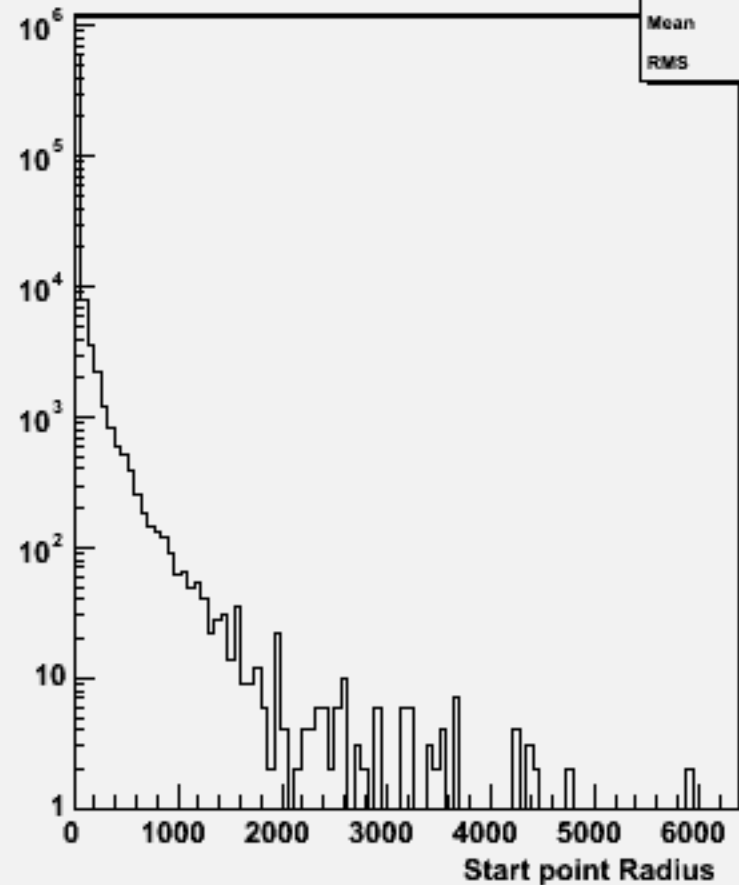
Start point R : w103843 ae1_e1uubb_o
