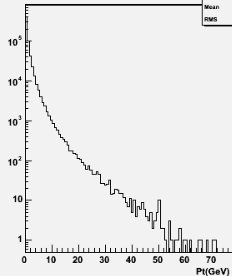
Start point Z : w103843 ae1_e1uubb_o
