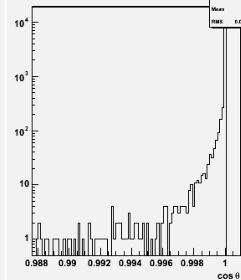
Jet cos \theta (All jets)w103843 ae1_e1uubb_o
