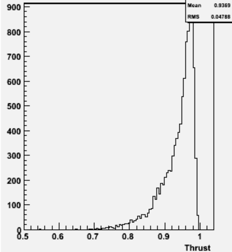
Thrust w103841 ae1_e1uubb_o
