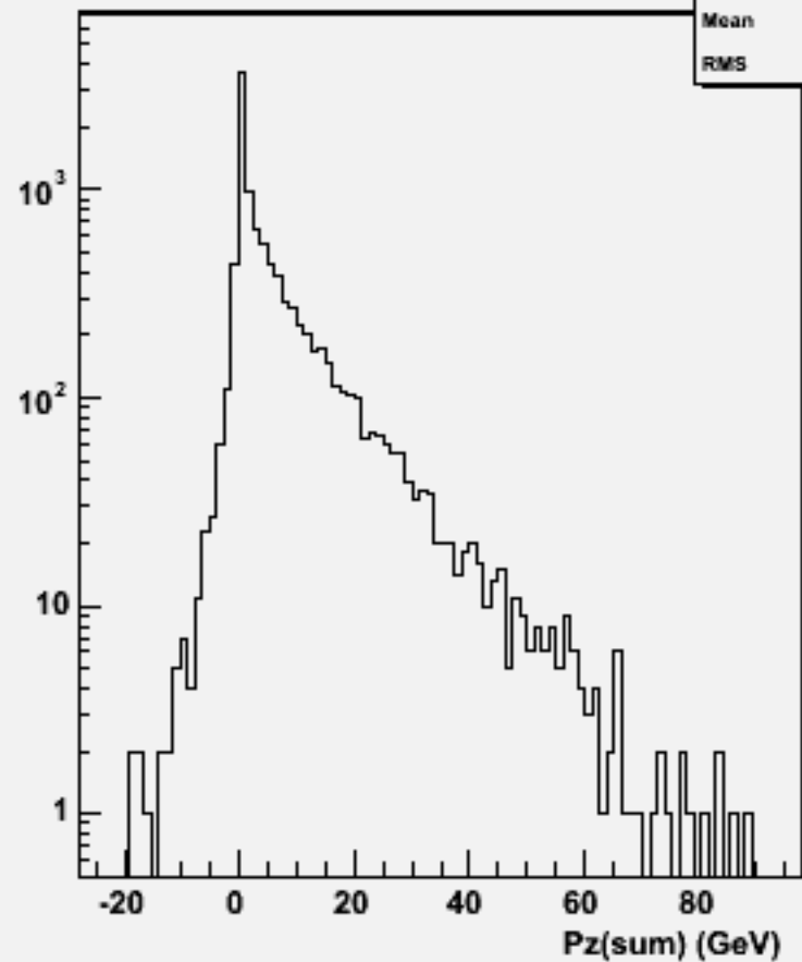
Pz Sum: w103841 ae1_e1uubb_o
