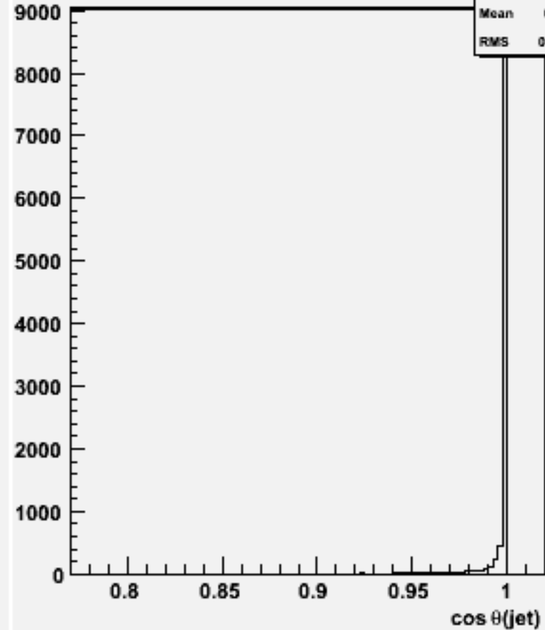
cos \theta for 2-jets :w103841 ae1_e1uubb_o
