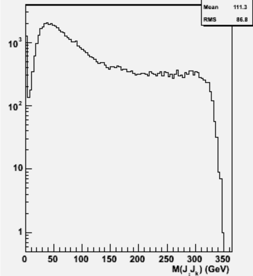
2jets mass(All comb)w103841 ae1_e1uubb_o
