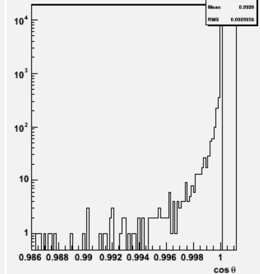
Jet cos \theta (All jets)w103841 ae1_e1uubb_o
