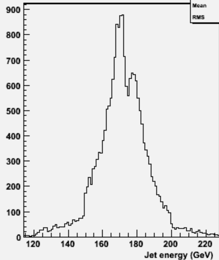
energy for 2-jets :w103841 ae1_e1uubb_o
