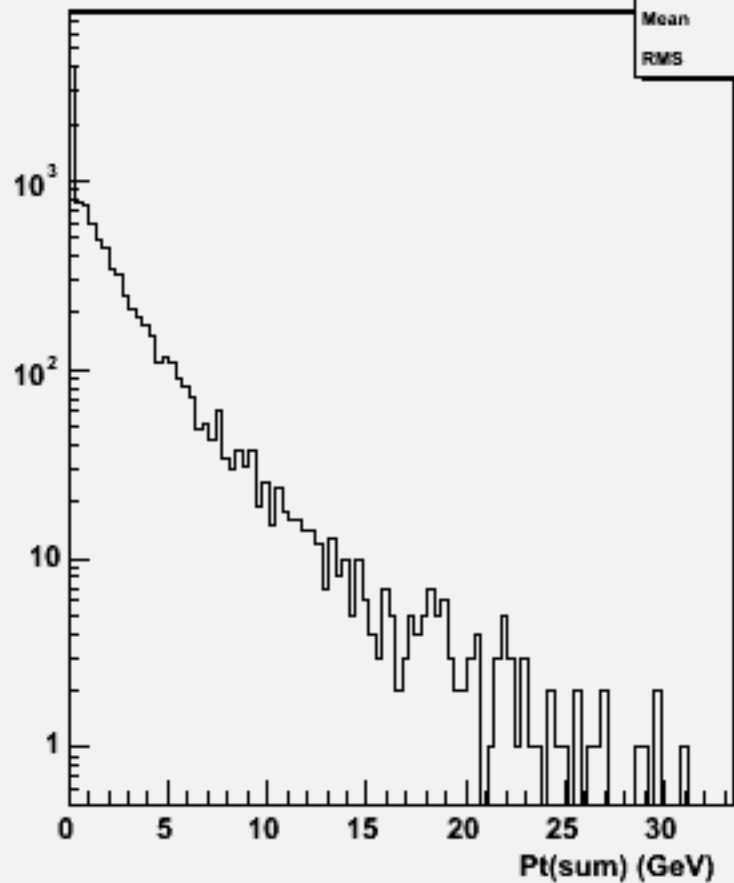
Pt Sum: w103841 ae1_e1uubb_o
