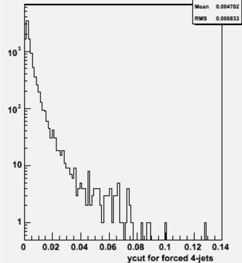
Ycut for 4-jets :w103841 ae1_e1uubb_o
