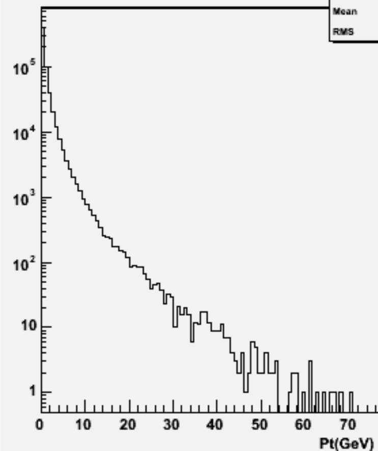
Start point Z : w103841 ae1_e1uubb_o
