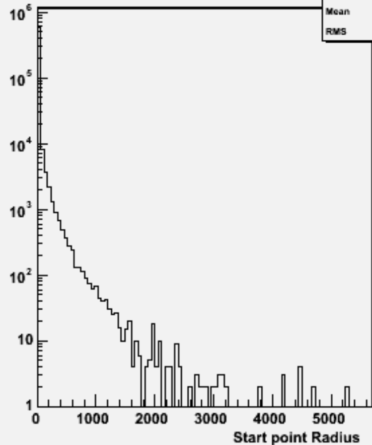
Start point R : w103841 ae1_e1uubb_o
