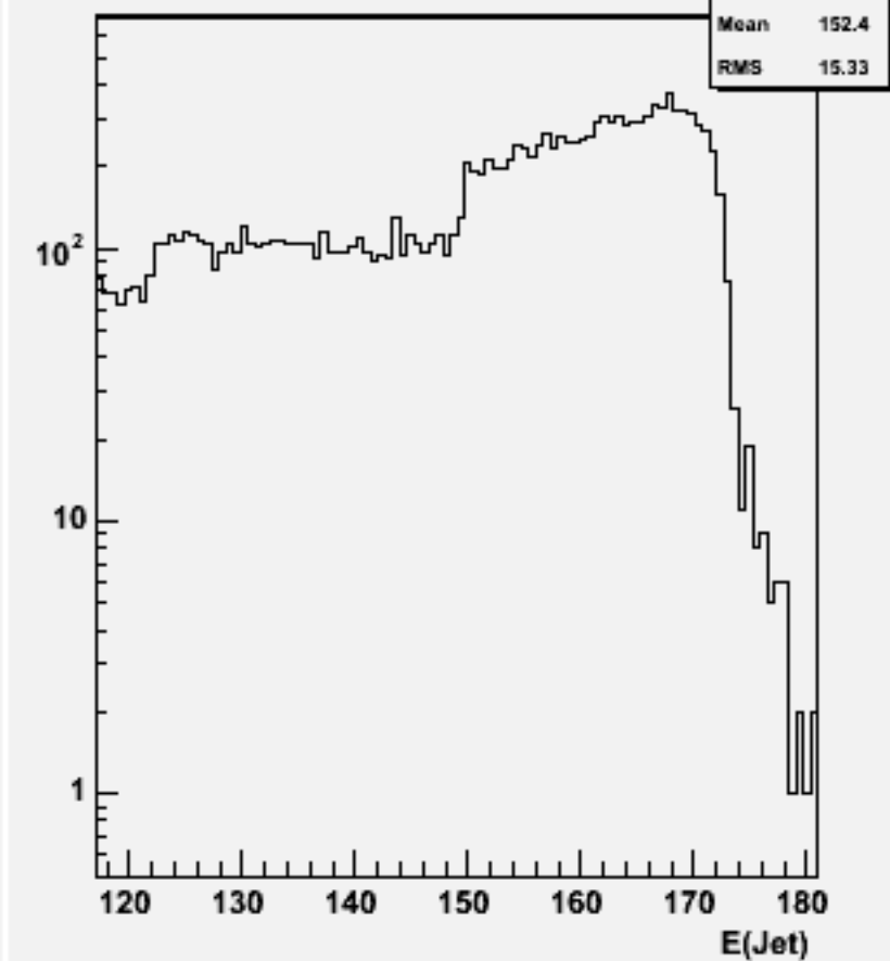
Jet energies(All jets)w103841 ae1_e1uubb_o
