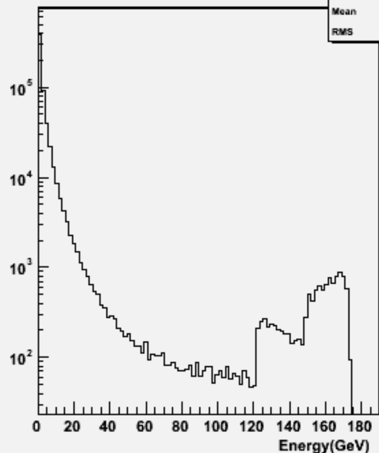
Start point R : w103841 ae1_e1uubb_o
