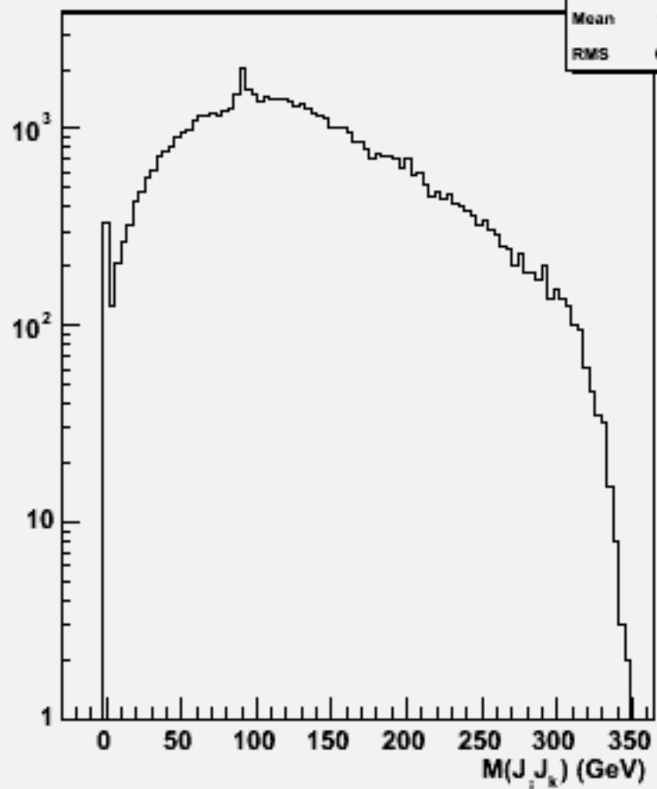
2jets mass(All comb)w103838 ae1_e1uuss_o
