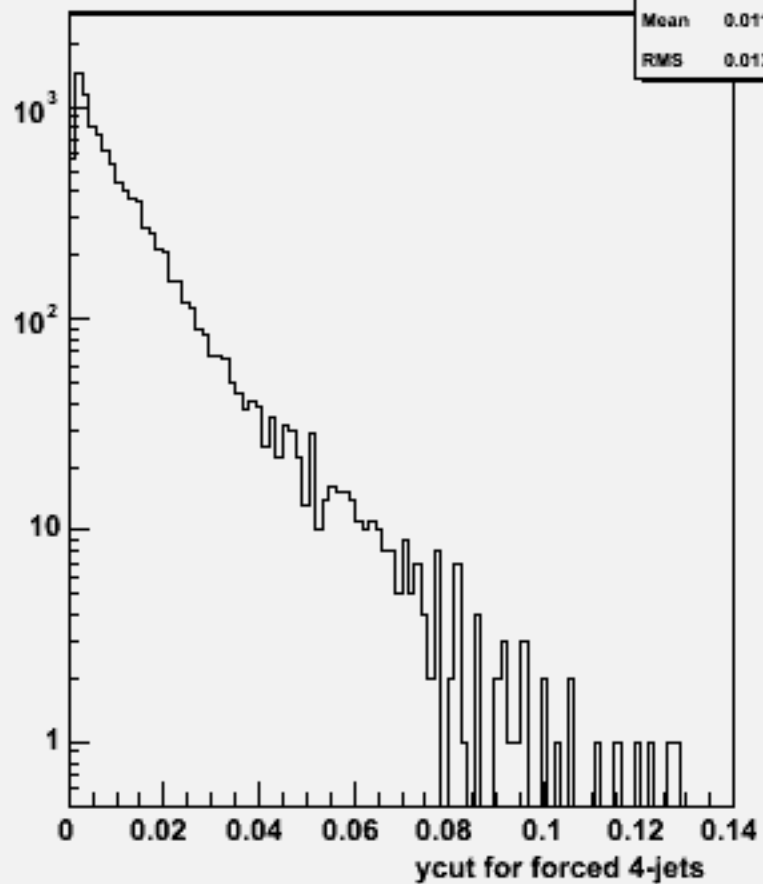
Ycut for 4-jets :w103838 ae1_e1uuss_o
