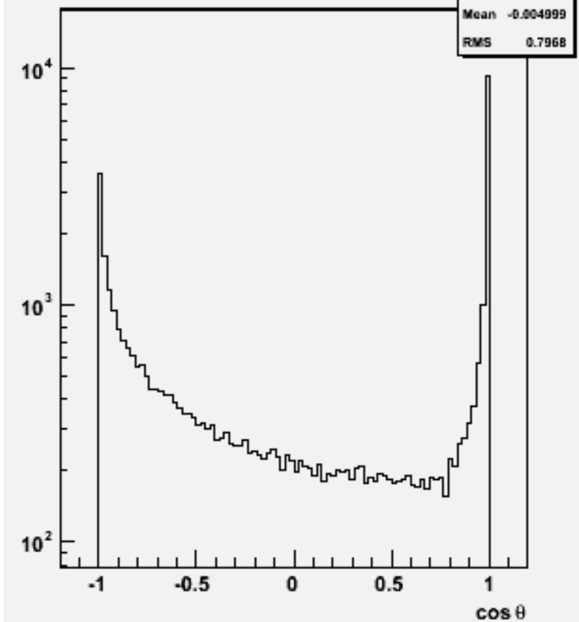
Jet cos \theta (All jets)w103838 ae1_e1uuss_o
