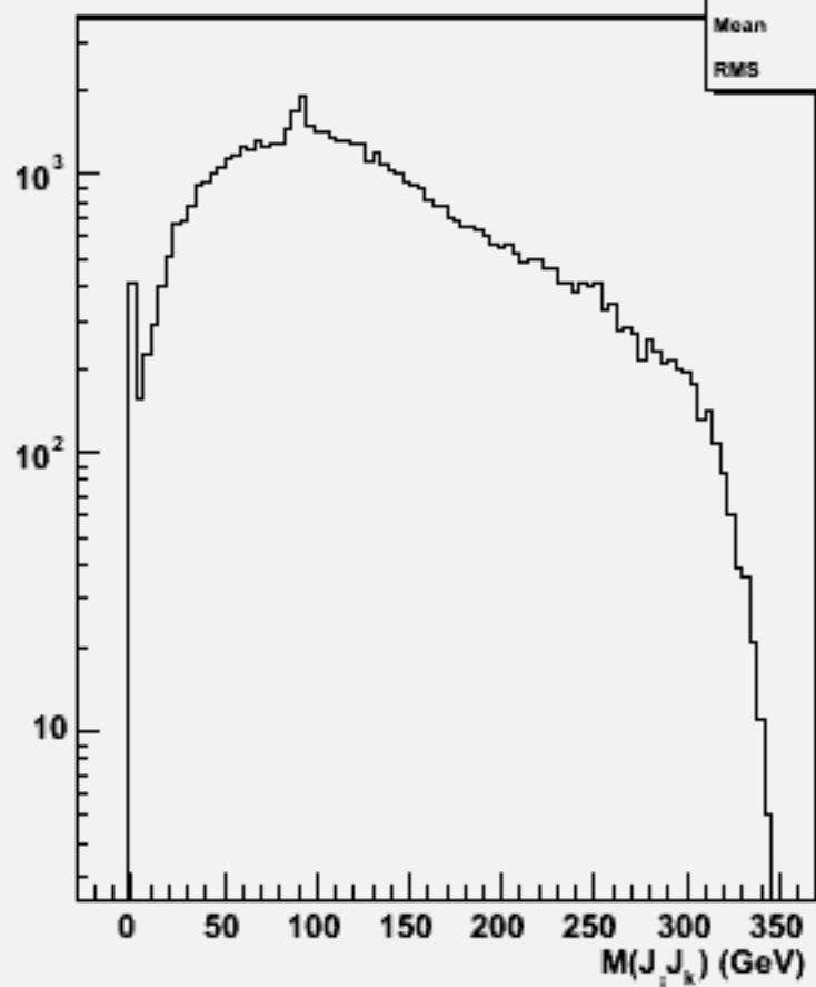
2jets mass(All comb)w103836 ae1_e1uuss_o
