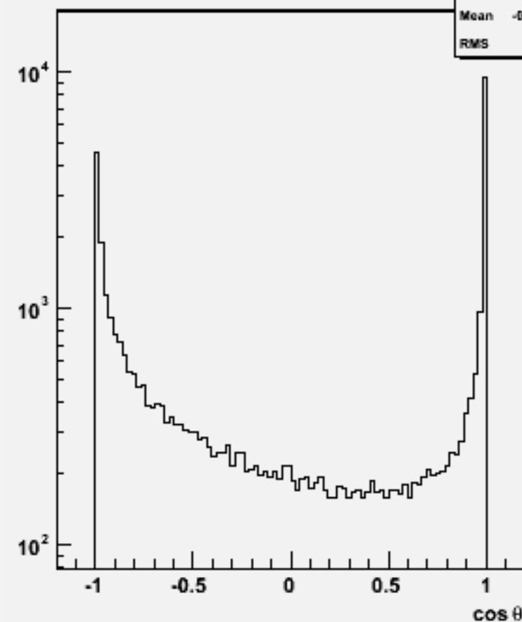
Jet cos \theta (All jets)w103836 ae1_e1uuss_o
