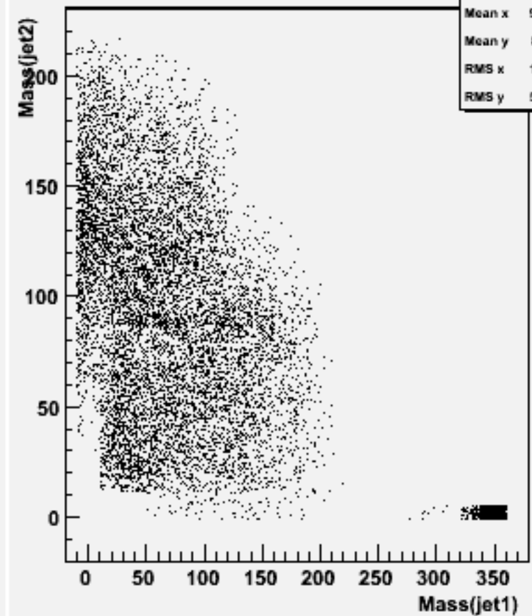
Jet mass for forced 2-jets : w103836 ae1_e1uuss_o
