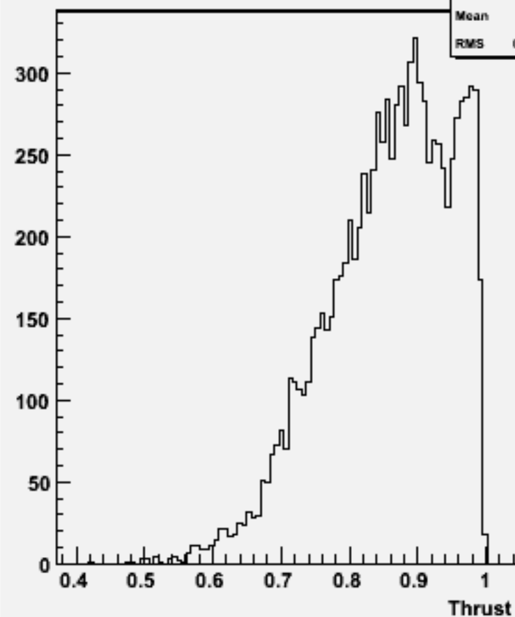
Thrust w103836 ae1_e1uuss_o
