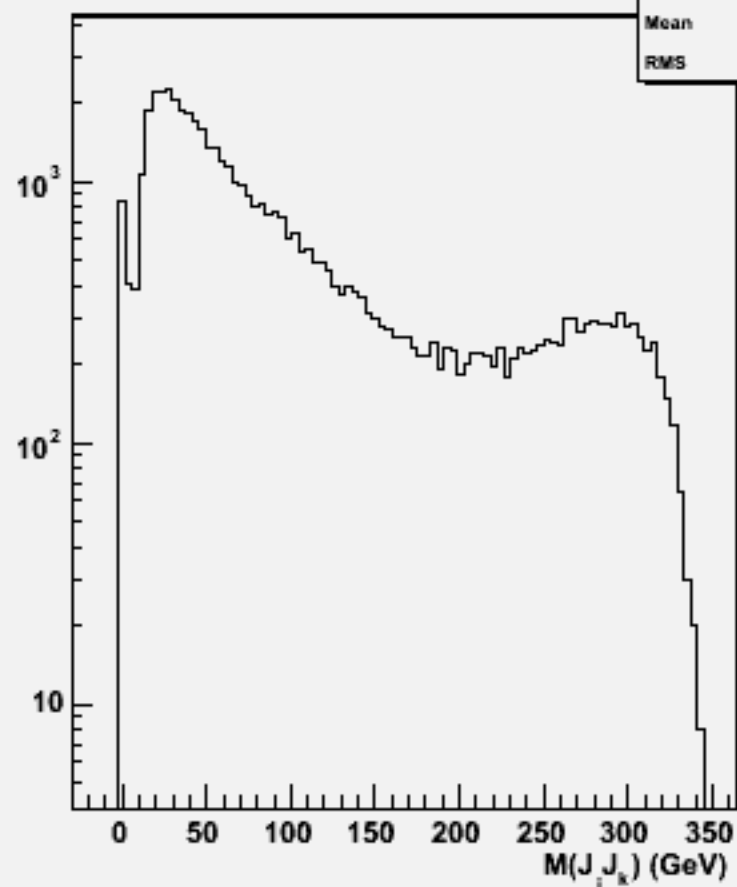
2jets mass(All comb)w103834 ae1_e1uue3e3_o
