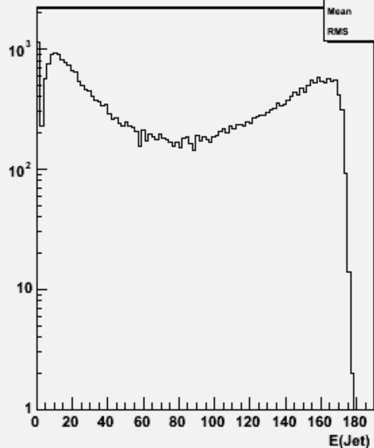
Jet energies(All jets)w103834 ae1_e1uue3e3_o
