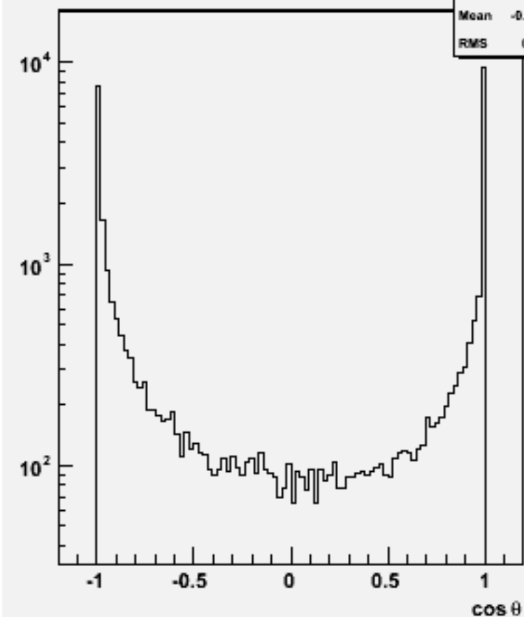
Jet cos \theta (All jets)w103834 ae1_e1uue3e3_o
