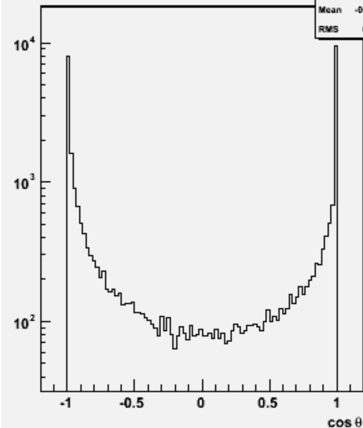
Jet cos \theta (All jets)w103832 ae1_e1uue3e3_o
