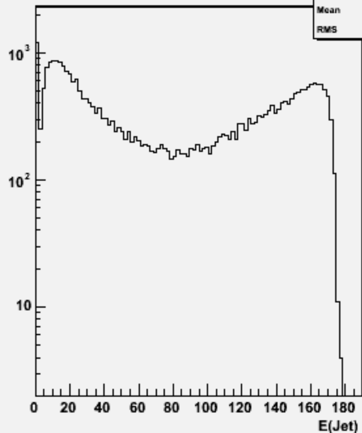
Jet energies(All jets)w103832 ae1_e1uue3e3_o
