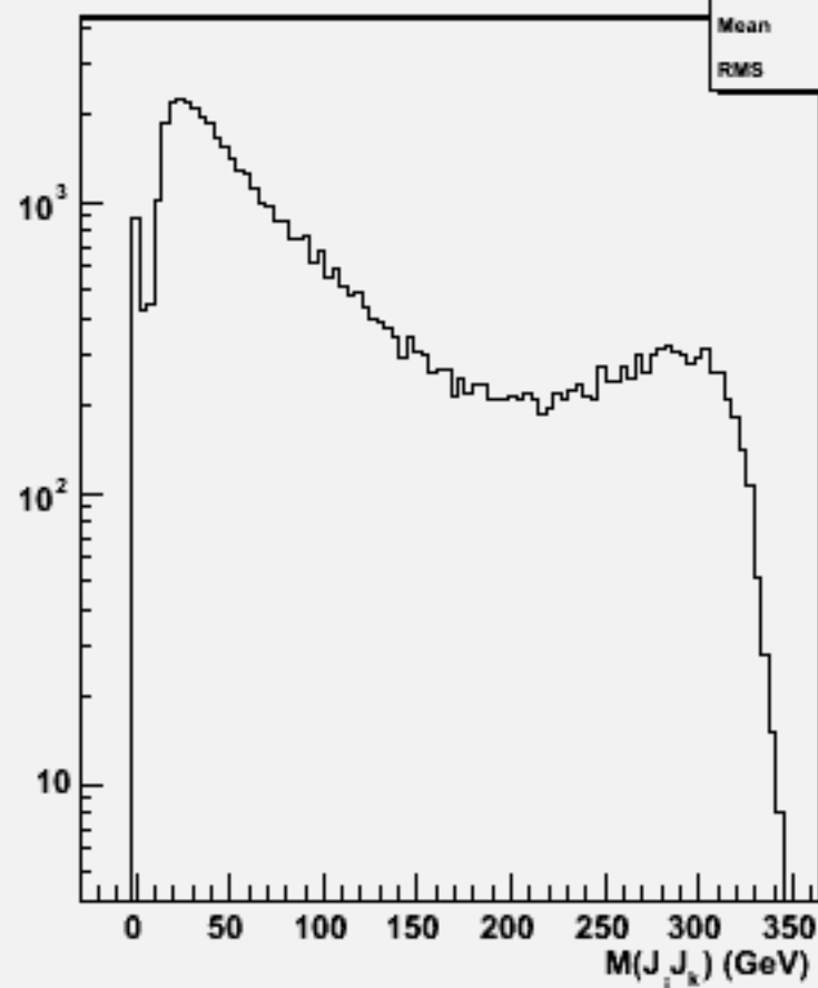
2jets mass(All comb)w103832 ae1_e1uue3e3_o
