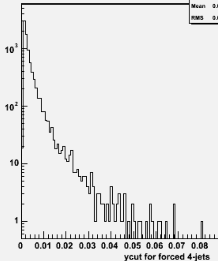
Ycut for 4-jets :w103832 ae1_e1uue3e3_o
