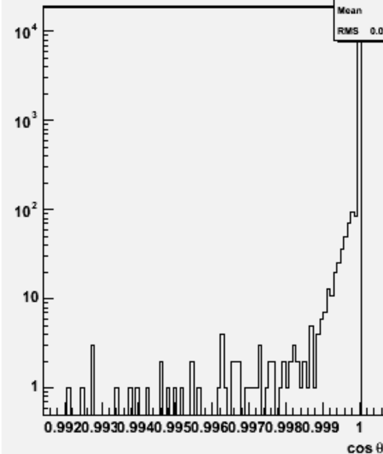
Jet cos \theta (All jets)w103831 ae1_e1uue2e2_o
