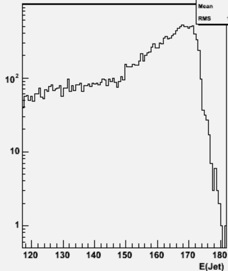
Jet energies(All jets)w103831 ae1_e1uue2e2_o
