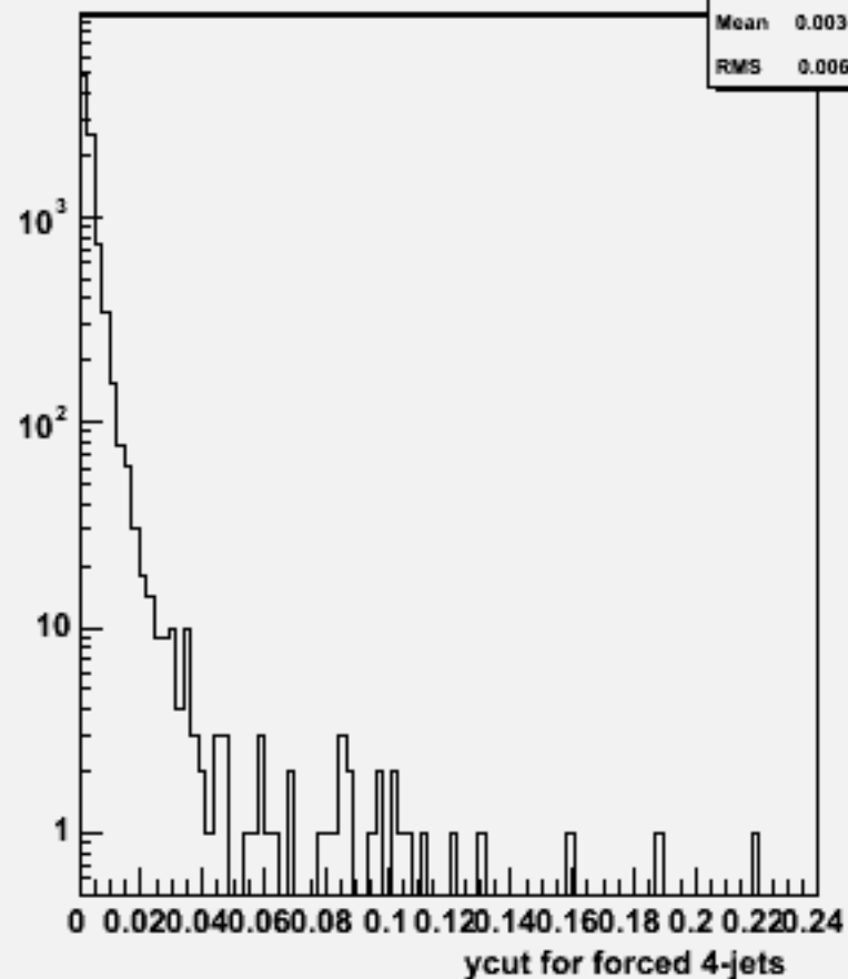
Ycut for 4-jets :w103831 ae1_e1uue2e2_o
