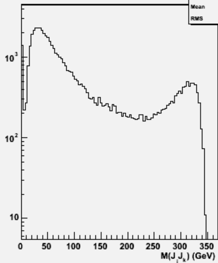
2jets mass(All comb)w103831 ae1_e1uue2e2_o
