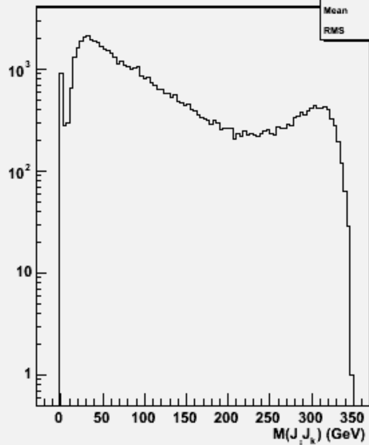
2jets mass(All comb)w103830 ae1_e1uue2e2_o
