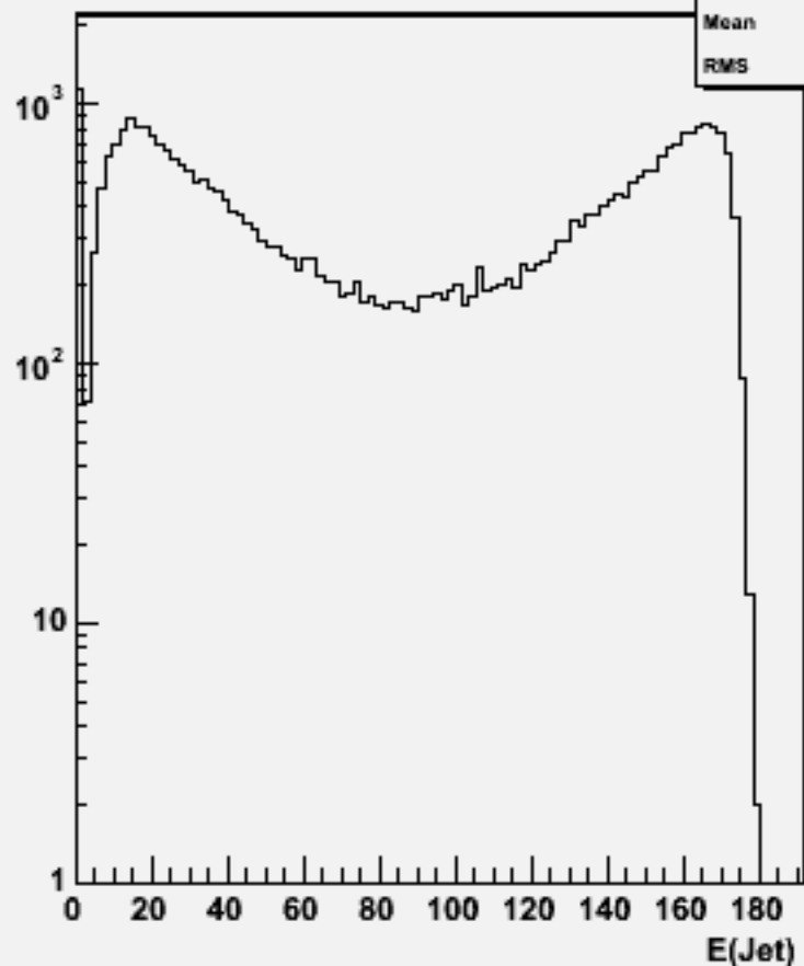
Jet energies(All jets)w103830 ae1_e1uue2e2_o
