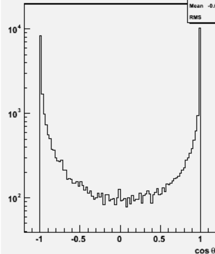
Jet cos \theta (All jets)w103830 ae1_e1uue2e2_o
