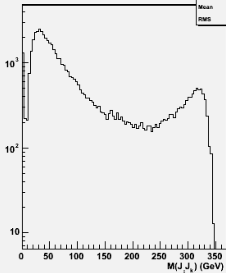
2jets mass(All comb)w103829 ae1_e1uue2e2_o
