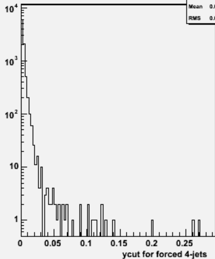
Ycut for 4-jets :w103829 ae1_e1uue2e2_o
