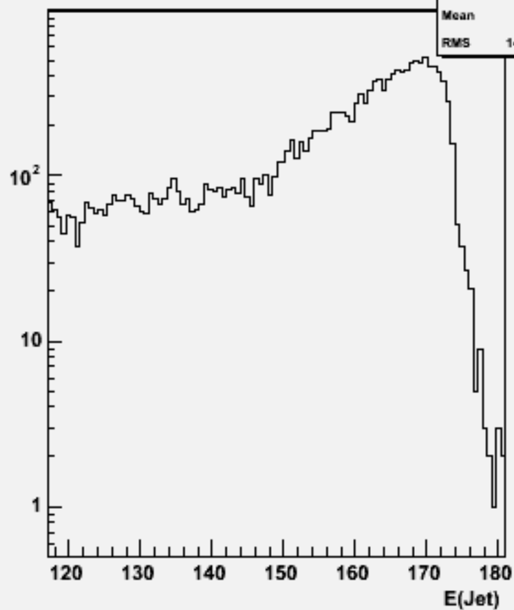
Jet energies(All jets)w103829 ae1_e1uue2e2_o
