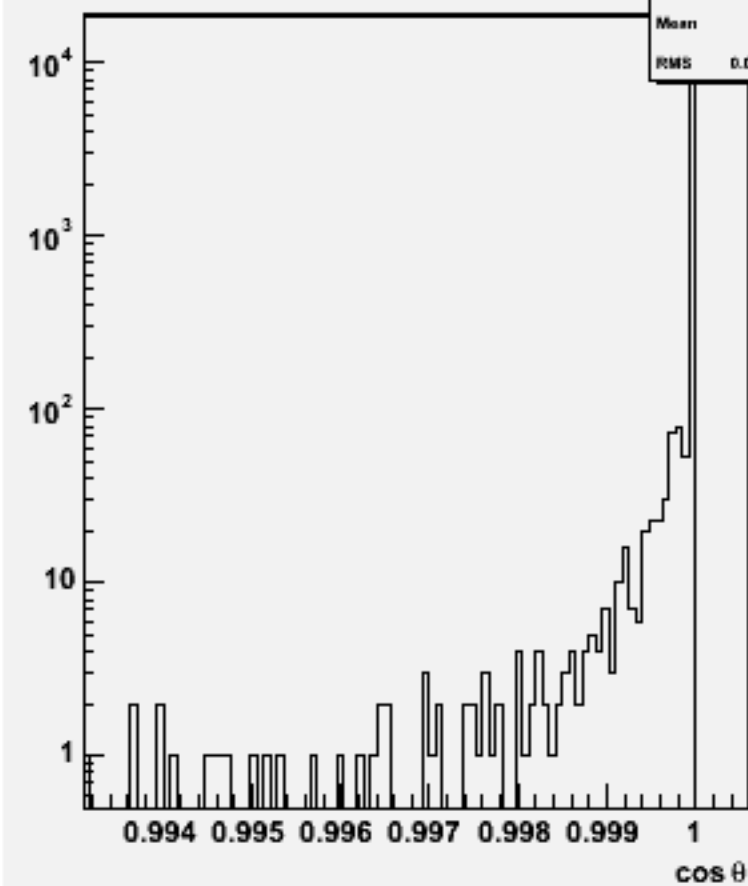
Jet cos \theta (All jets)w103829 ae1_e1uue2e2_o
