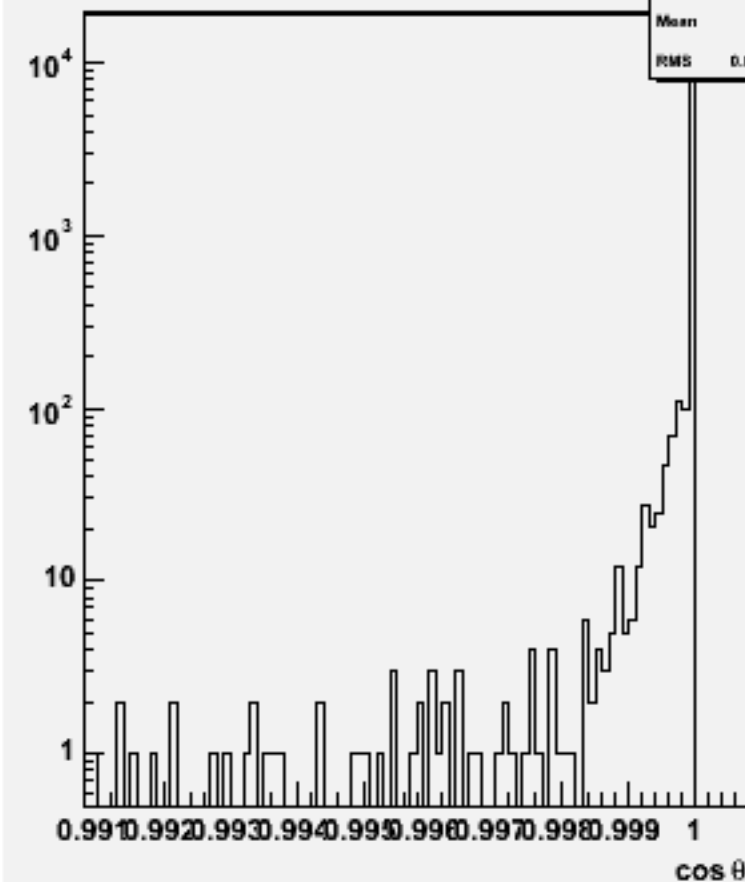
Jet cos \theta (All jets)w103827 ae1_e1uue1e1_o
