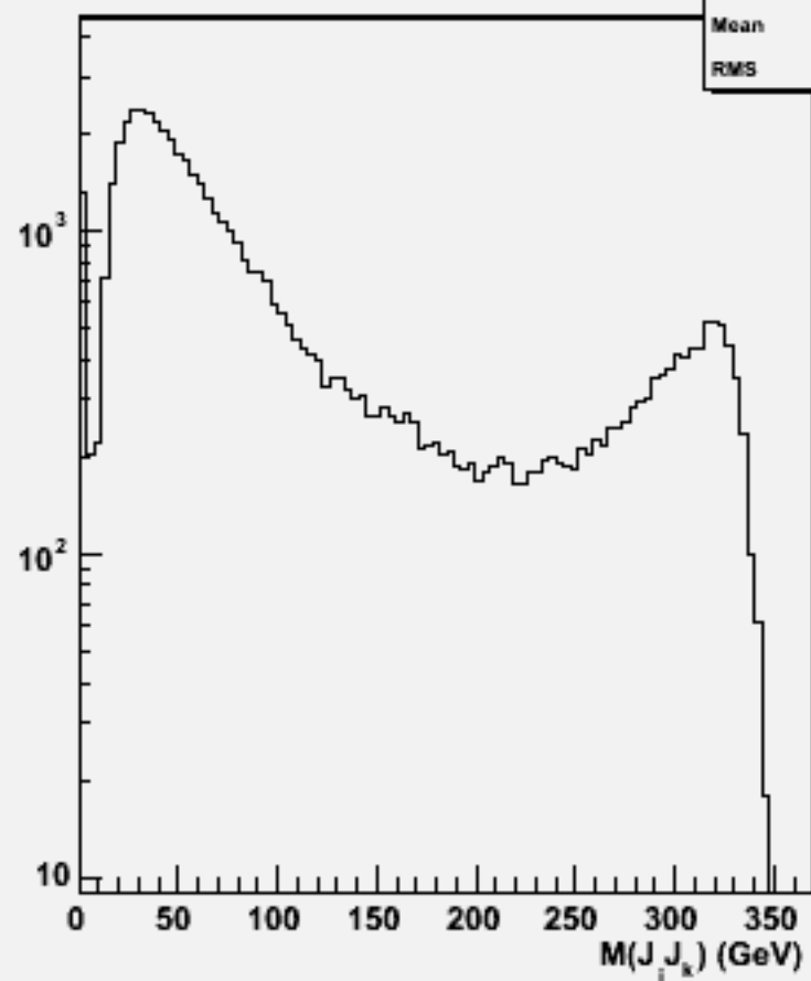
2jets mass(All comb)w103827 ae1_e1uue1e1_o
