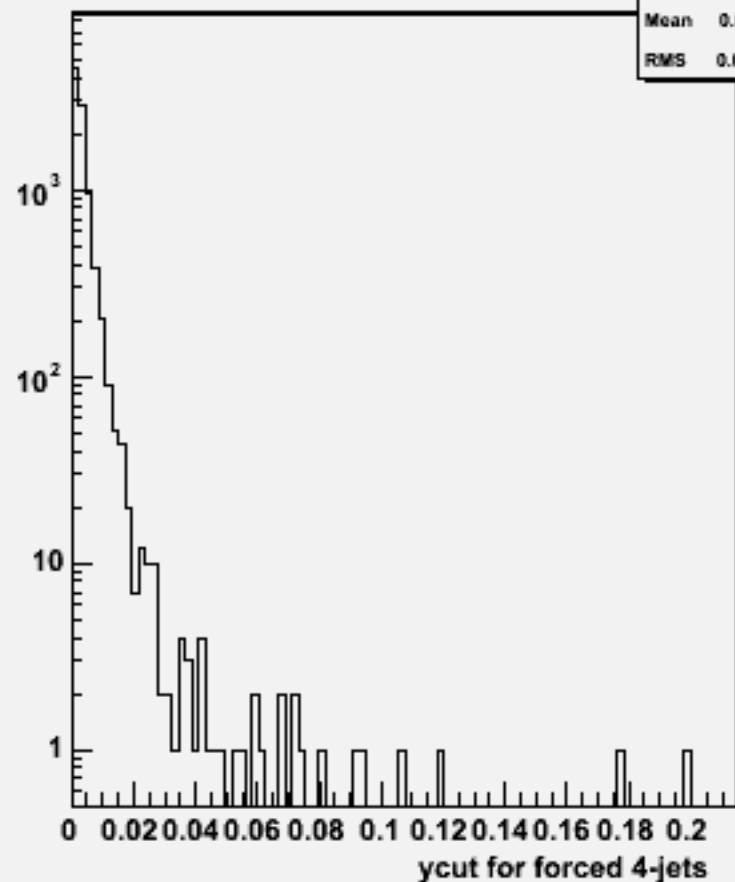
Ycut for 4-jets :w103827 ae1_e1uue1e1_o
