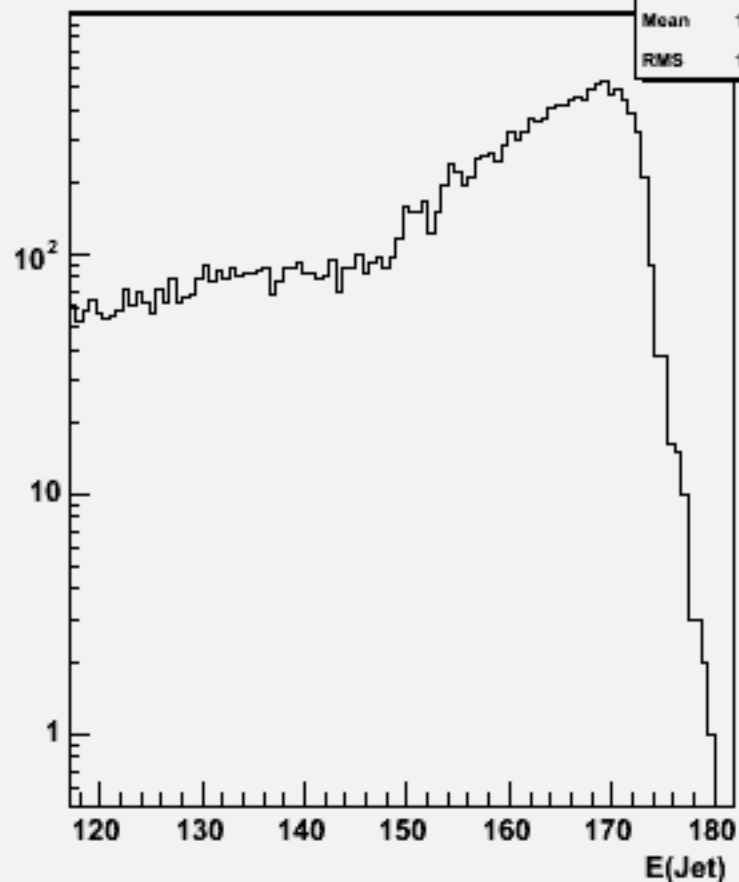
Jet energies(All jets)w103827 ae1_e1uue1e1_o
