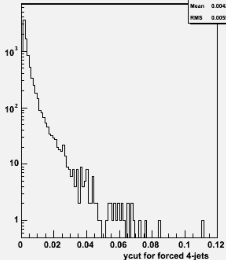
Ycut for 4-jets :w103826 ae1_e1uue1e1_o
