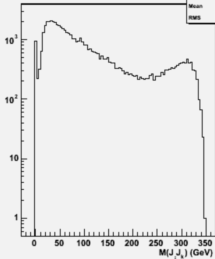
2jets mass(All comb)w103826 ae1_e1uue1e1_o
