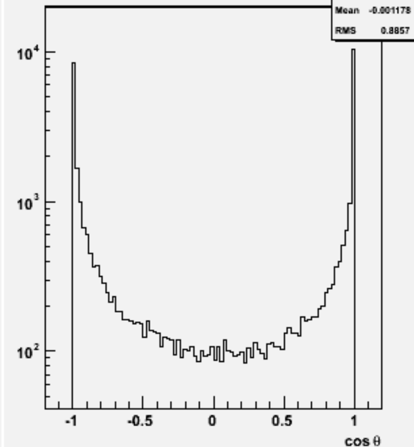
Jet cos \theta (All jets)w103826 ae1_e1uue1e1_o
