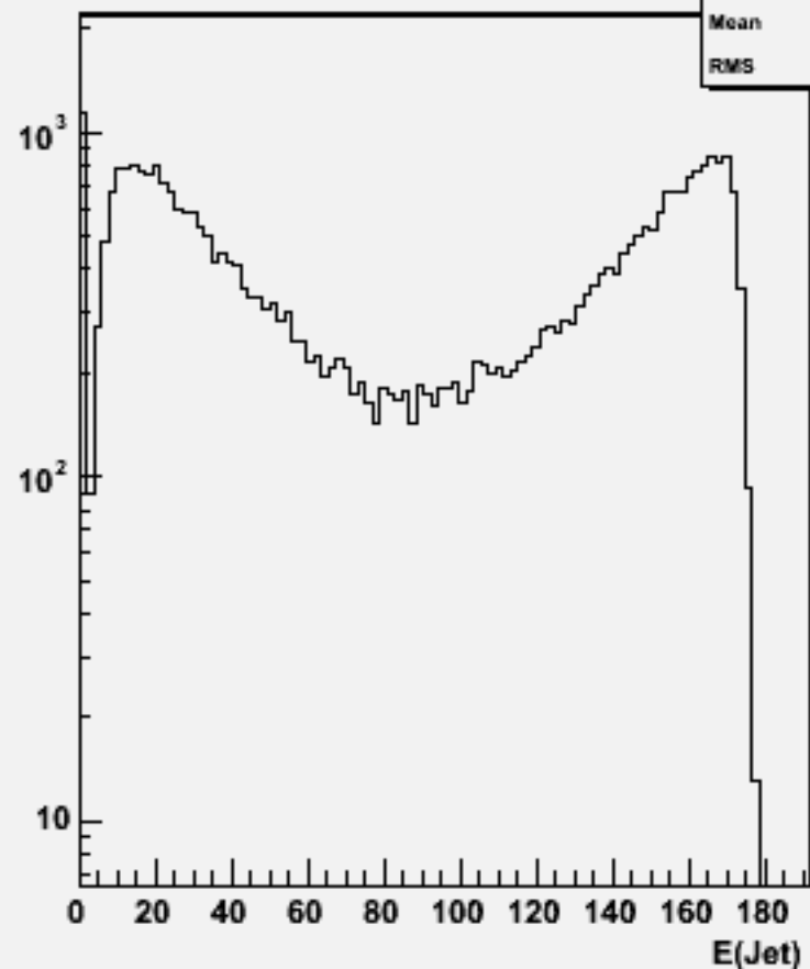
Jet energies(All jets)w103826 ae1_e1uue1e1_o
