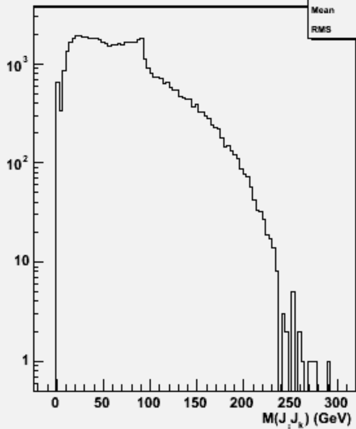
2jets mass(All comb)w103820 ae1_e1n3n3bb_o
