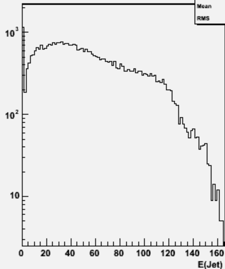
Jet energies(All jets)w103820 ae1_e1n3n3bb_o
