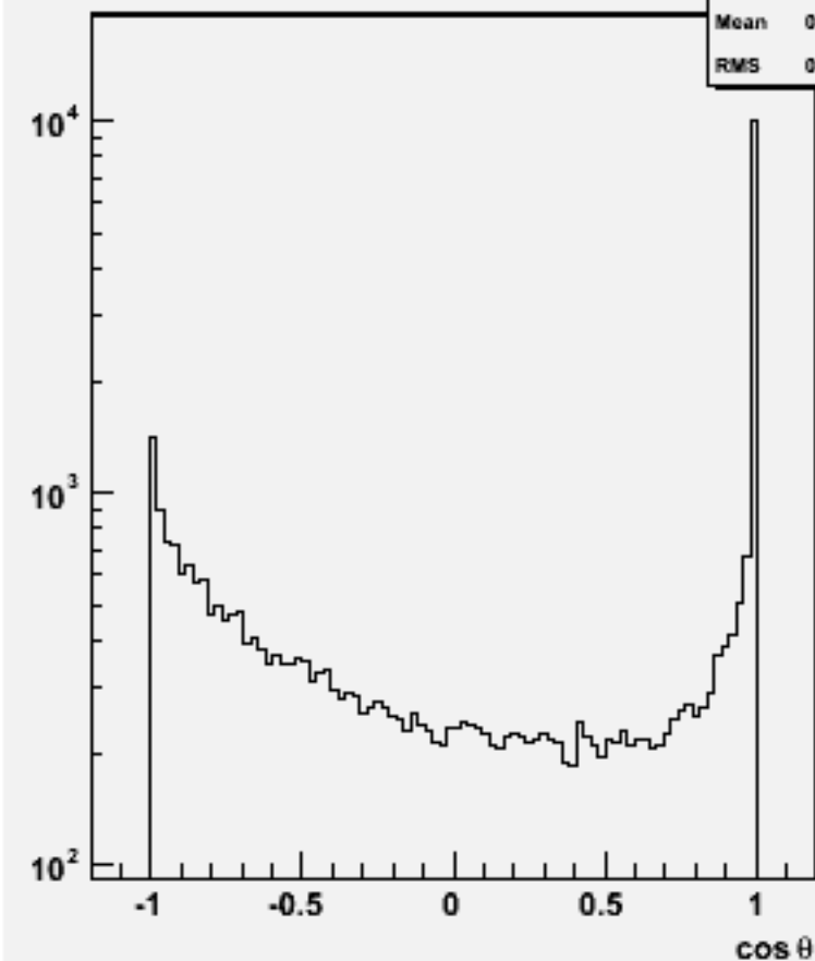
Jet cos \theta (All jets)w103820 ae1_e1n3n3bb_o
