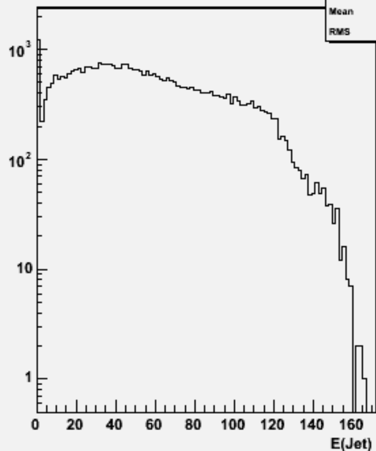
Jet energies(All jets)w103818 ae1_e1n3n3ss_o
