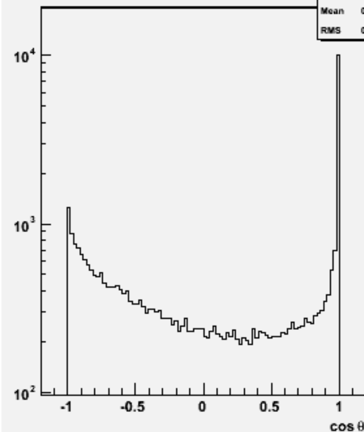
Jet cos \theta (All jets)w103818 ae1_e1n3n3ss_o
