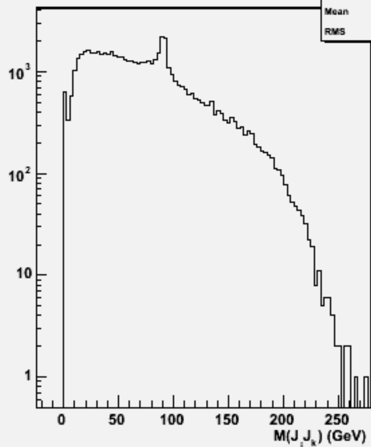
2jets mass(All comb)w103818 ae1_e1n3n3ss_o
