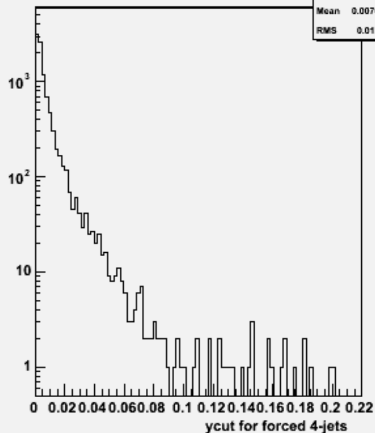
Ycut for 4-jets :w103818 ae1_e1n3n3ss_o
