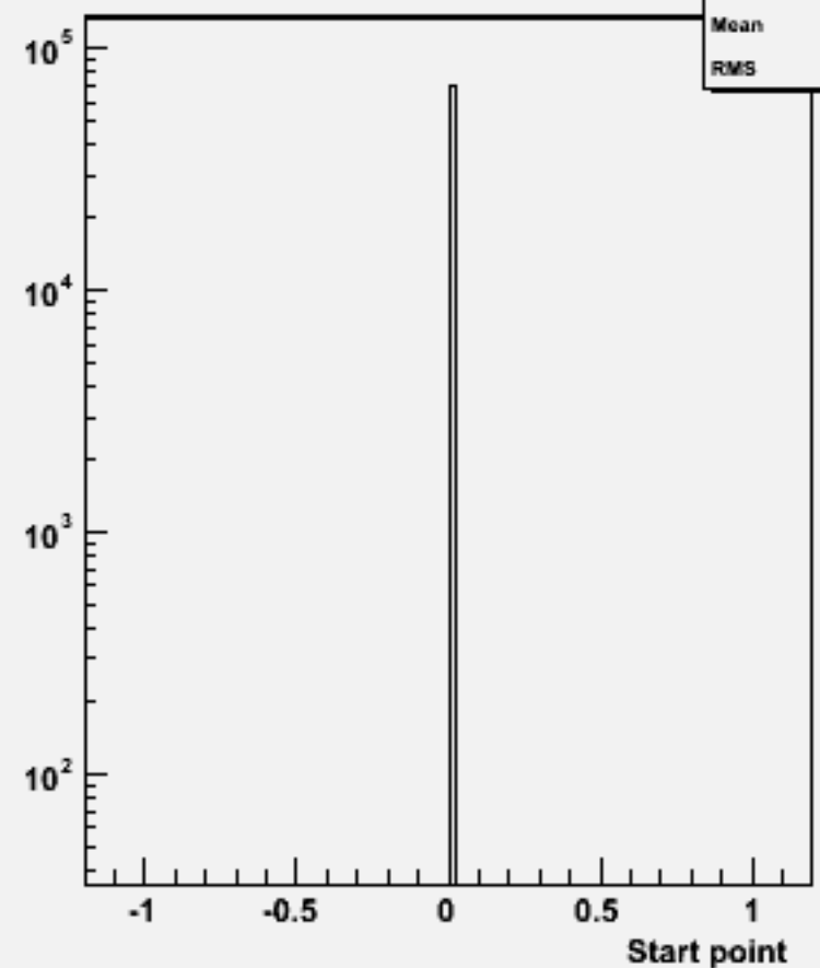
Start point Z : w103808 ae1_e1n3n3e2e2_o
