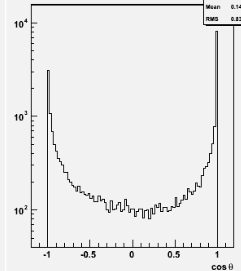
Jet cos \theta (All jets)w103808 ae1_e1n3n3e2e2_o
