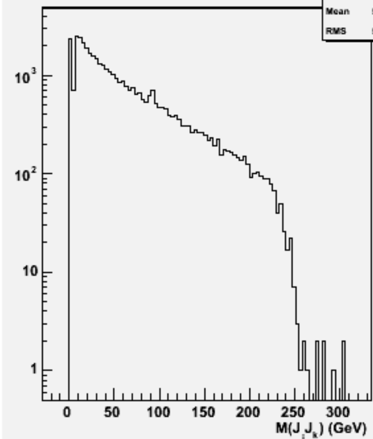
2jets mass(All comb)w103808 ae1_e1n3n3e2e2_o
