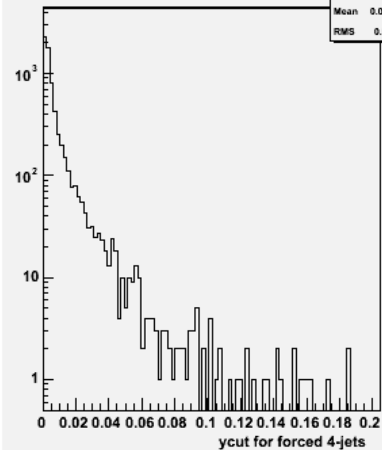
Ycut for 4-jets :w103808 ae1_e1n3n3e2e2_o
