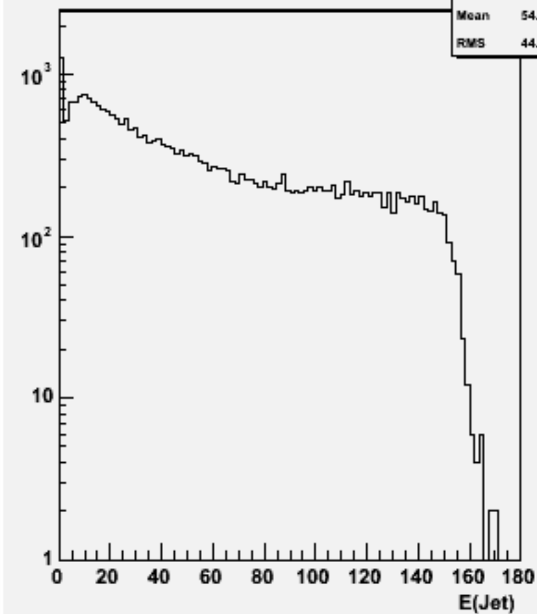
Jet energies(All jets)w103808 ae1_e1n3n3e2e2_o
