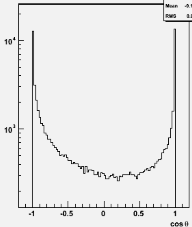
Particle cos \theta : w103808 ae1_e1n3n3e2e2_o
