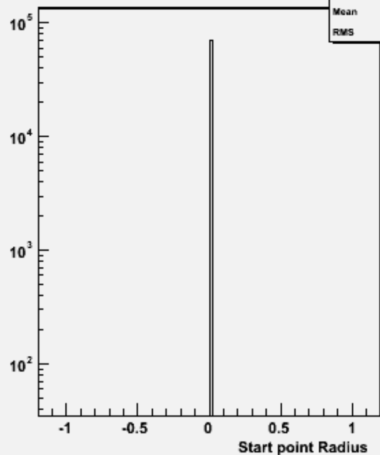
Start point R : w103808 ae1_e1n3n3e2e2_o
