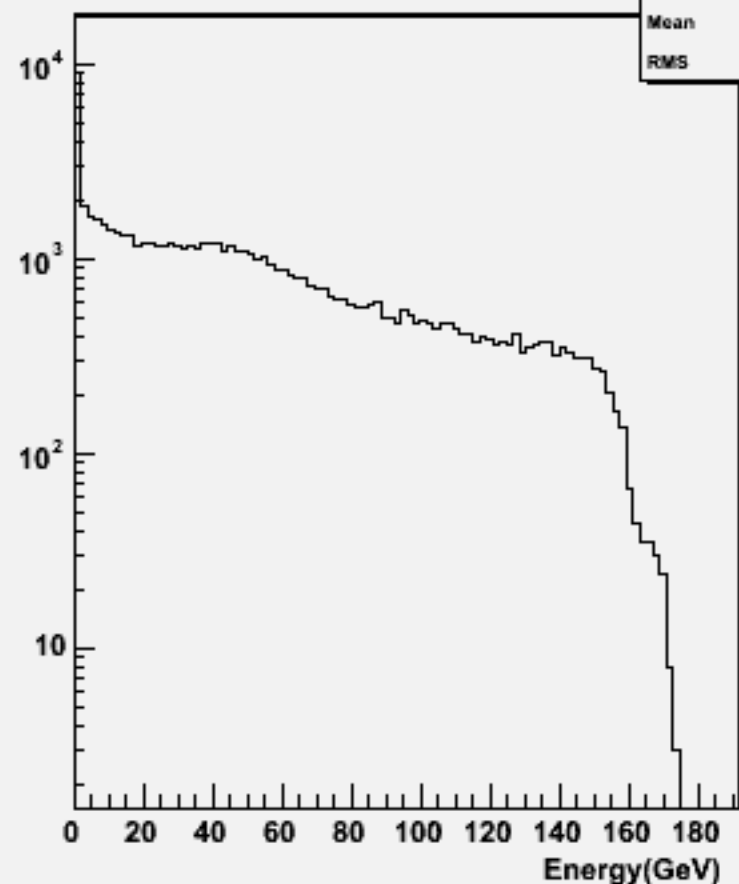
Particle Energy : w103808 ae1_e1n3n3e2e2_o
